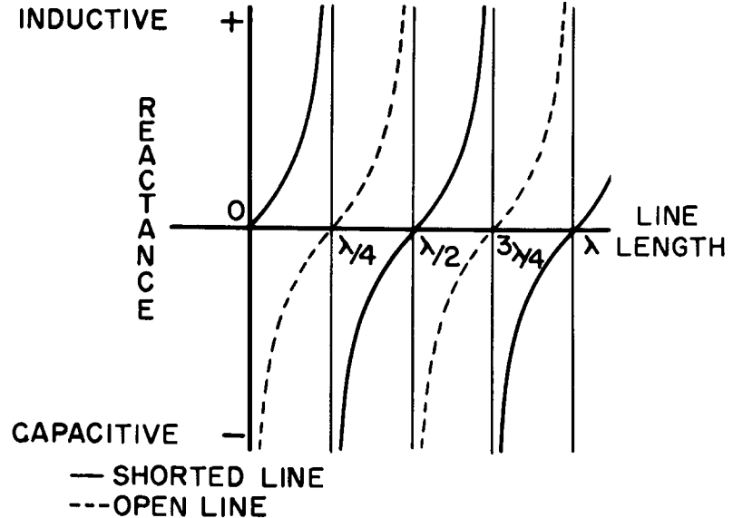
INPUT IMPEDANCE/LINE LENGTH IN WAVELENGTHS FOR A LOSSLESS LINE
