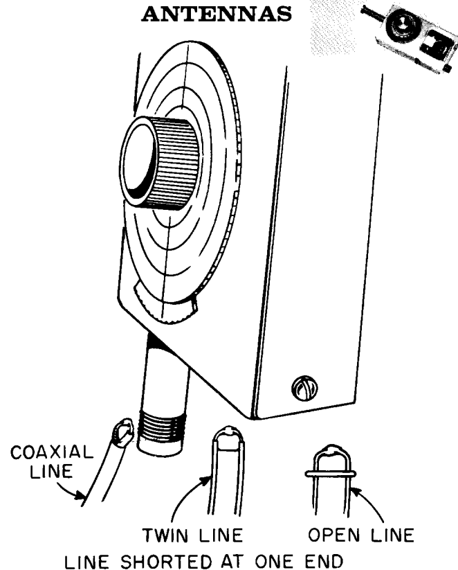
FIGURE 11. COUPLING TO TRANSMISSION LINES.
