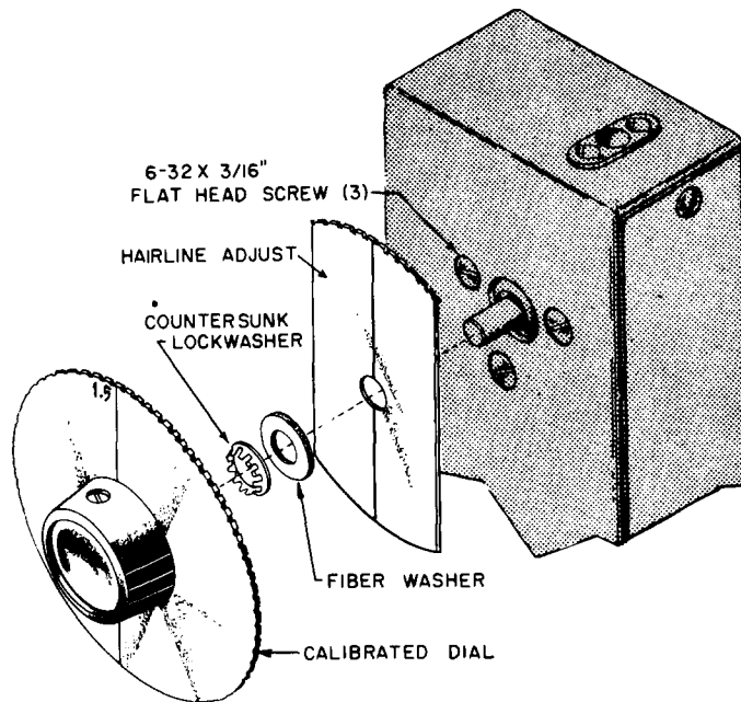
FIGURE 8. MOUNTING THE DIAL
