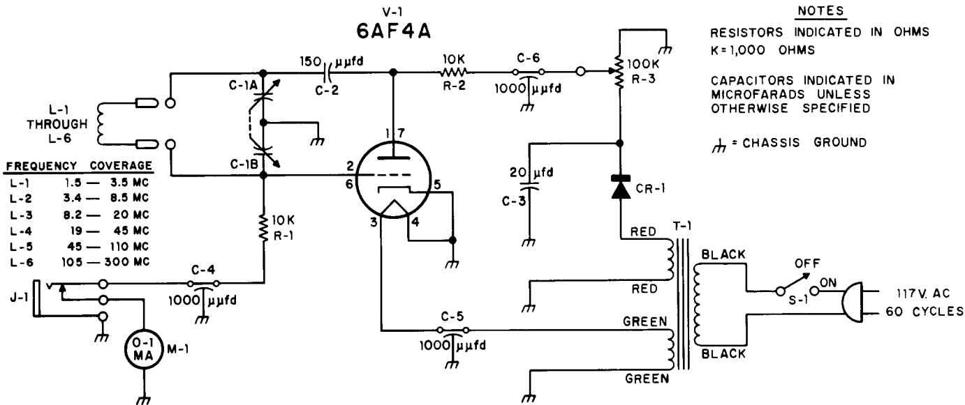
SCHEMATIC DIAGRAM OF GRID DIP METER
