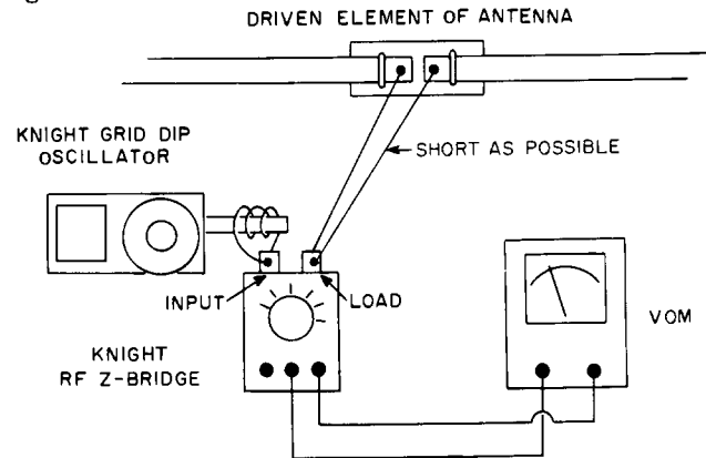
FIGURE 12. COUPLING TO AN ANTENNA THROUGH AN SWR BRIDGE.
