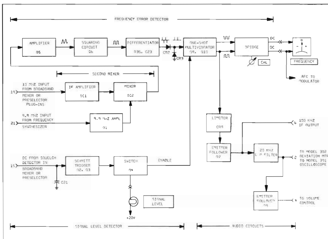
Figure 4-3. Second IF and Discriminator Circuits, Simplified Block Diagram
