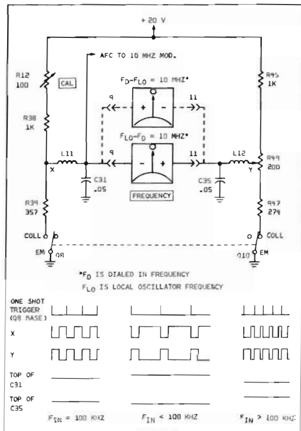
Figure 4-4. Frequency Meter Bridge Circuit
