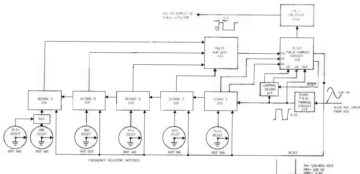
Figure 4-2. Divid-by-N Counter, Simplified Block Diagram
