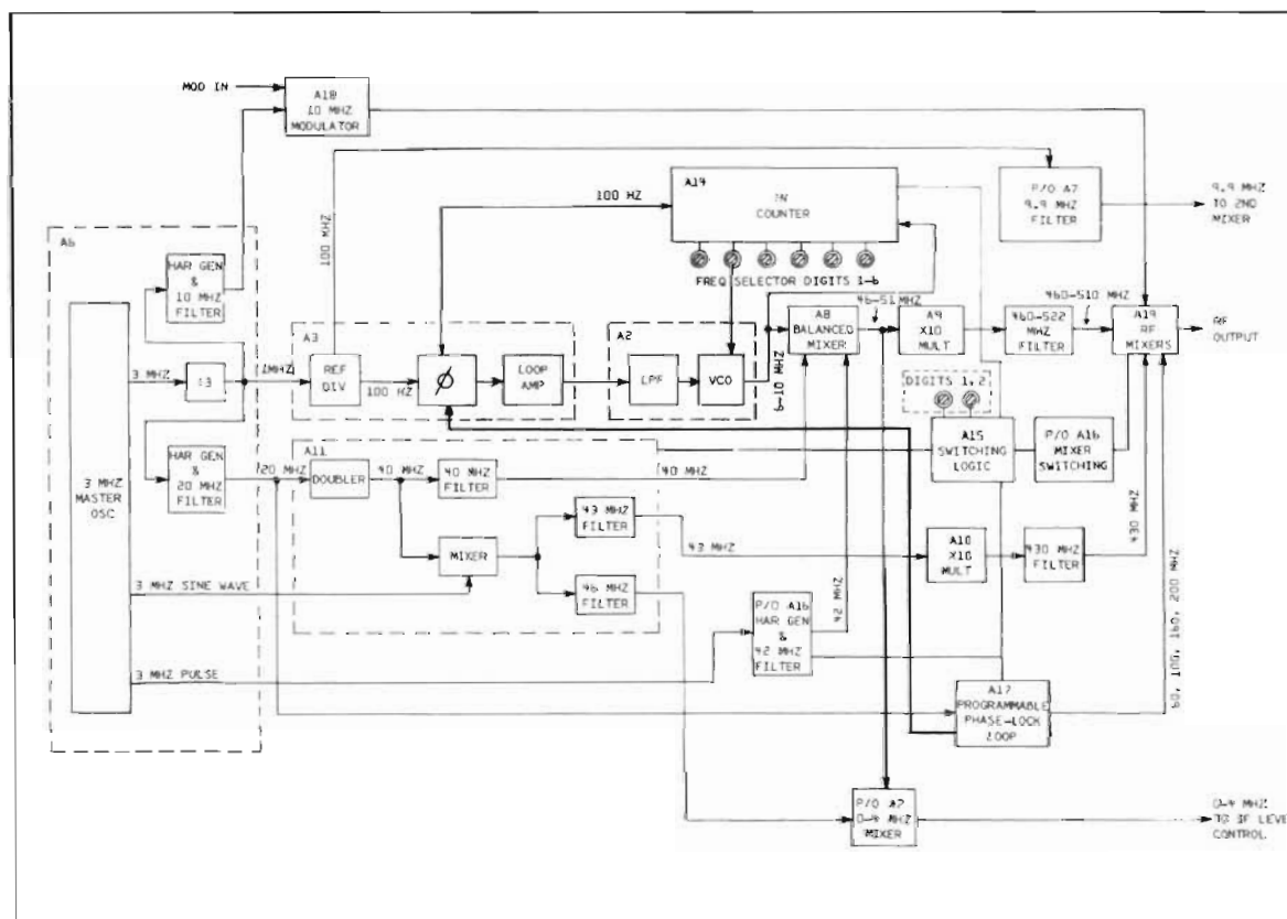
Figure 4-1. Frequency Synthesizer, Simplified Block Diagram
