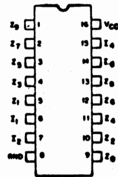
BASE CONNECTIONS
