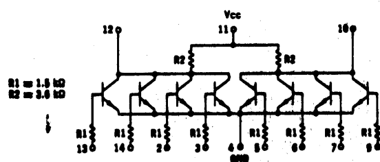
MC723P - J-K FLIP-FLOP
