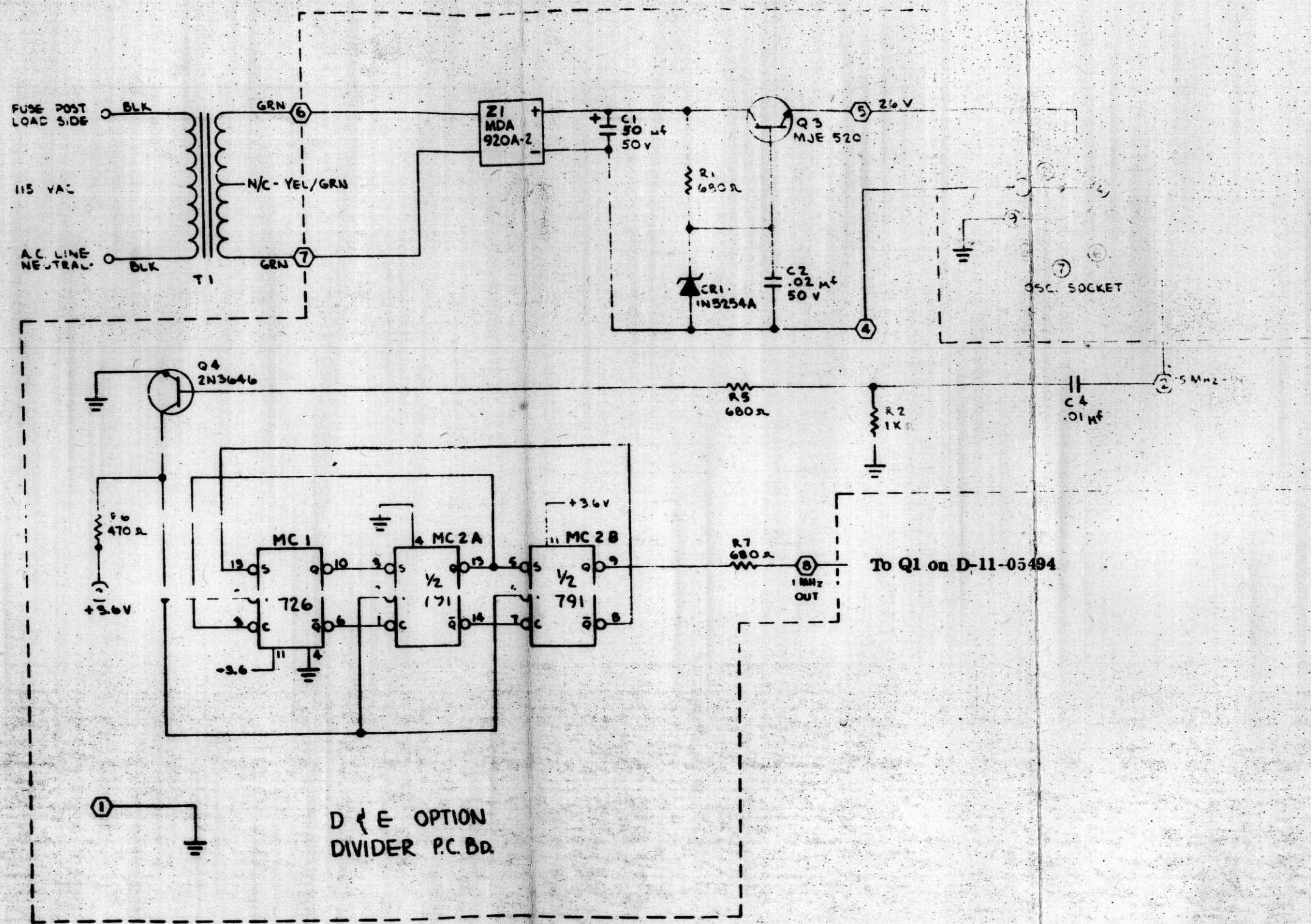
MODEL 1650 D and E OPTION OSCILLATOR SCHEMATIC C-11-06115
