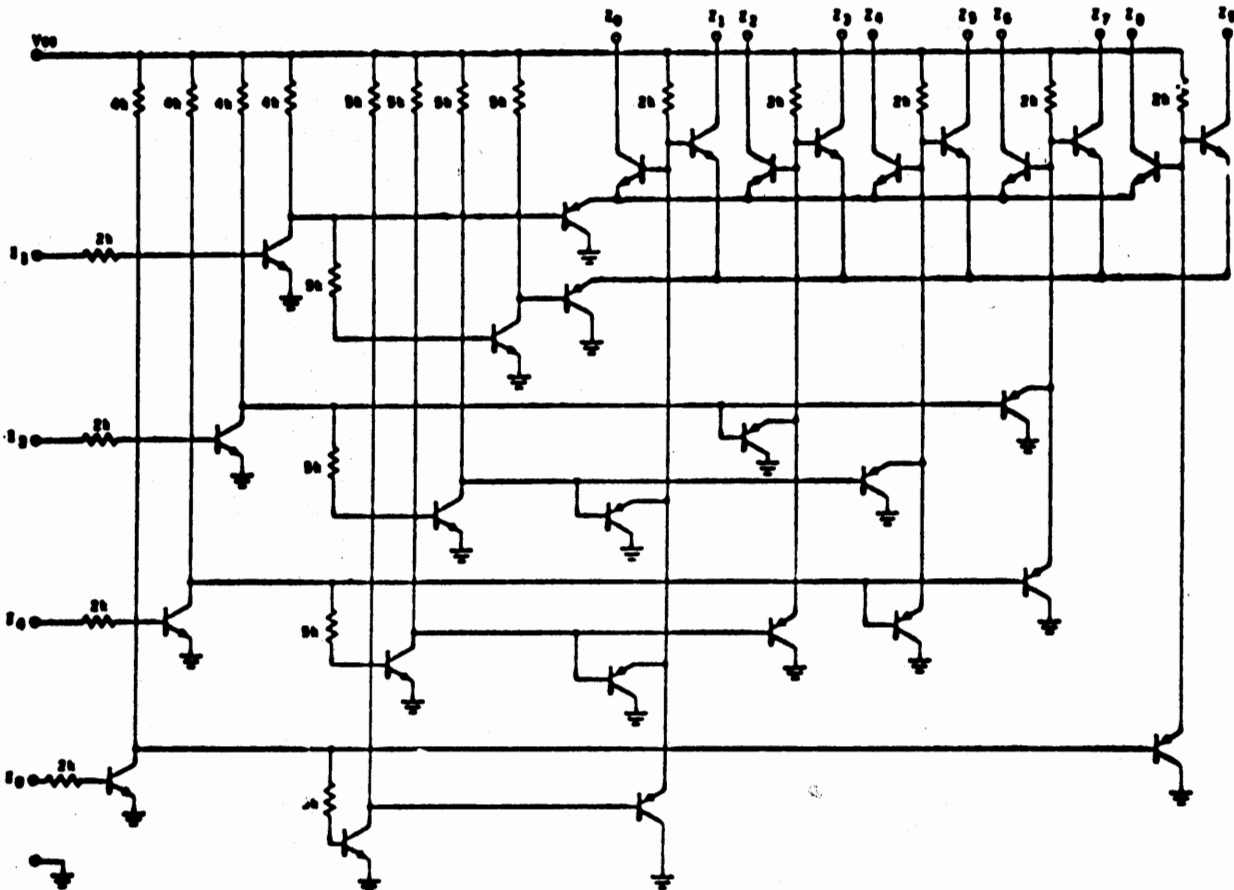
Schematic Diagram Decimal Decoder \mu L 9960
