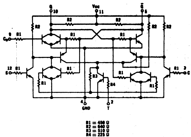
MC723P - J-K FLIP-FLOP
