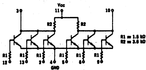
MC718P - DUAL 3-INPUT GATE
