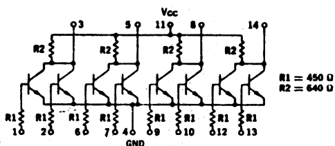
MC724P - QUAD 2-INPUT GATE
