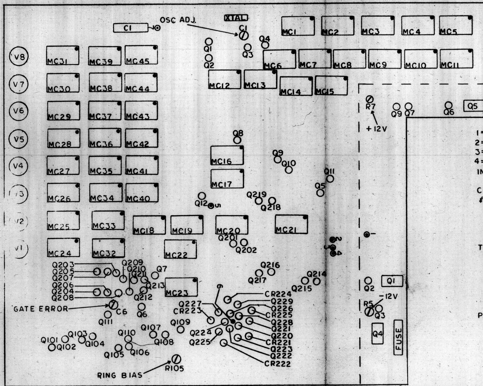
MODEL 1615/1650 PCB COMPONENT LAYOUT
