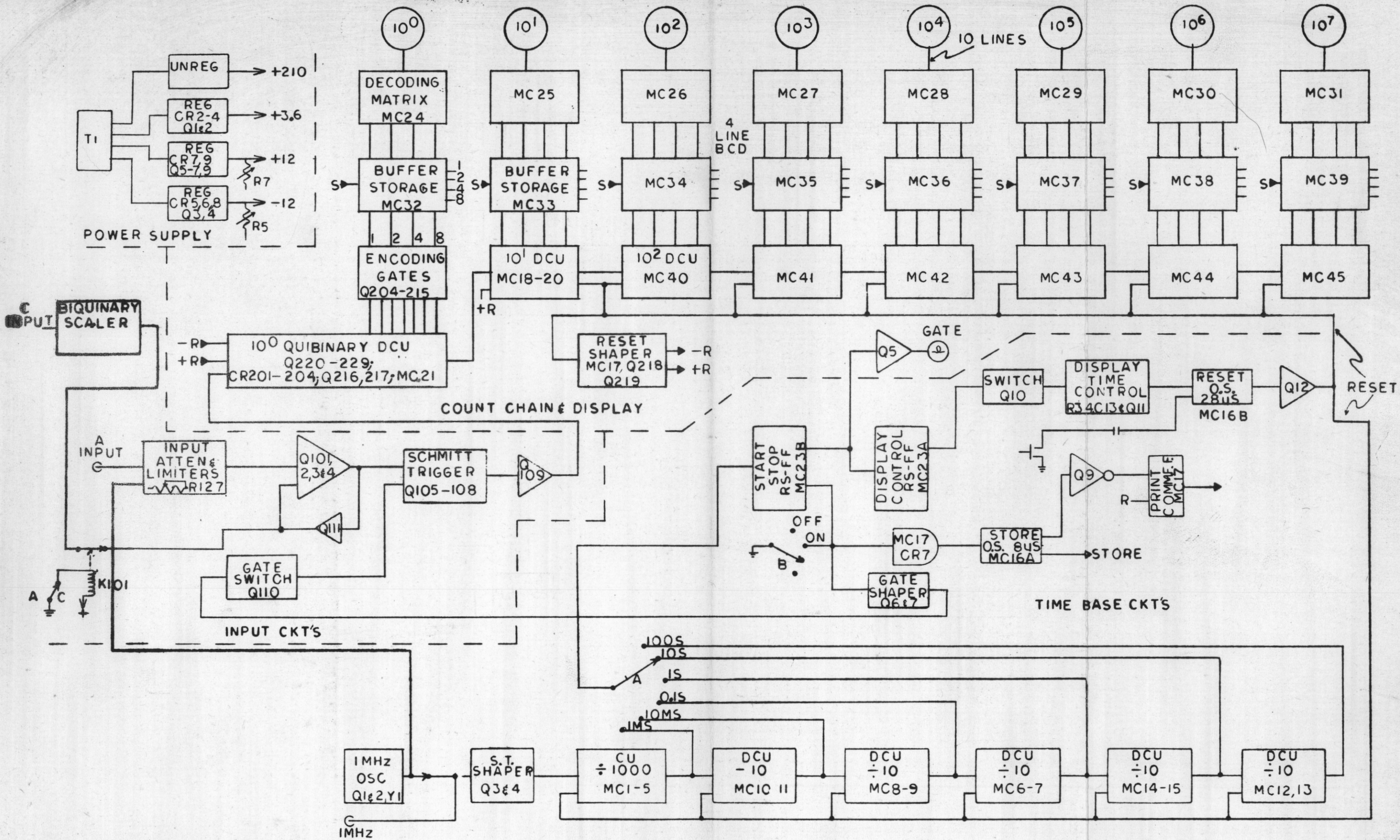
MODEL 1650 FIGURE 3-1 SIMPLIFIED BLOCK DIAGRAM
