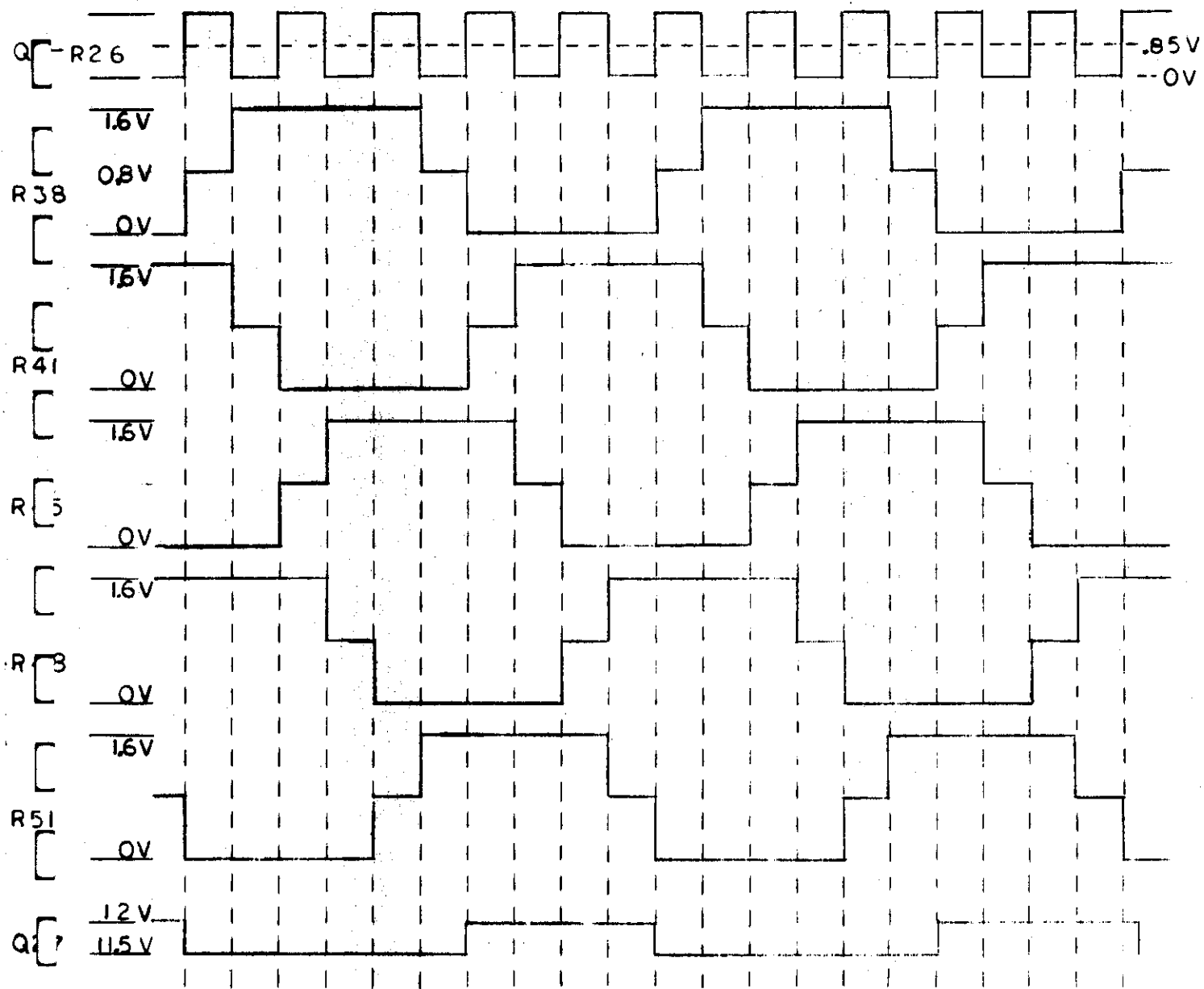
Figure 3-2 Quinary Counter Bias Waveforms and Timing
