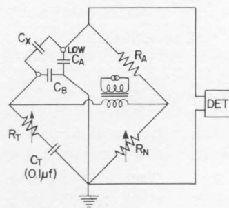
Figure 11. Capacitance to Ground for Capacitance Measurement.
