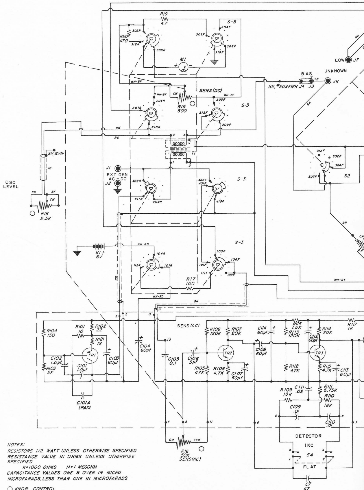
Figure 22. Schematic
