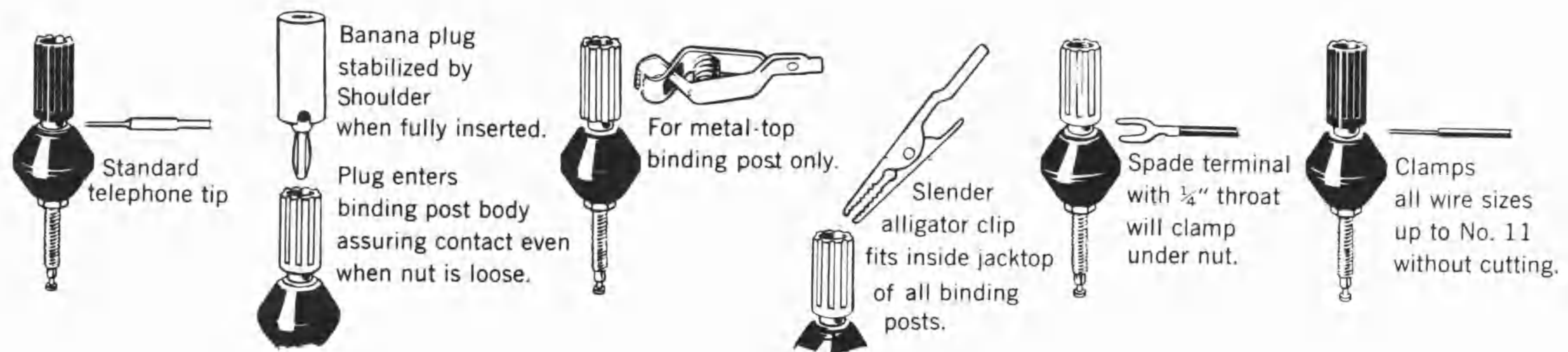
Figure 1-7. Methods of connection to the measurement terminals.
