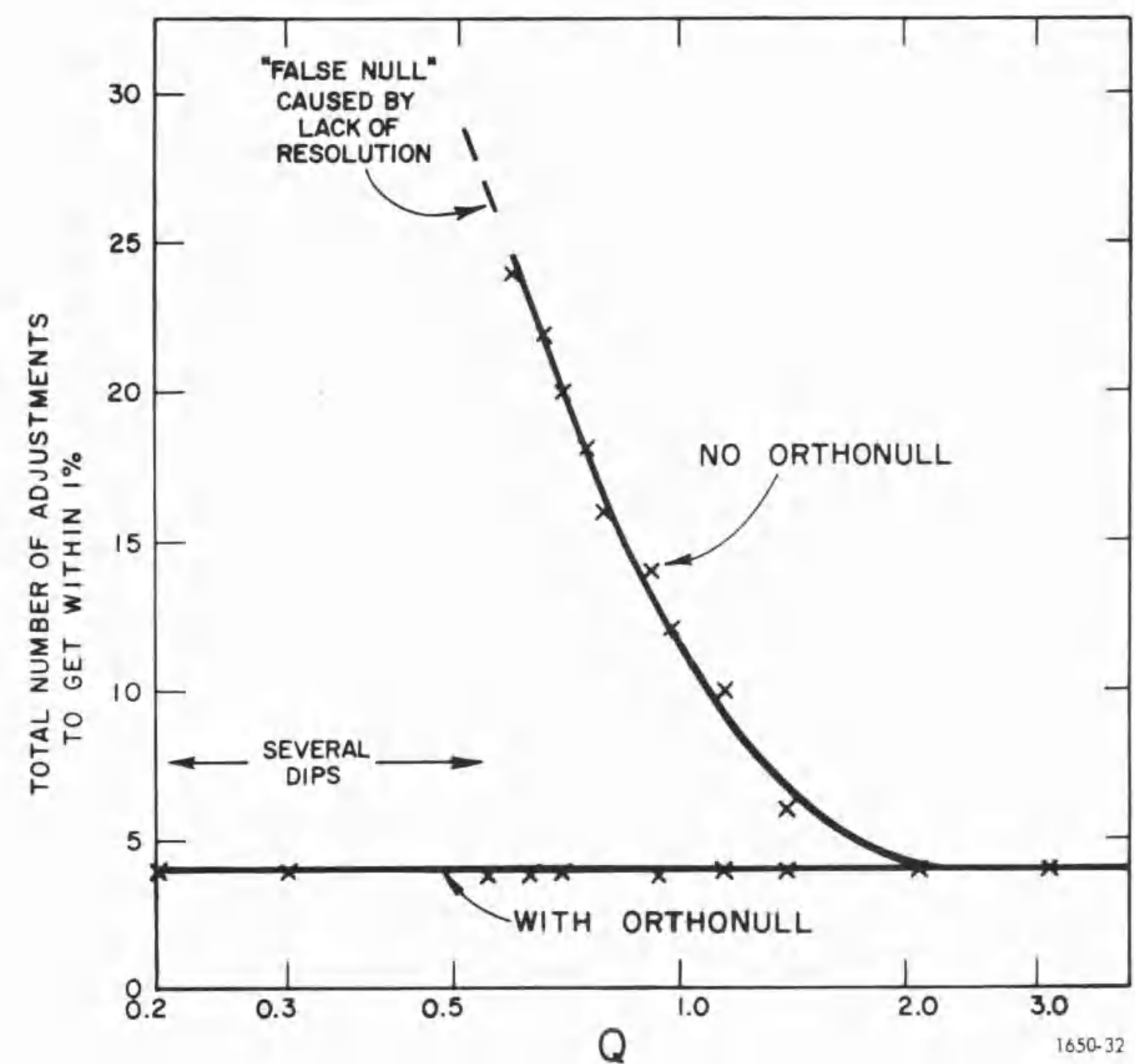
Figure 4-3. Number of balances vs Q .
