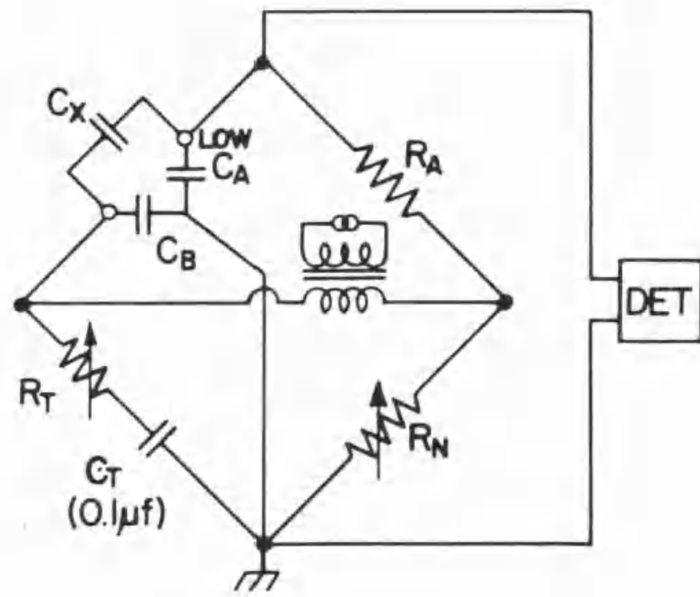
Figure 4-1. Capacitance to ground for capacitance measurement.
