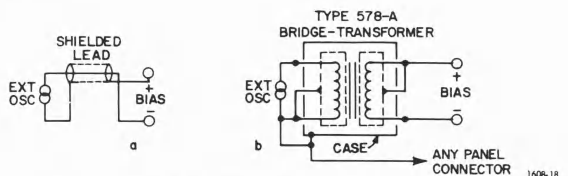
Figure 2-3. Methods of applying external ac.
