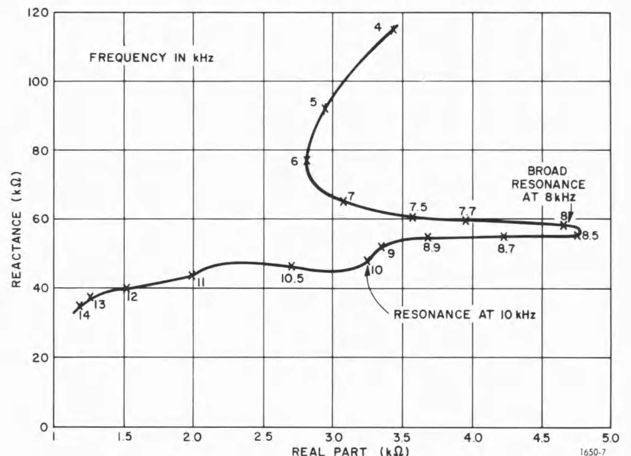
Figure 3-9. Typical impedance-vs-frequency response of a piezoelectric microphone.
