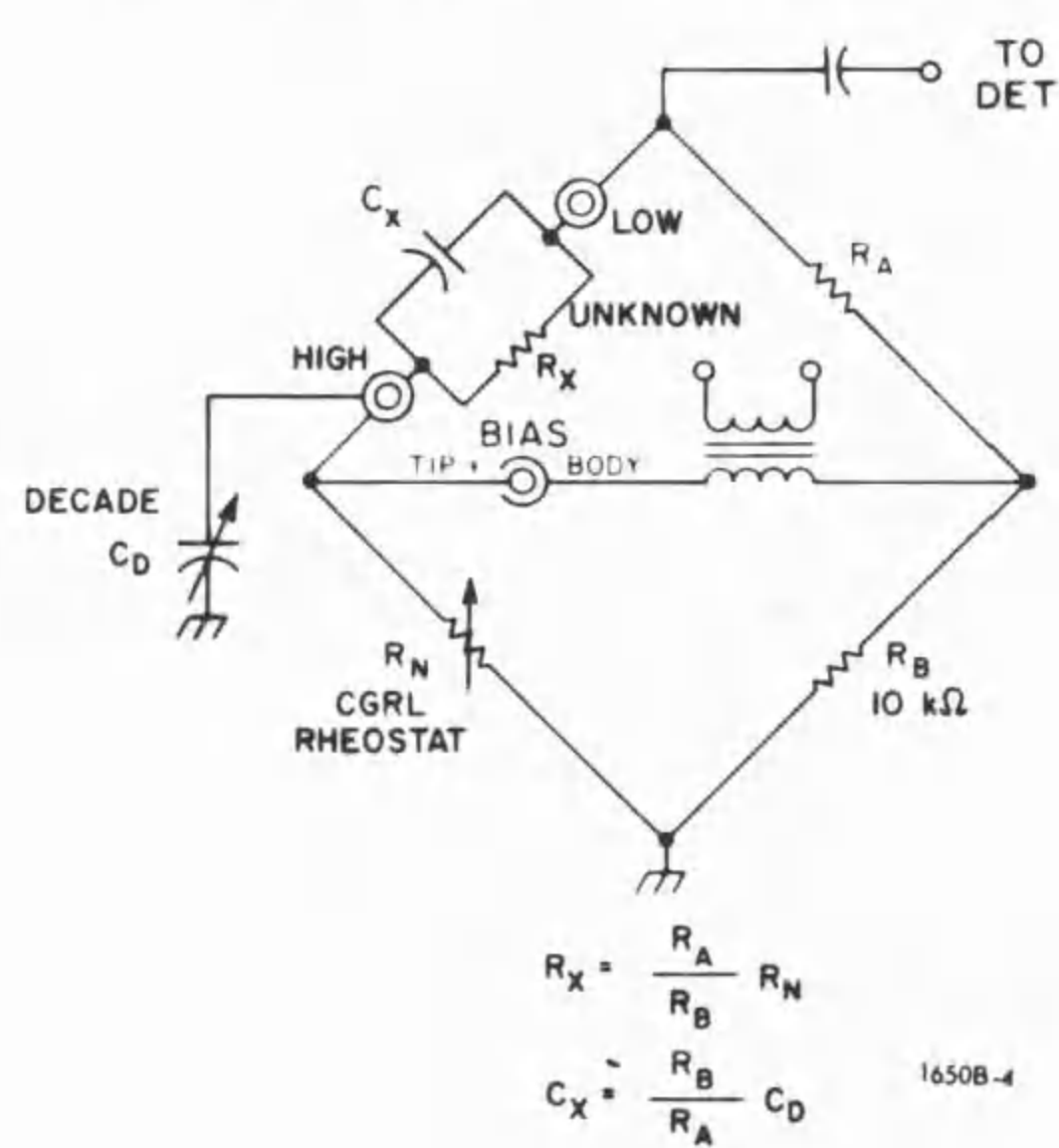
Figure 3-6. Circuit for measuring capacitive resistors.
