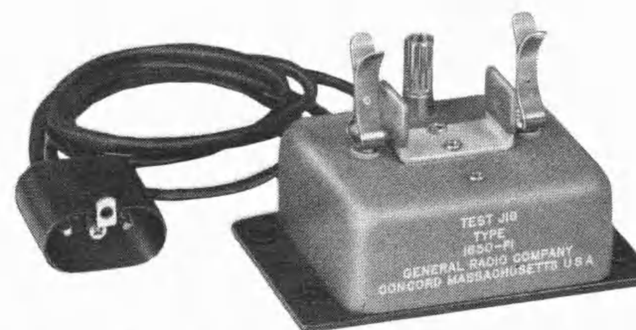
Figure 3-11. Type 1650-P1 Test Jig.
