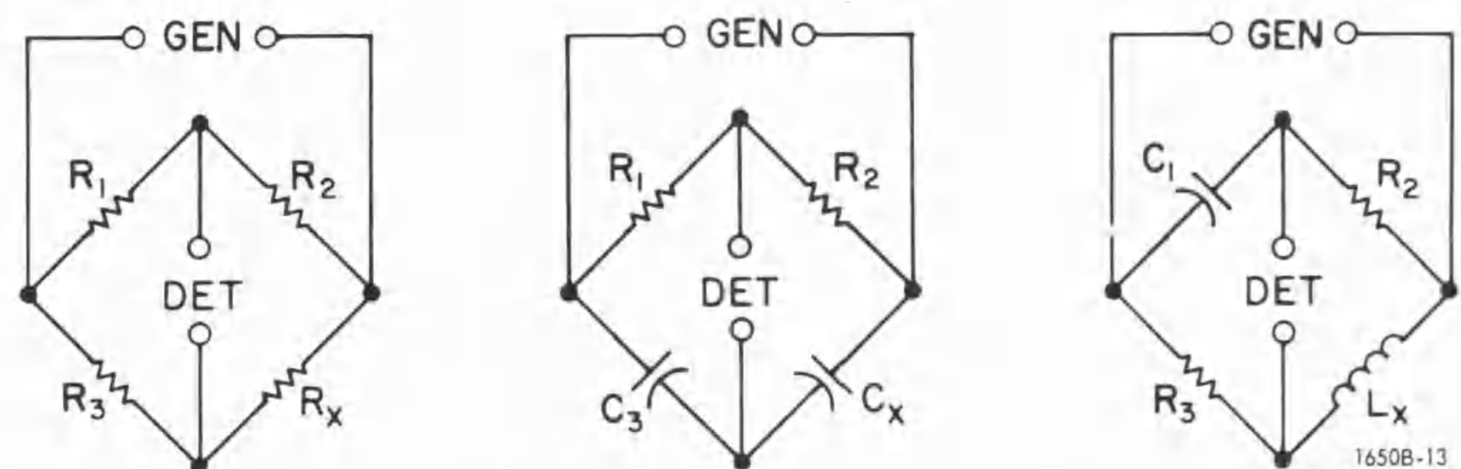
Figure 5-1. The general Wheatstone bridge circuit.
