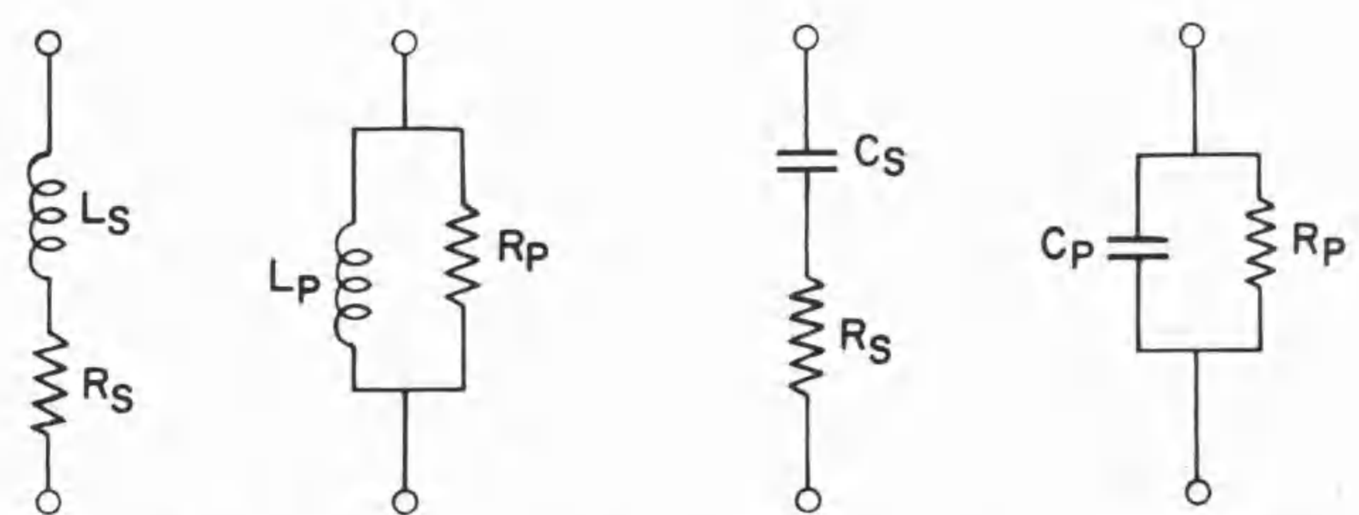
Figure 1-3. Equivalent circuits for complex impedance.
