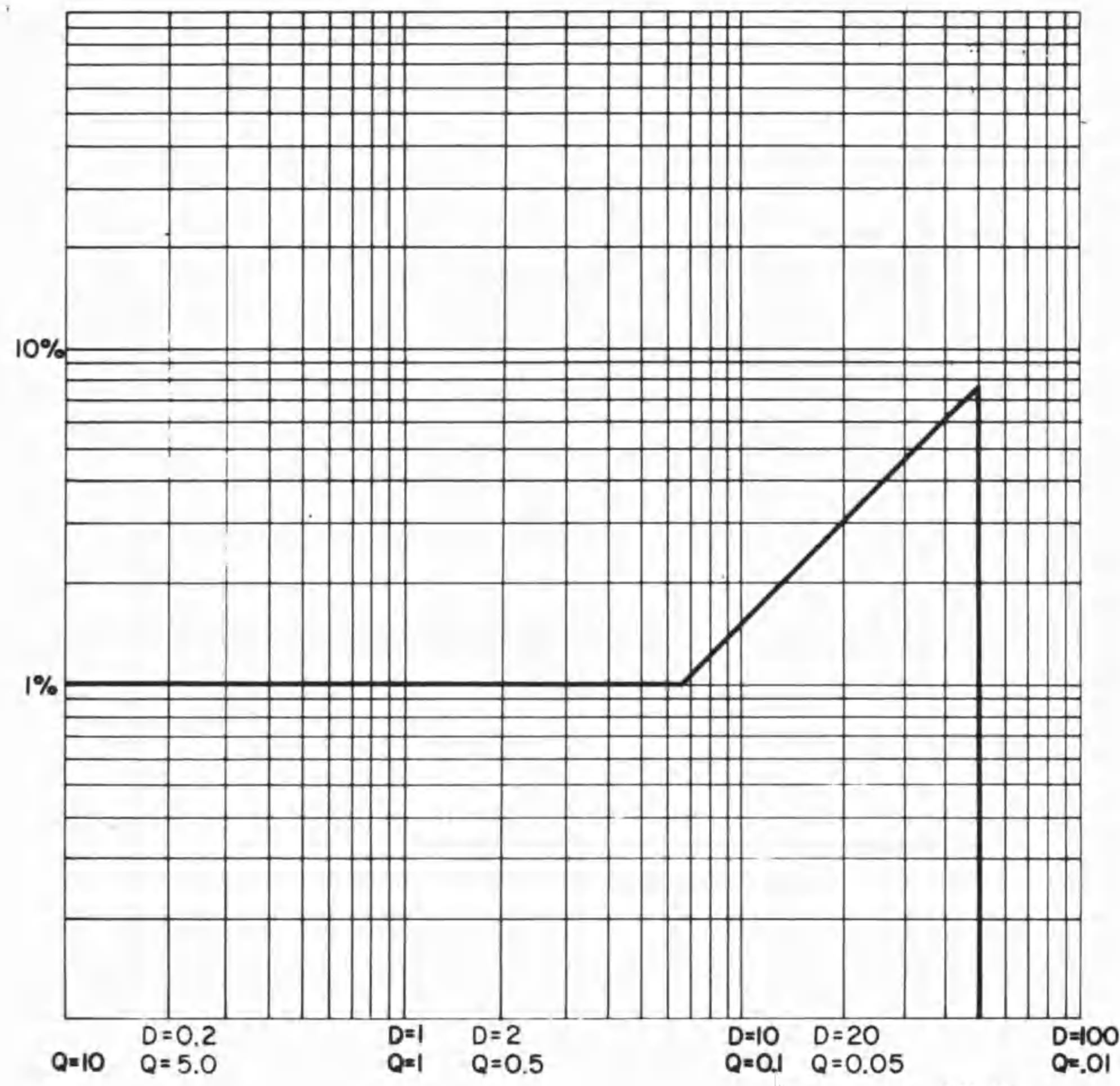
Figure 4-4. Accuracy vs D or Q.
