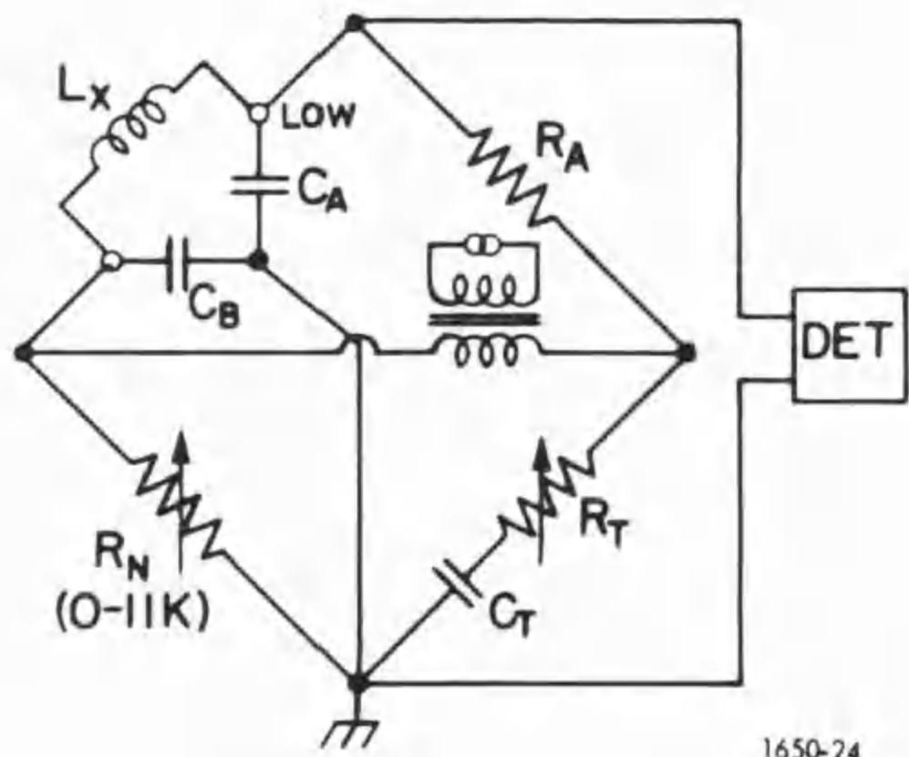
Figure 4-2. Capacitance to ground for inductance measurement.
