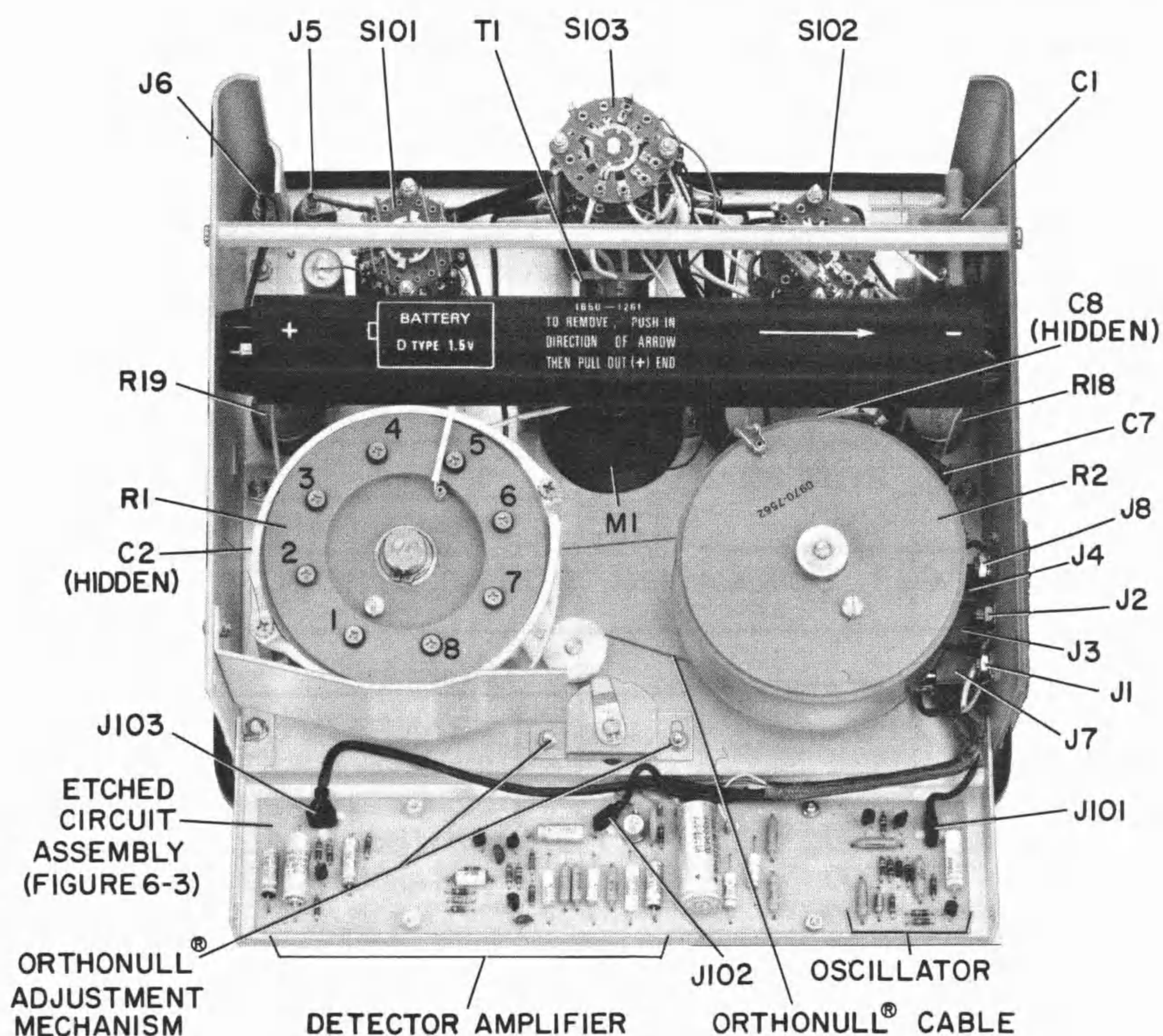
Figure 6 - 2. Interior view of 1650-B Bridge.
