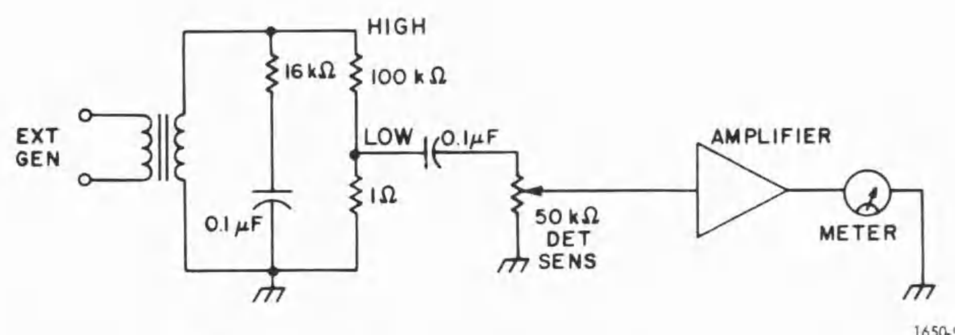
Figure 6 - 3. Schematic for checking the detector circuit.
