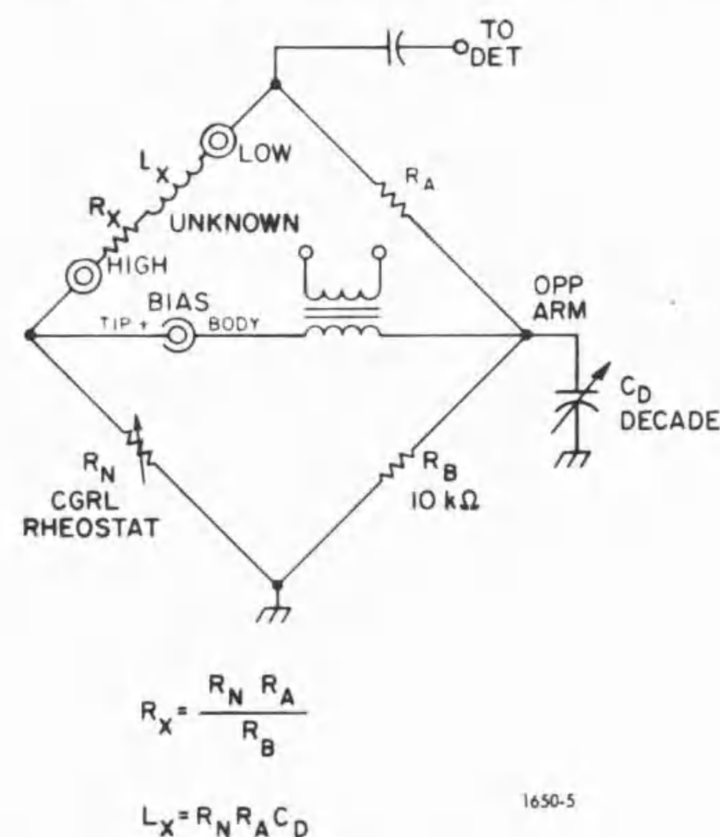
Figure 3-7. Circuit for measuring inductive resistors.
