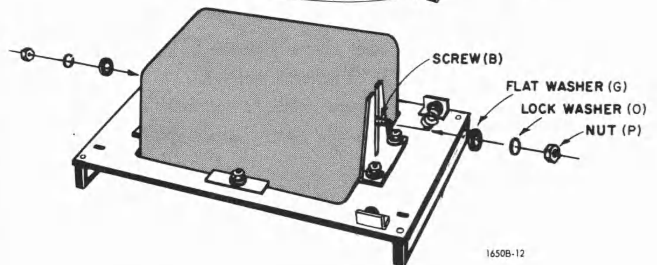
Figure 1-4. Rack mounting the 1650-B.
