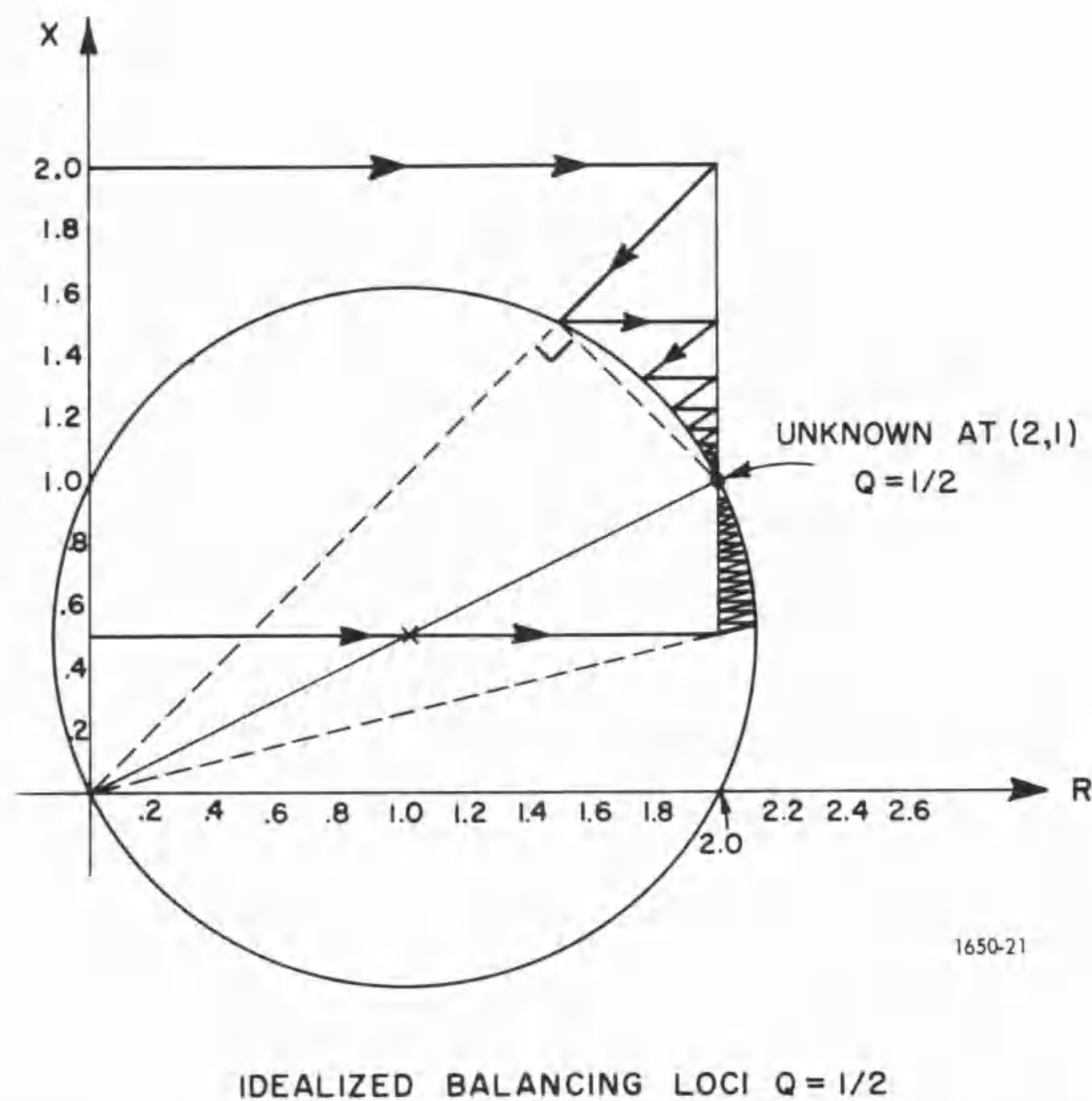
Figure 5-8. Loci of "sliding null" balance.
