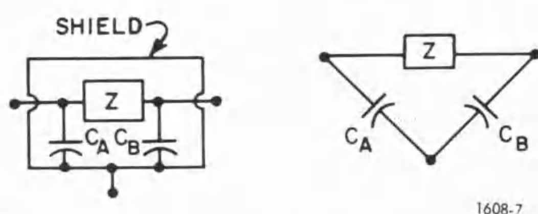
Figure 3-10. Shielded three-terminal impedance.
