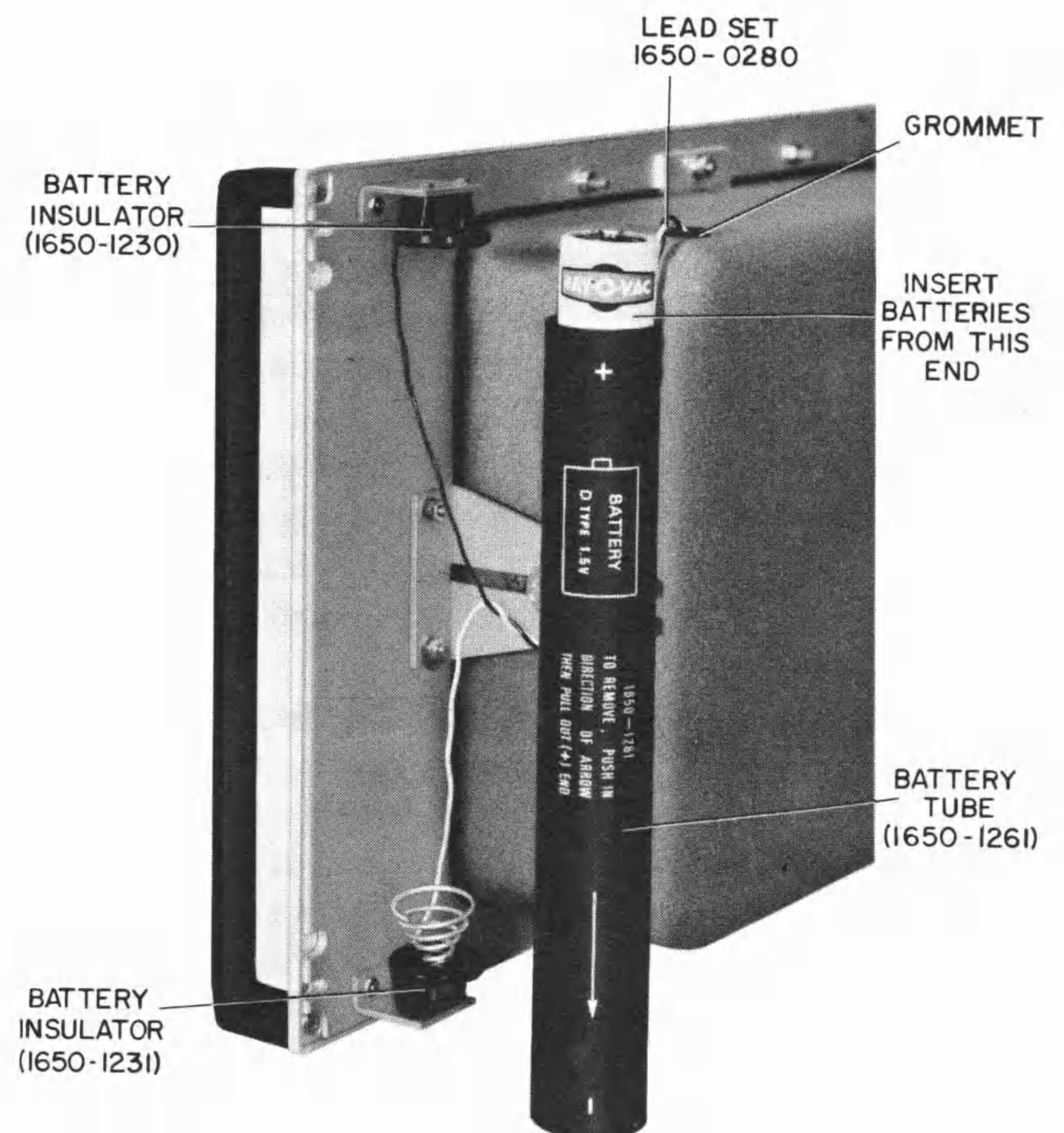
Figure 1-6. Battery mounting for rack-mounted 1650-B Bridge.
