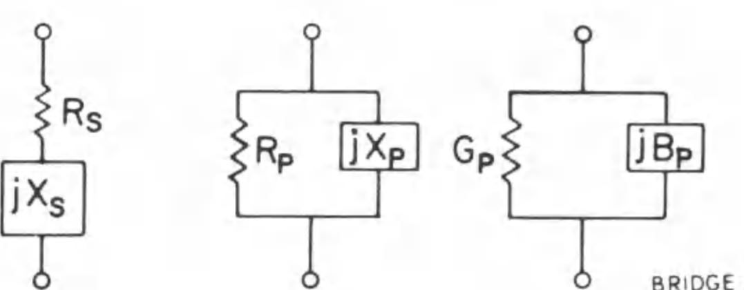
Figure 5-5. Series and parallel components of impedance.
