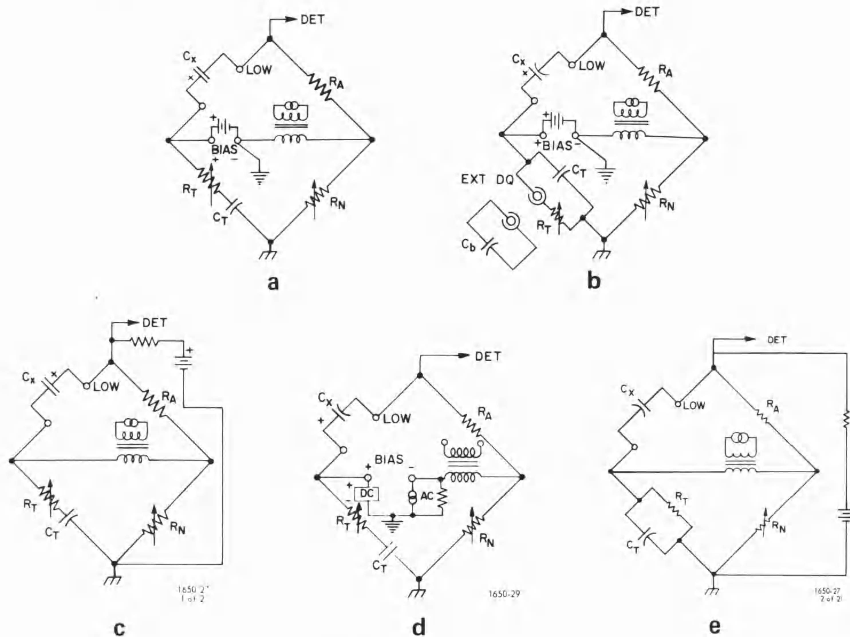
Figure 3-1. Methods of applying dc voltages to capacitance.
