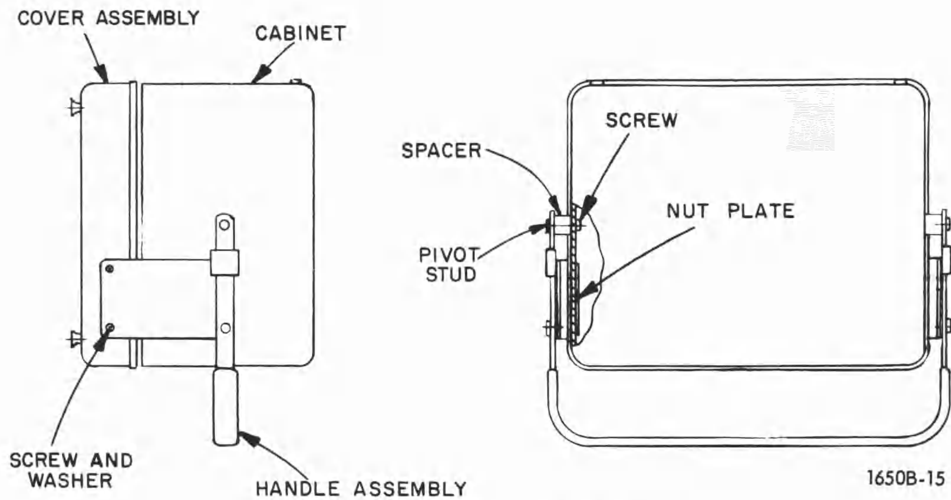
Figure 6 - 7. Complete cabinet assembly (P/N 4182-2002).
