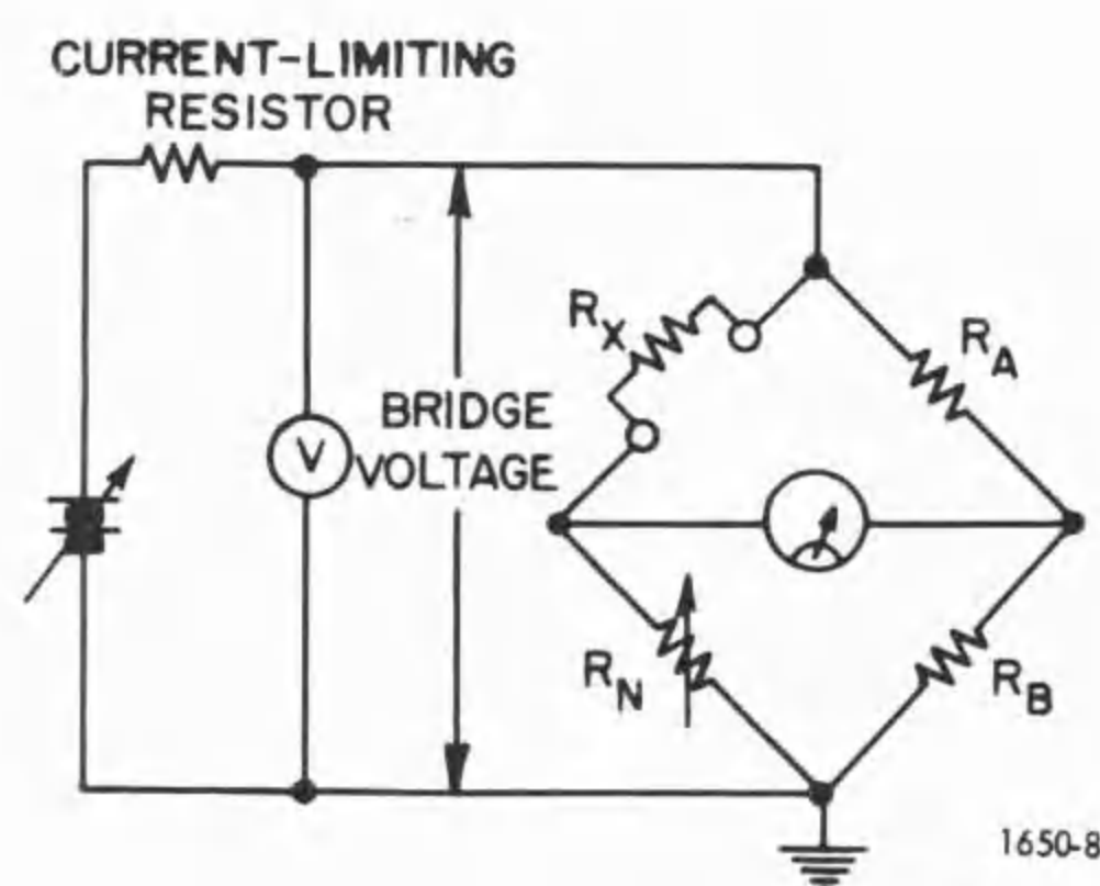
Figure 2-2. Circuit for standard test voltage measurements.
