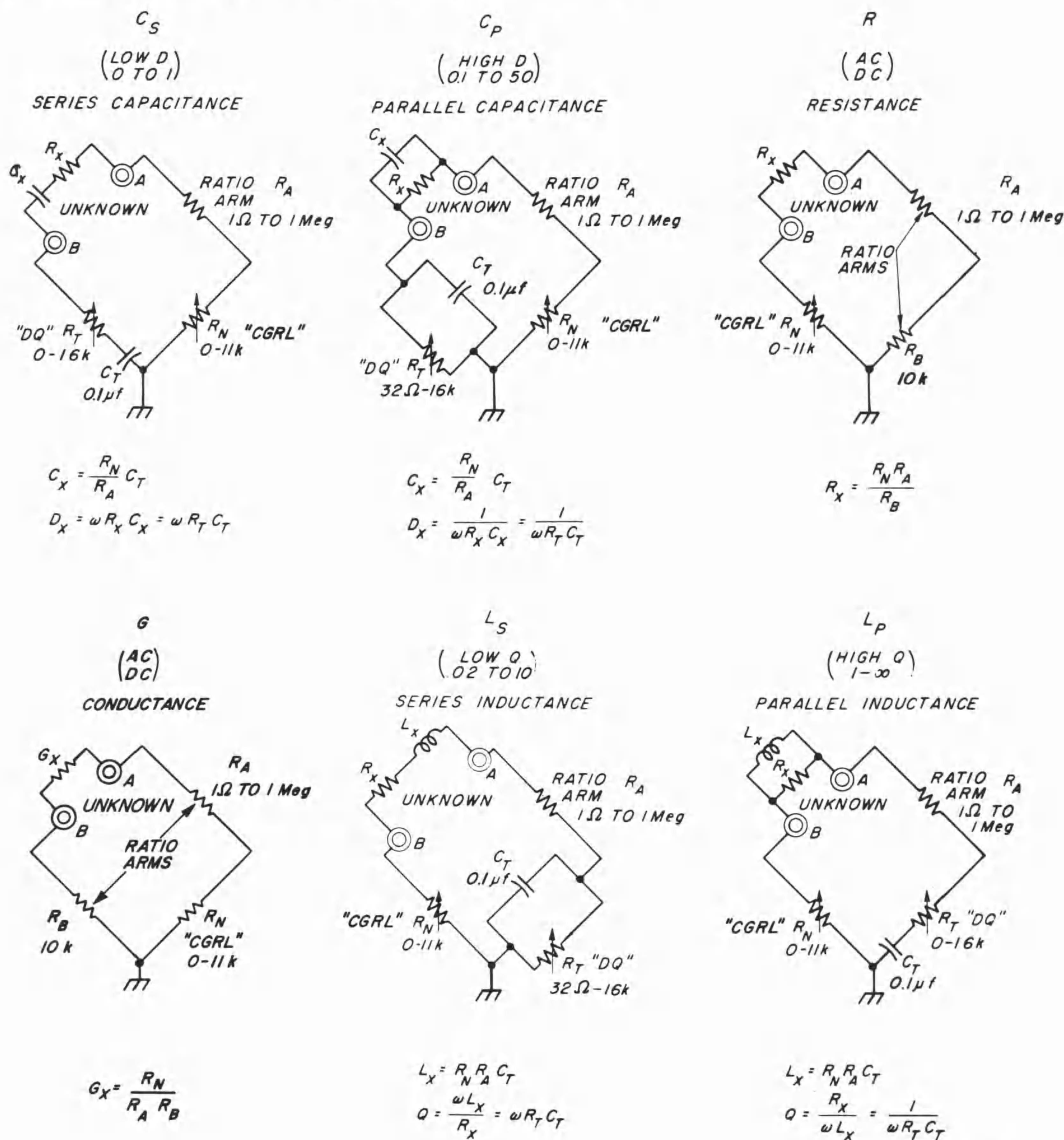
Figure 2-1. Bridge circuits used in impedance bridge.
