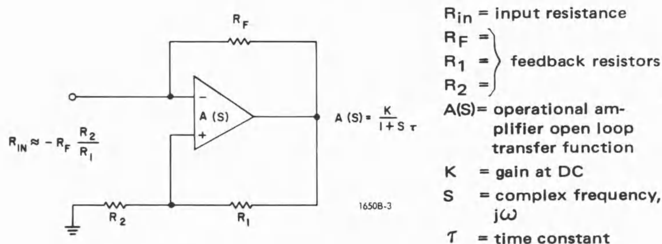
Figure 3-5. Operational amplifier.
