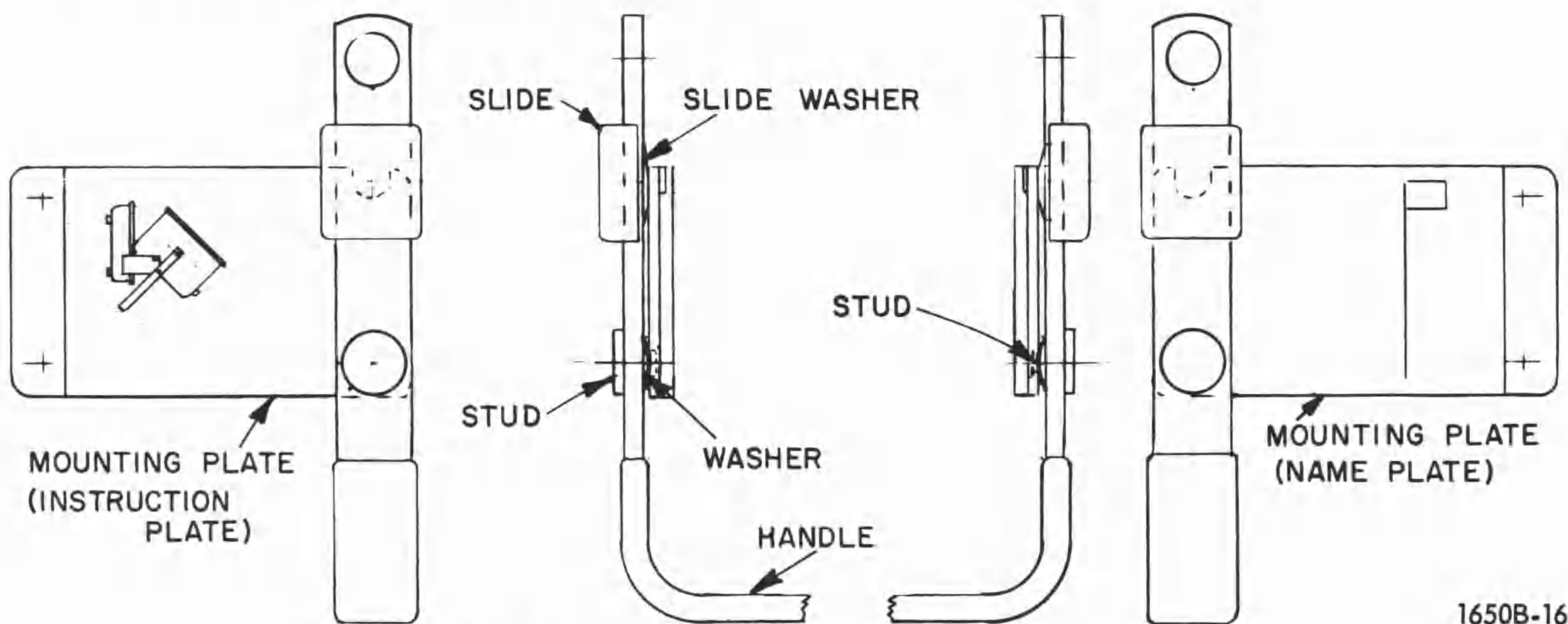
Figure 6 - 8. Complete handle and mounting plate assembly (P/N 5361-2002).
