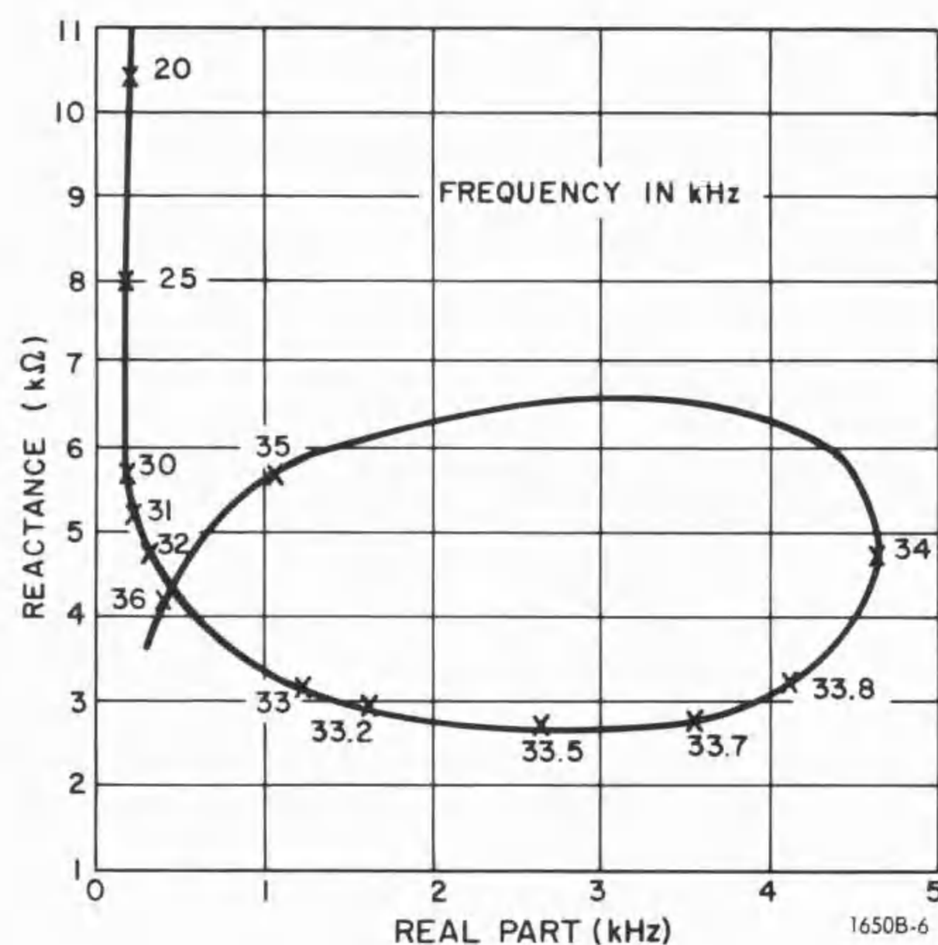
Figure 3-8. Typical impedance-vs-frequency response of an ultrasonic transducer.
