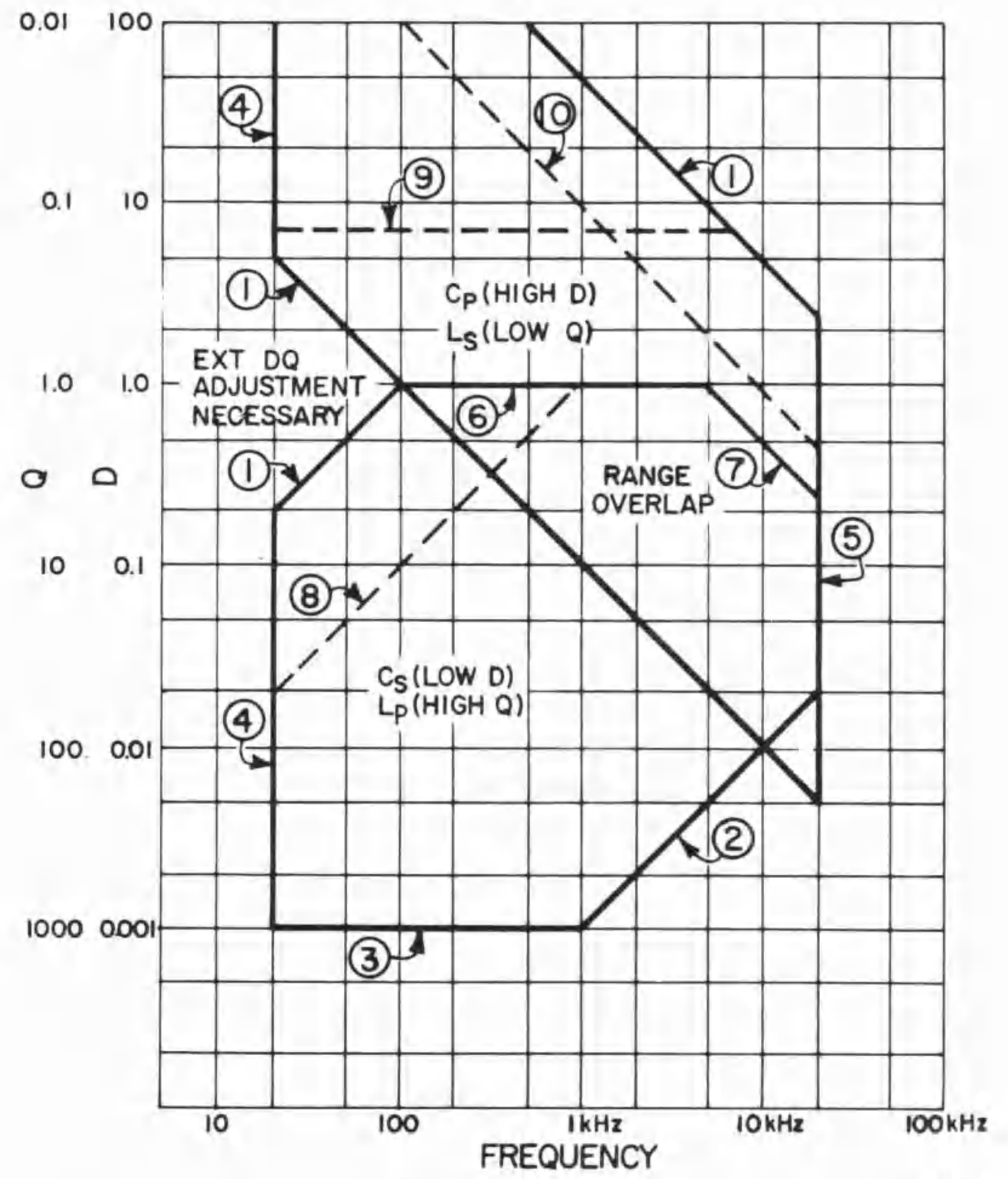
Figure 4-5. DQ ranges vs frequency.
