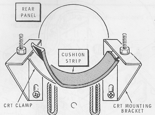
Detail 5-14A
