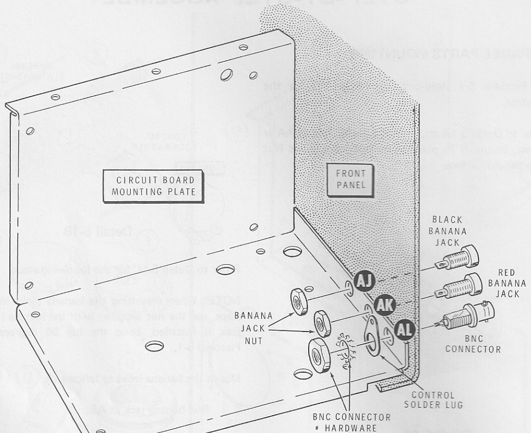
Detail 5-1D
