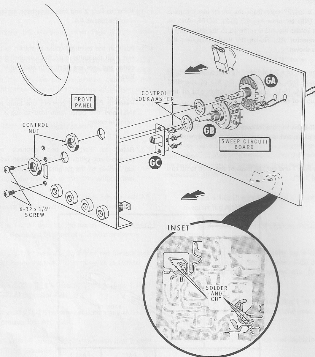
PICTORIAL 5-3
