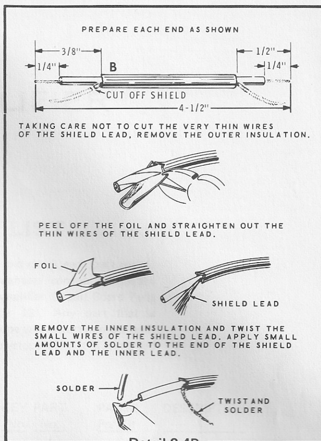
Detail 2-4B
