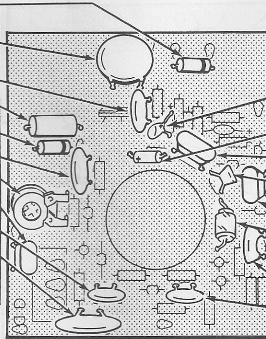
PICTORIAL 4-2
