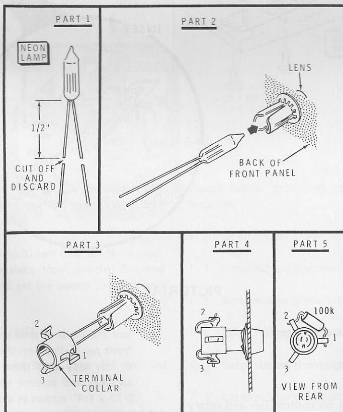
Detail 5-2A
