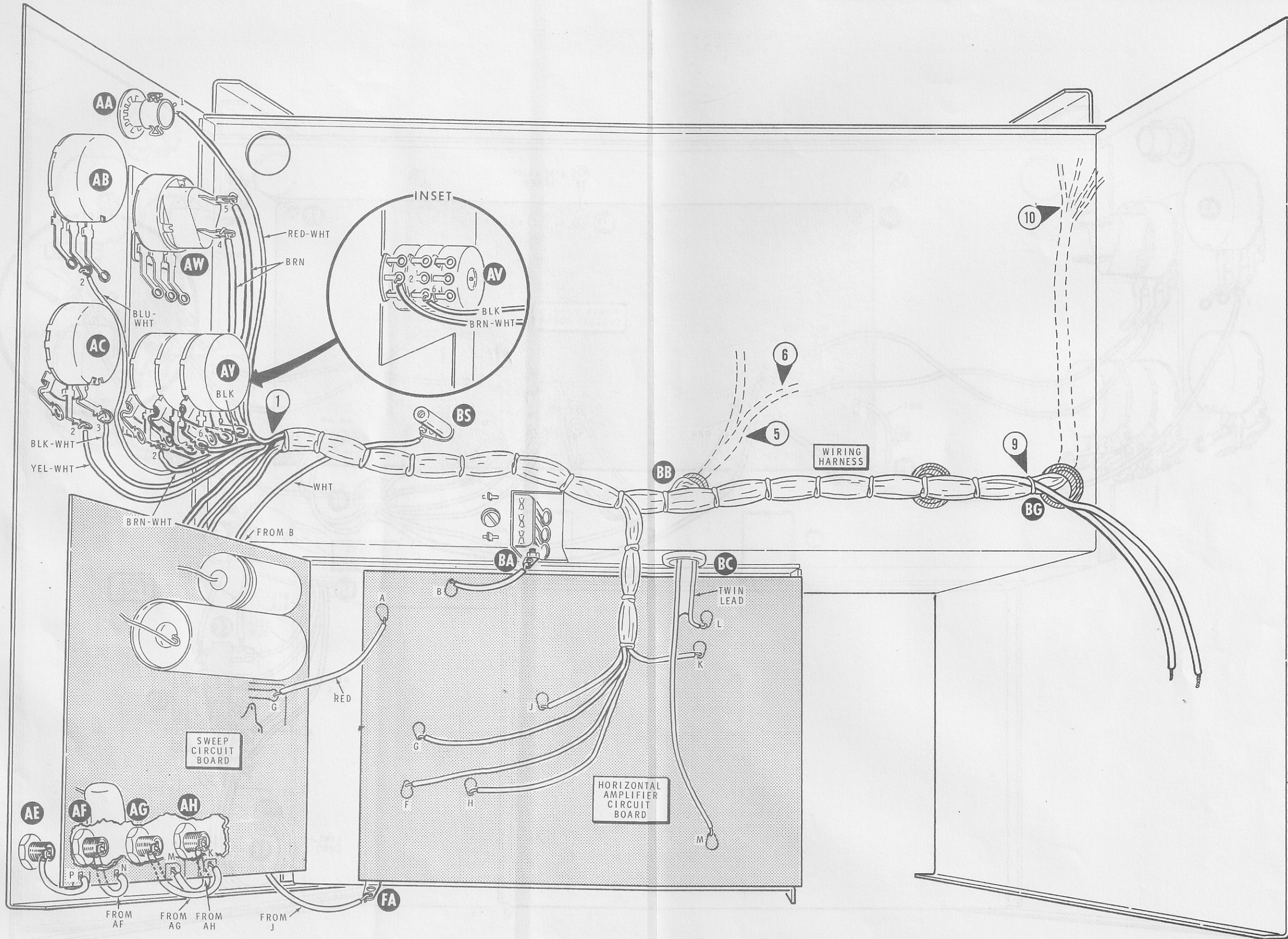
PICTORIAL 5-7
