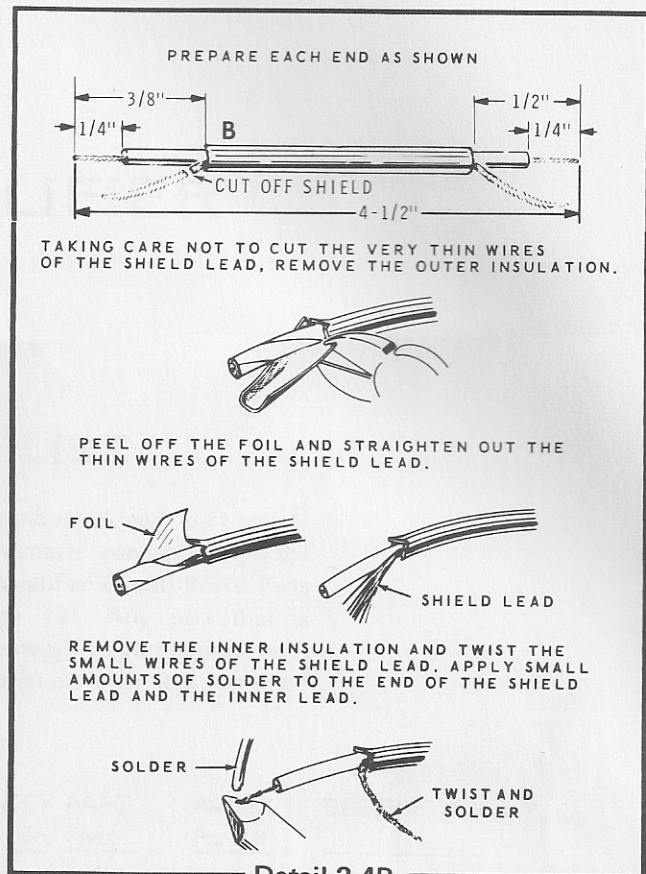
Detail 2-4B
