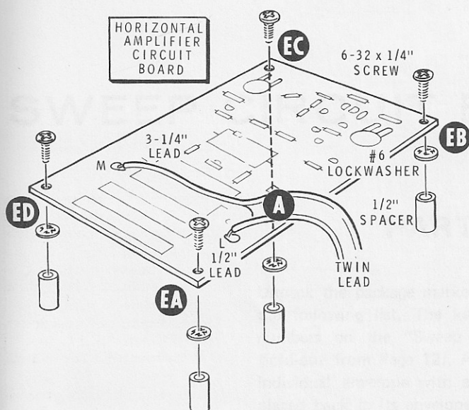
PICTORIAL 3-4
