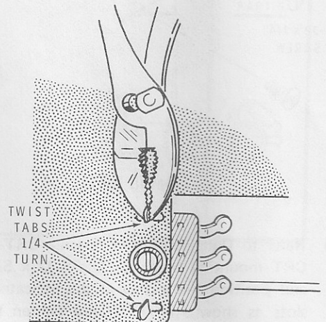
Detail 5-5C
