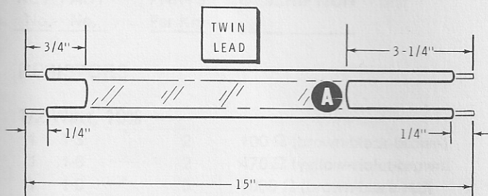
Detail 2-4A
