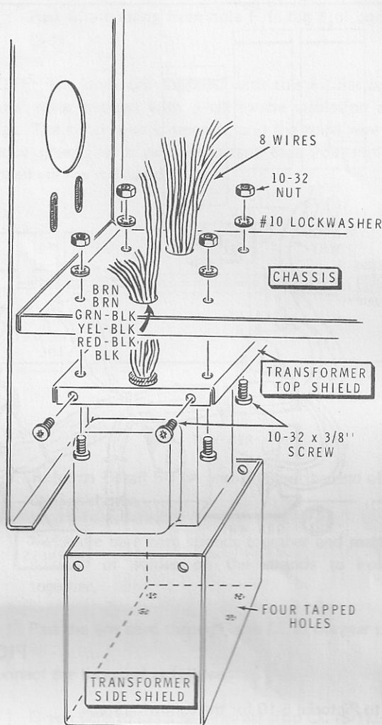
Detail 5-9A
