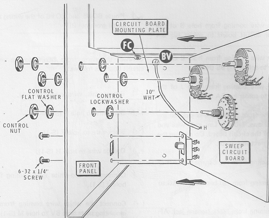
Detail 5-7D
