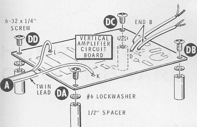
PICTORIAL 2-4
