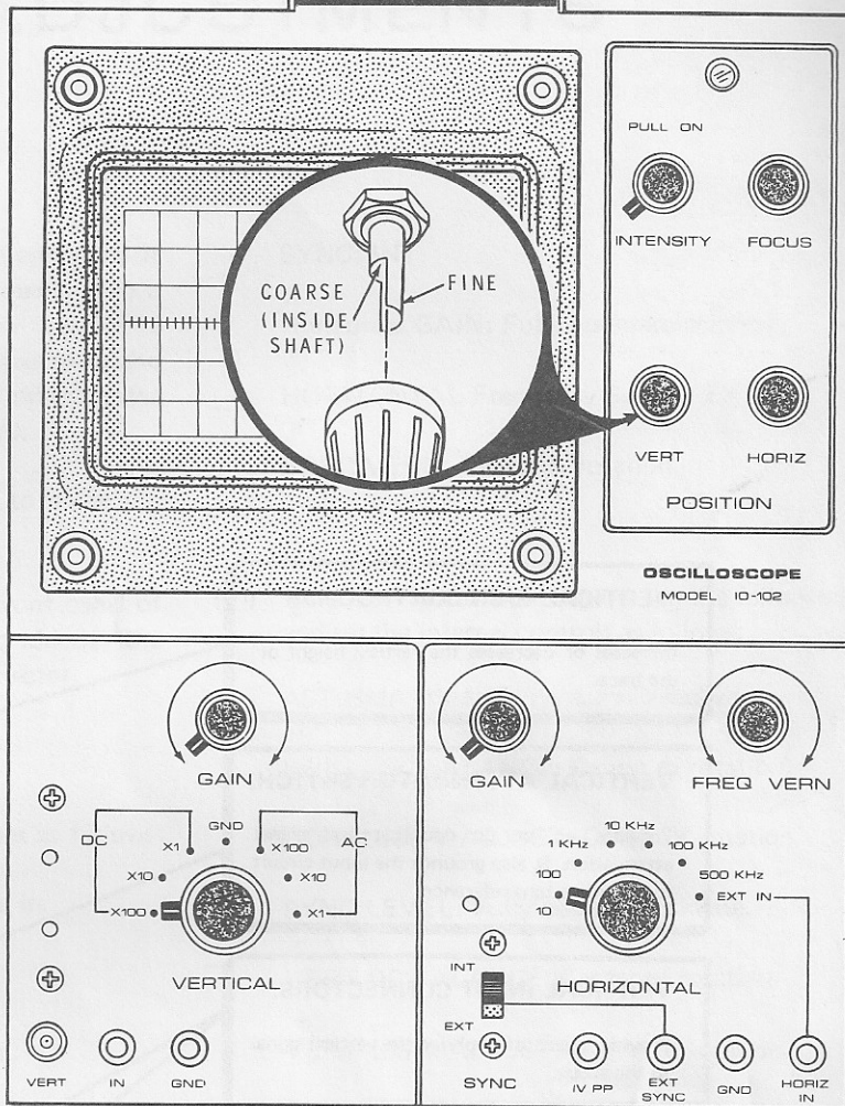
PICTORIAL 5-15
