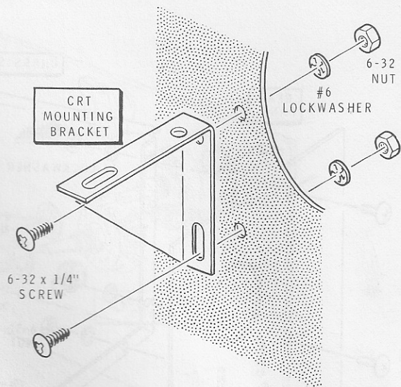
Detail 5-4C
