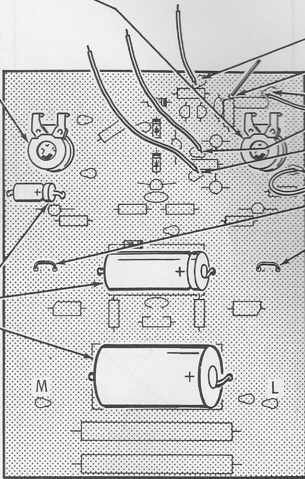
PICTORIAL 3-3
