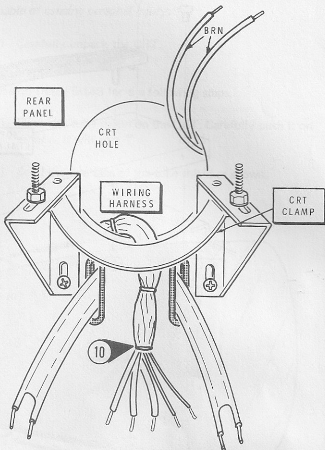
Detail 5-12A
