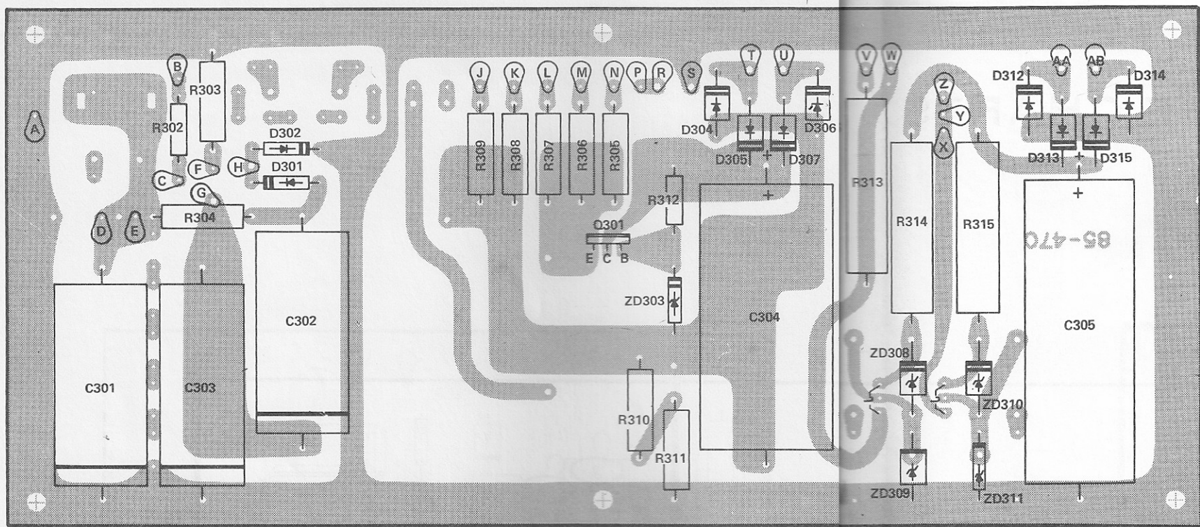
POWER SUPPLY CIRCUIT BOARD (Viewed from foil side)
