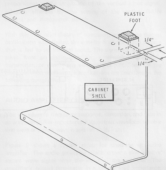
Detail 6-1A
