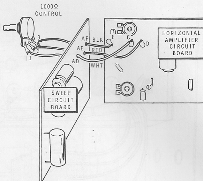
Detail 5-7A
