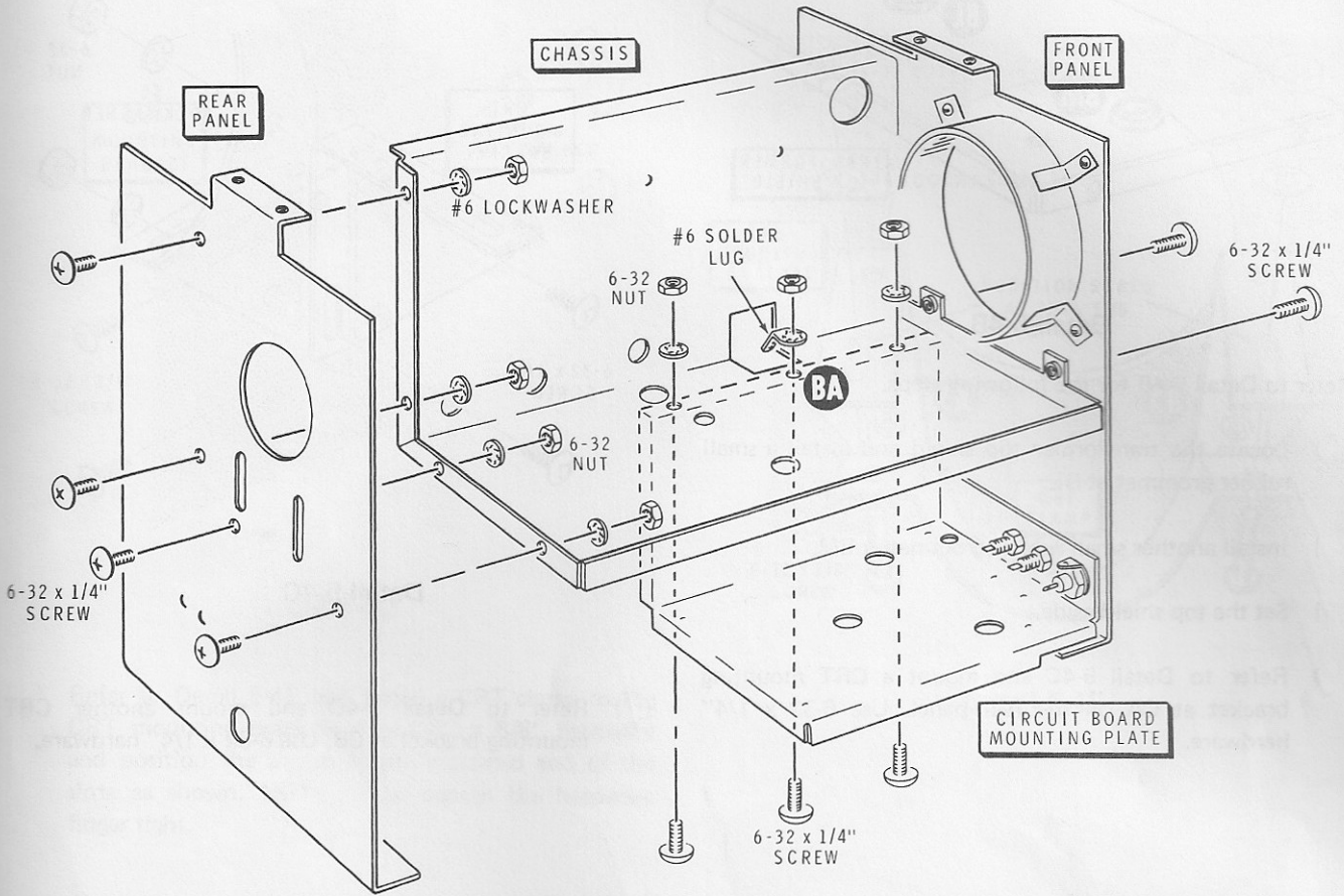
Detail 5-4A
