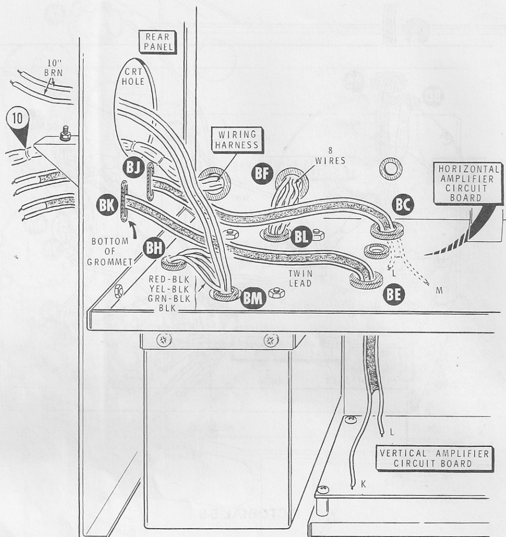
PICTORIAL 5-9
