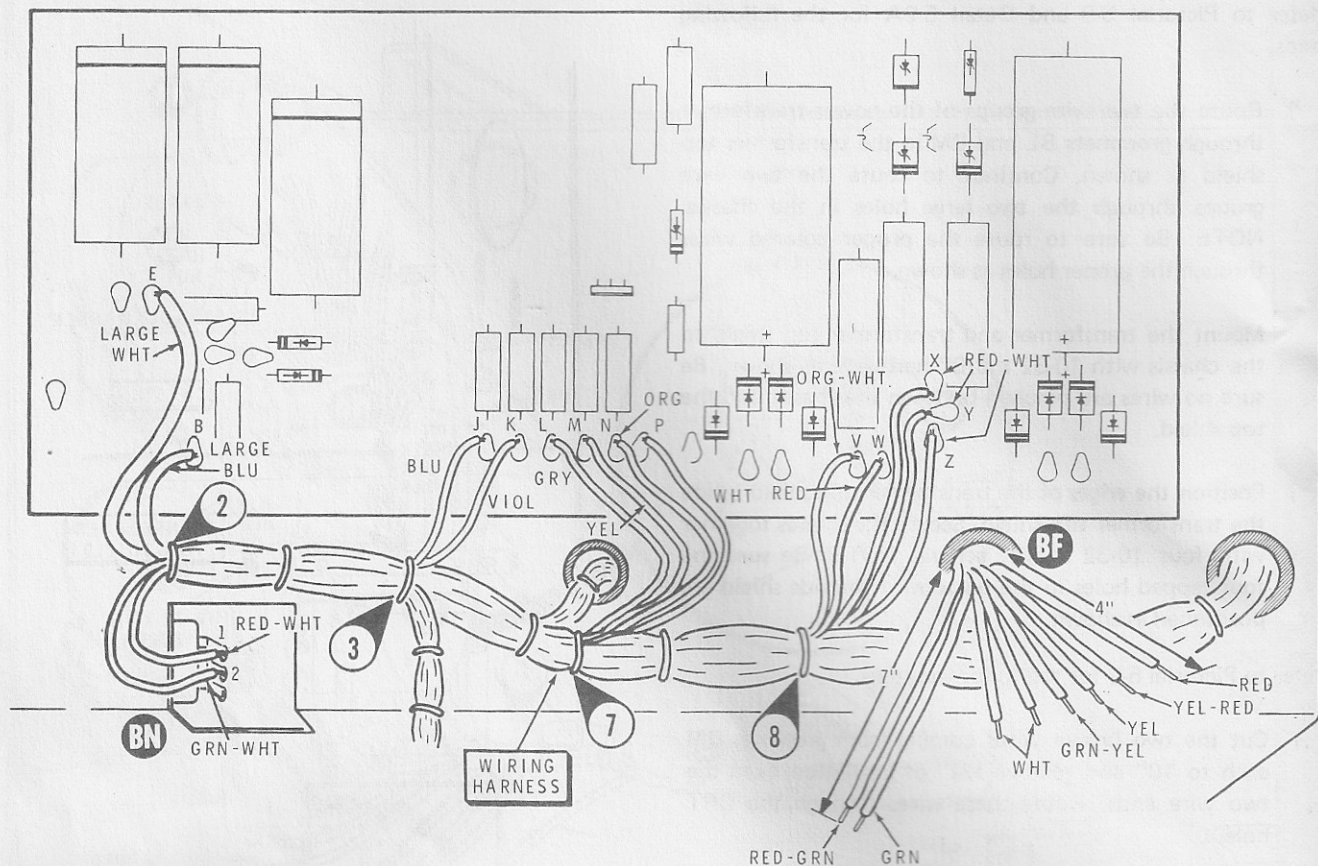
PICTORIAL 5-10
