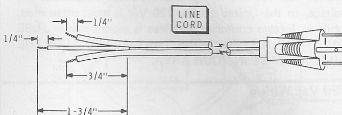
Detail 5-11A
