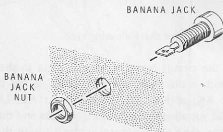
Detail 5-1C
