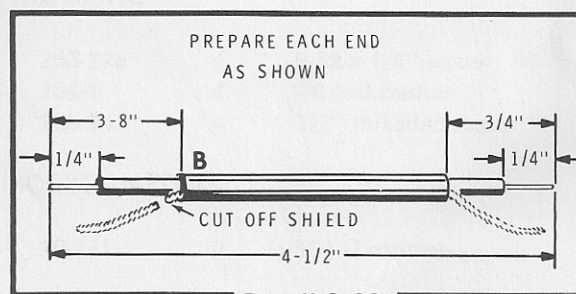
Detail 2-4C
