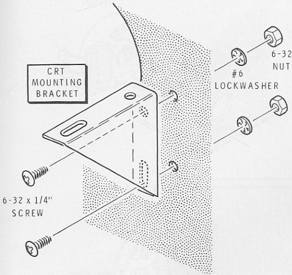
Detail 5-4D
