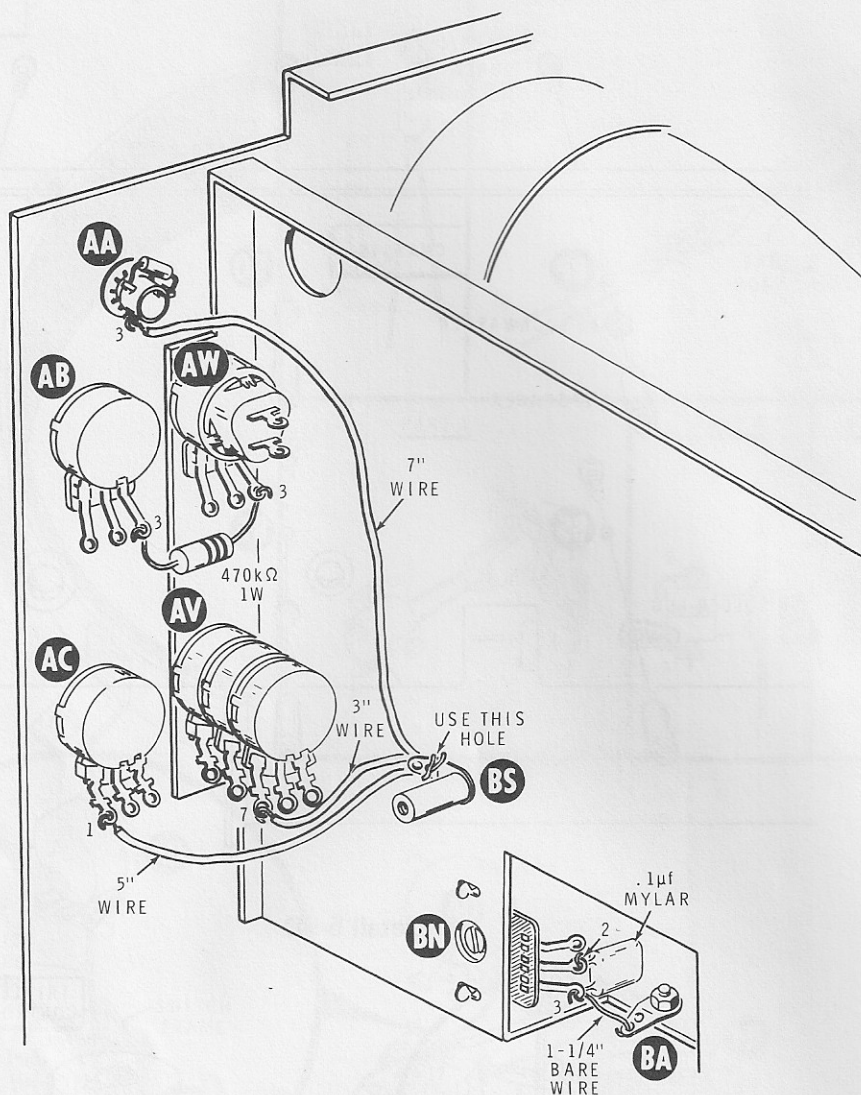
PICTORIAL 5-6
