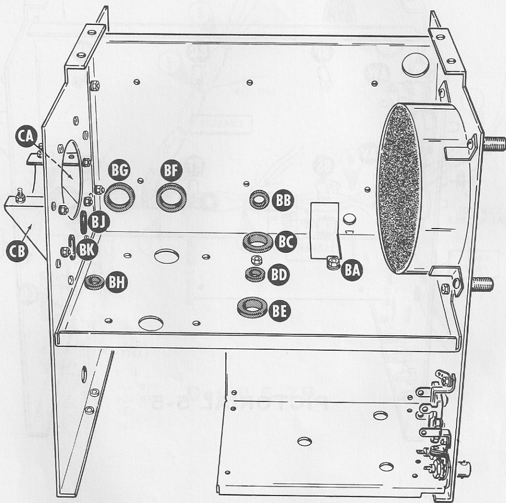
PICTORIAL 5-4
