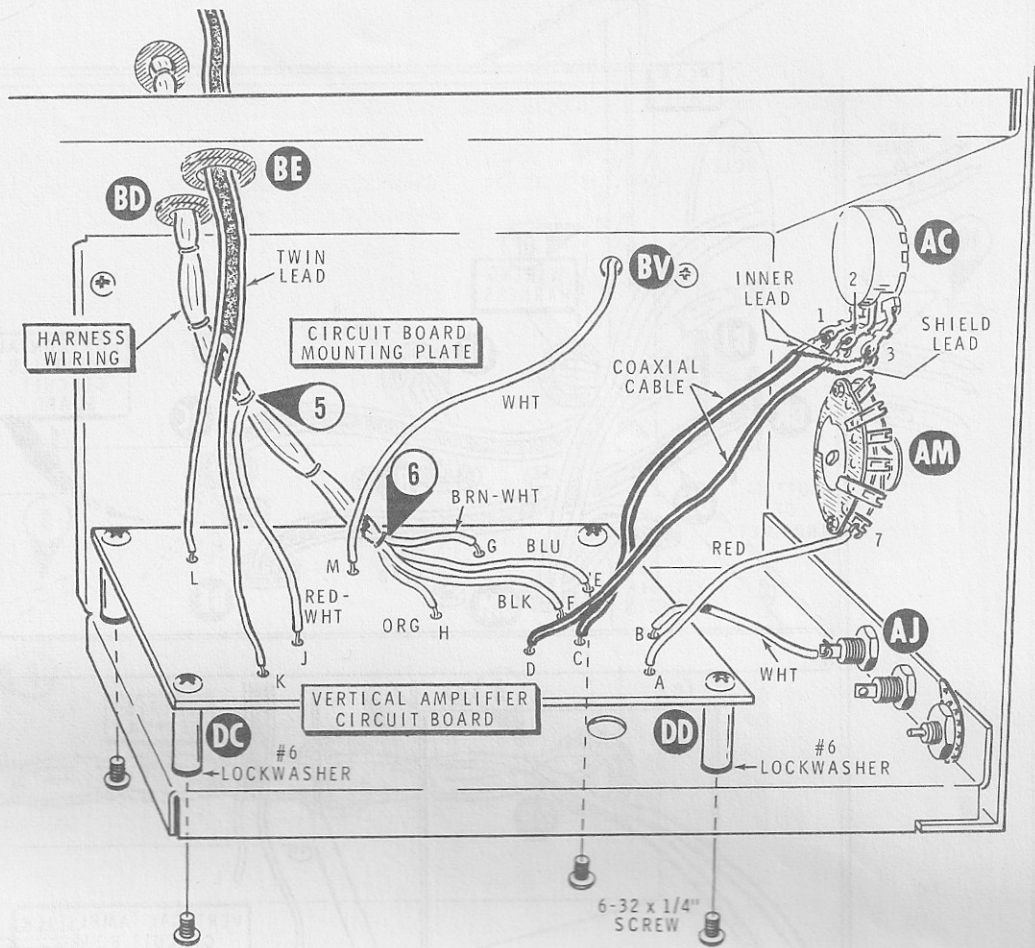
PICTORIAL 5-8
