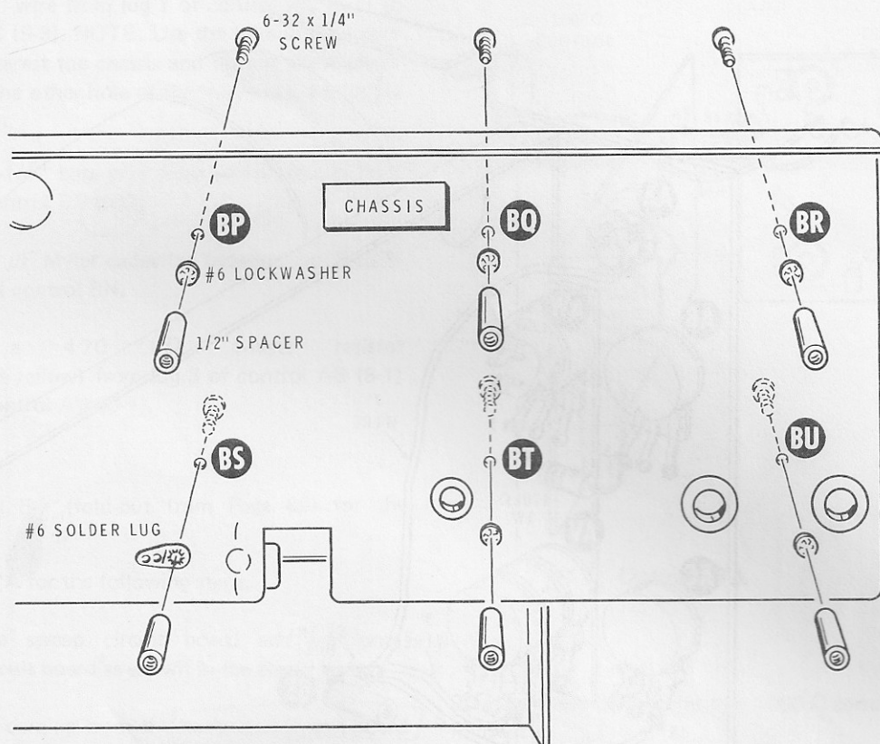
Detail 5-5D
