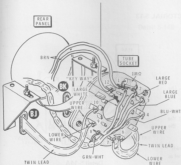
PICTORIAL 5-12
