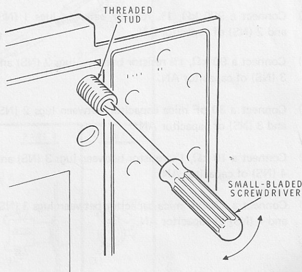
Detail 5-1H
