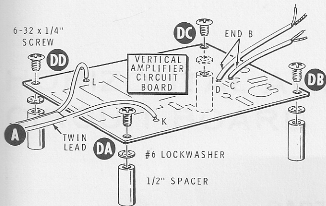
PICTORIAL 2-4
