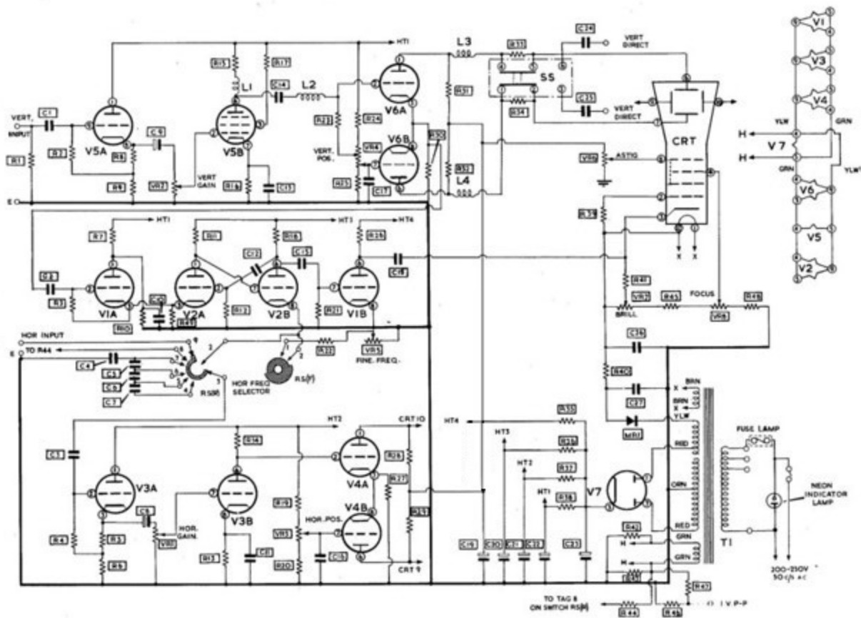
CIRCUIT DIAGRAM HEADHILL SERVICE CORPORATION Model 95-2
