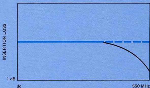
Figure 6. Typical frequency response of a step attenuator.
