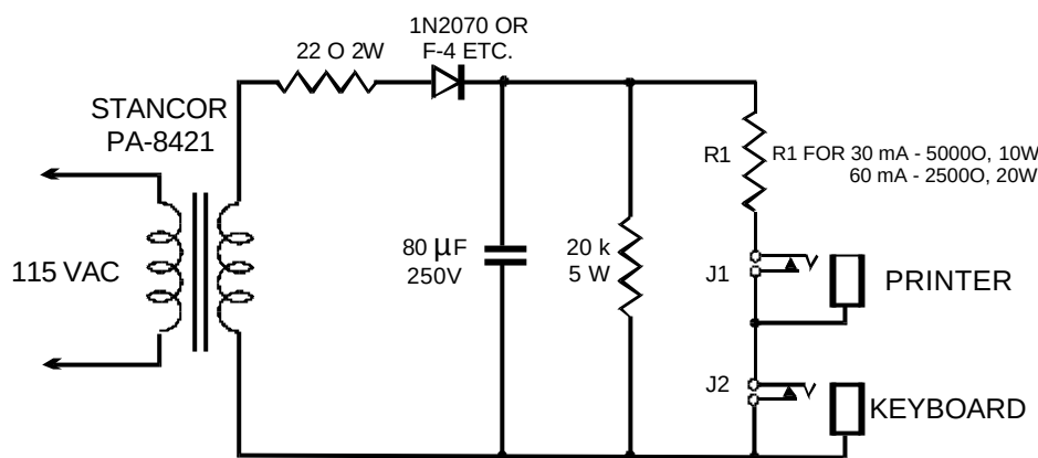
LOCAL LOOP SUPPLY FIGURE 1
