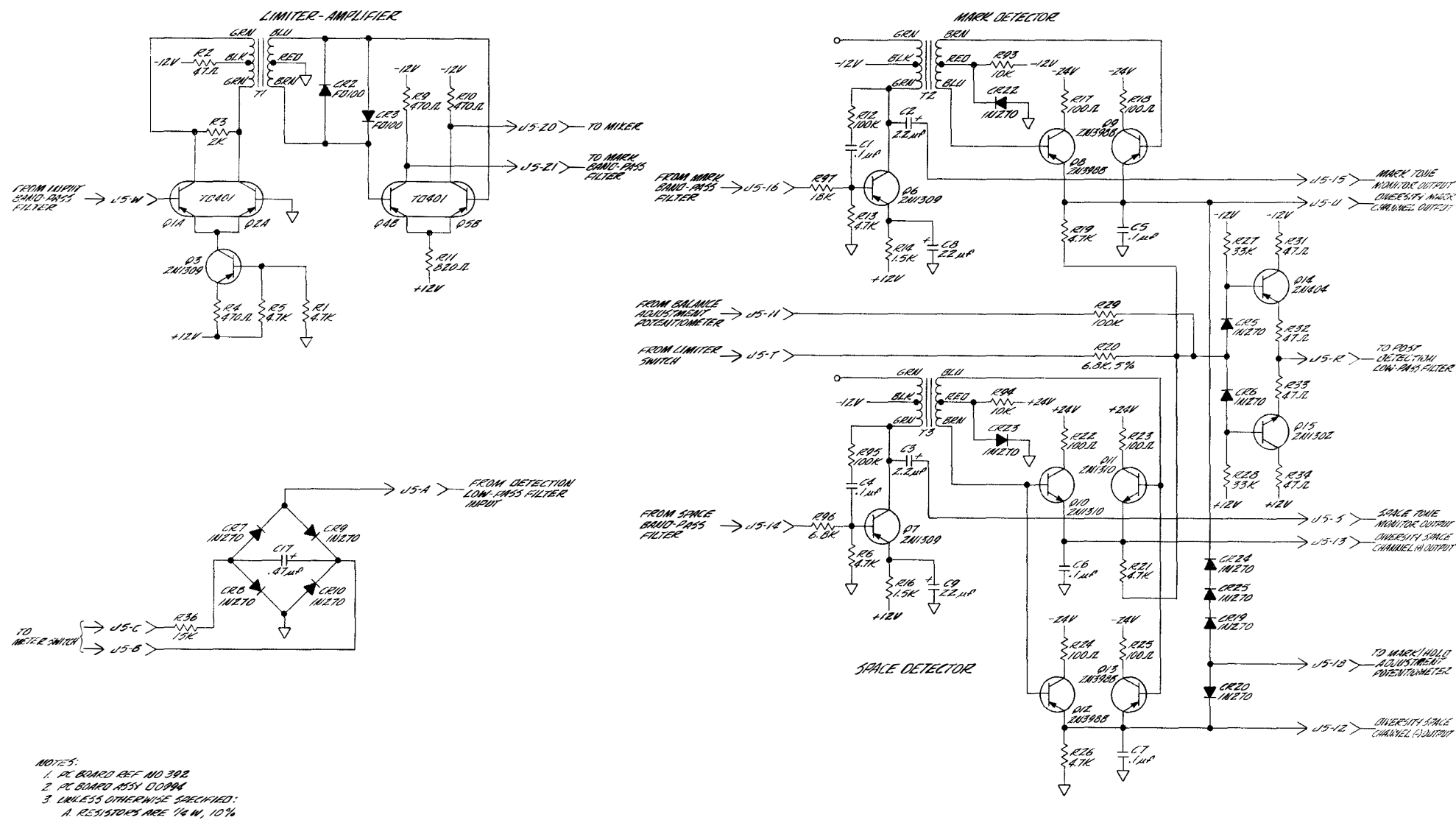
Figure 6-2. Detector Circuits Schematic Diagram D3668A, Sheet 1
