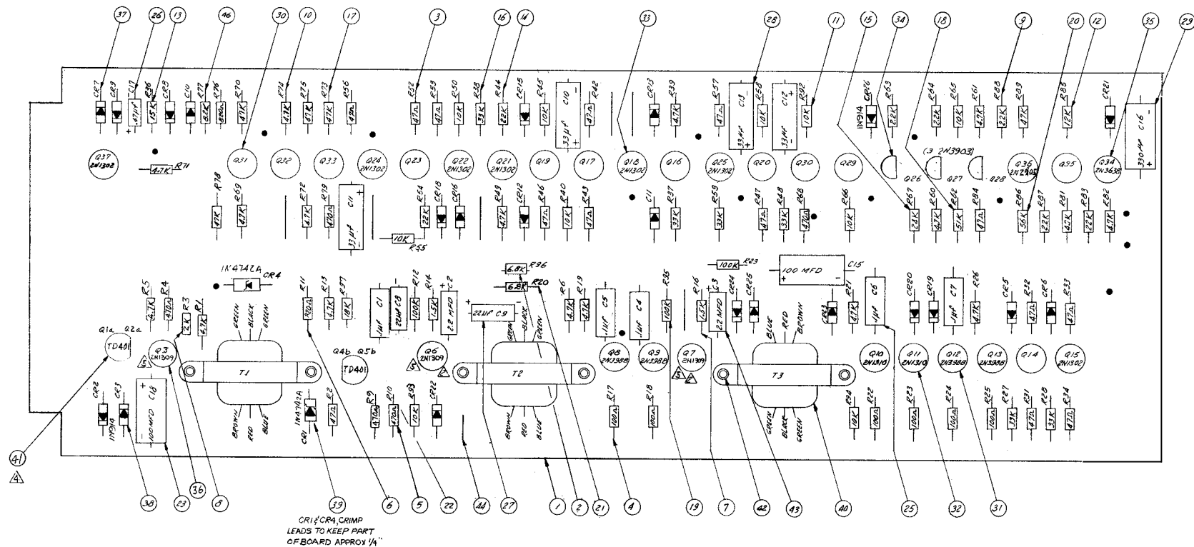
Figure 7-3. Detector Circuits PC Board D0994L
