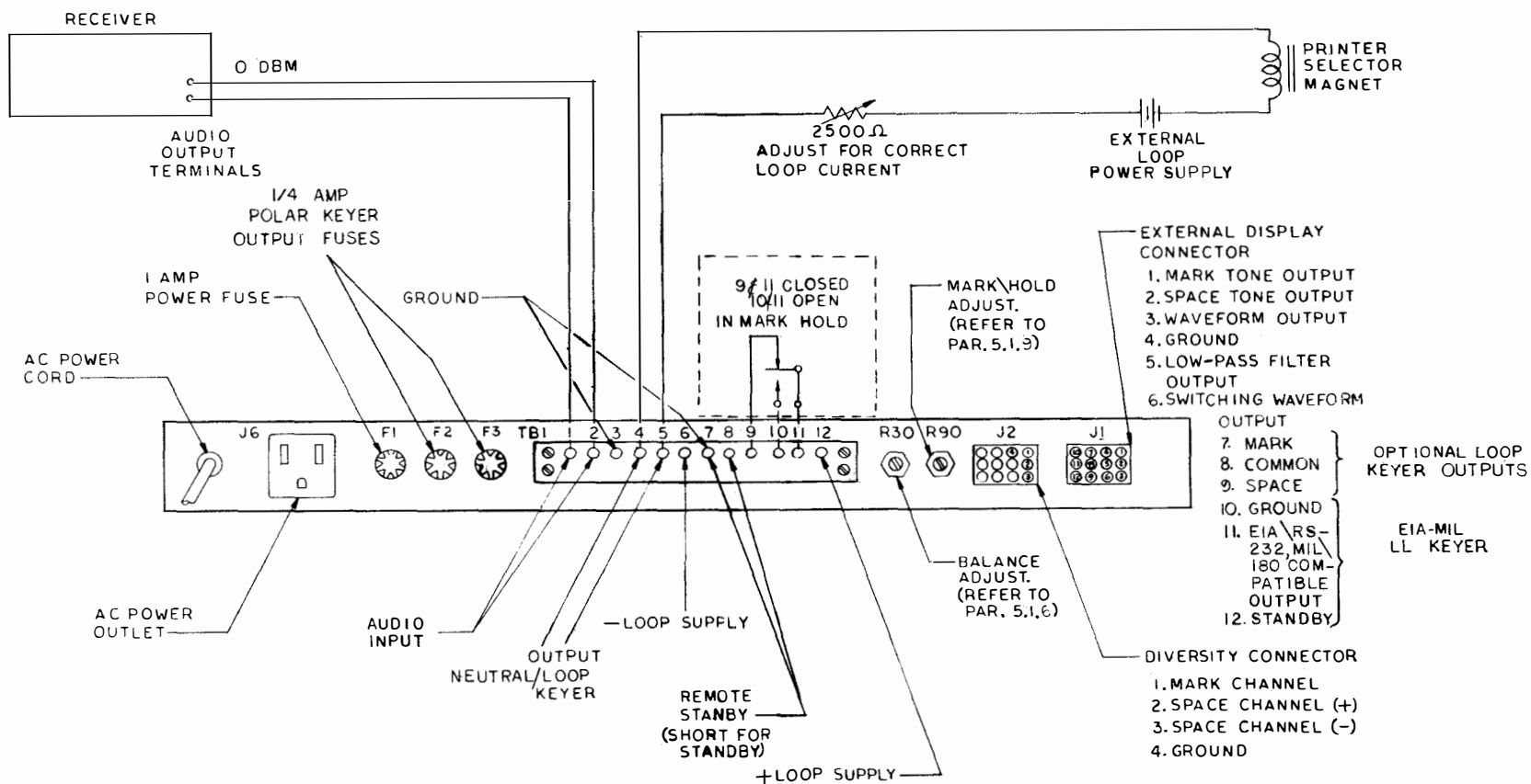
Figure 2-1. Typical Demodulator Installation C1100C
