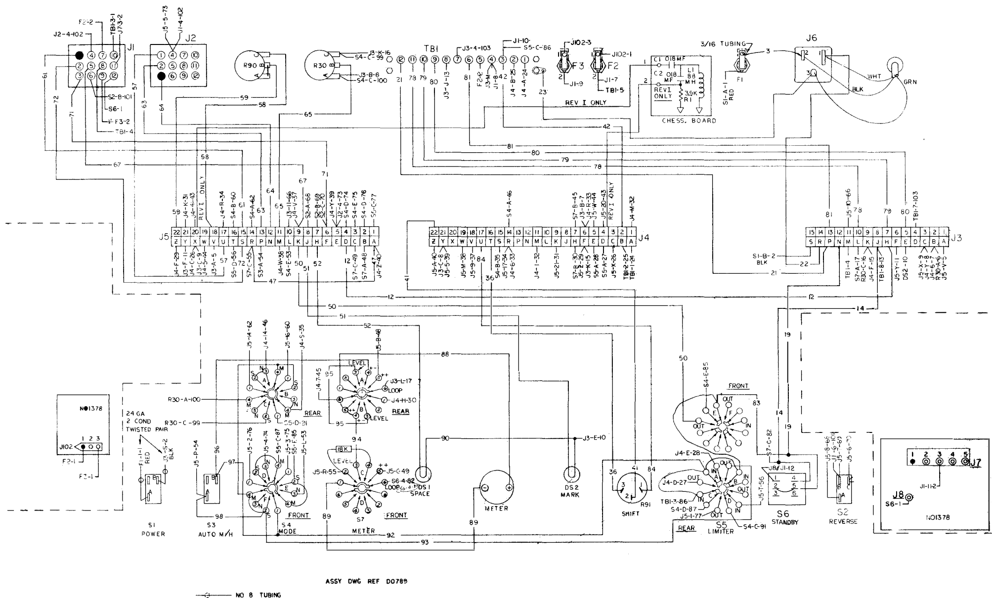
Figure 6-4. Model 1203 Wiring Diagram D07900, Sheet 5
