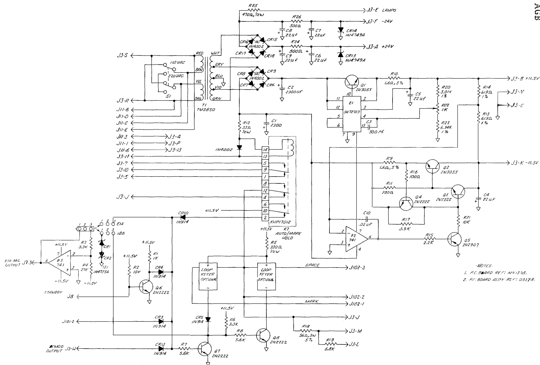
Figure 6-3. Power Supply Schematic Diagram D3446B
