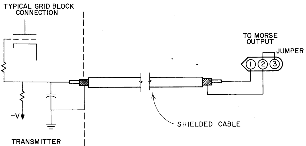
Figure 2.2 Typical Connection for Grid Block Keying
