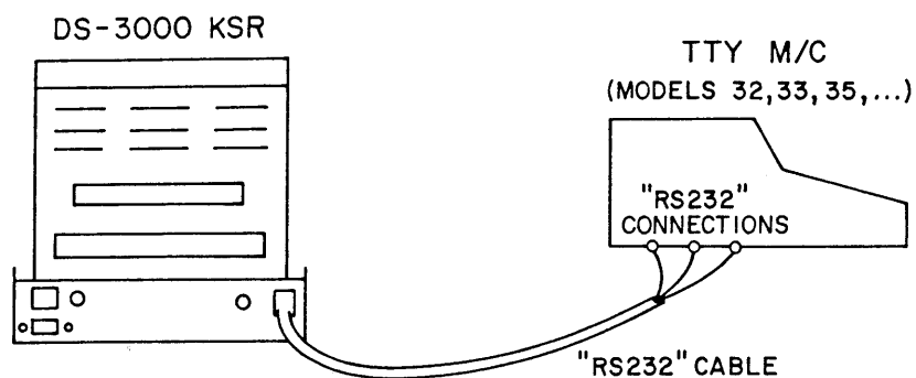
(a) Typical RS-232C connections to a TTY machine
