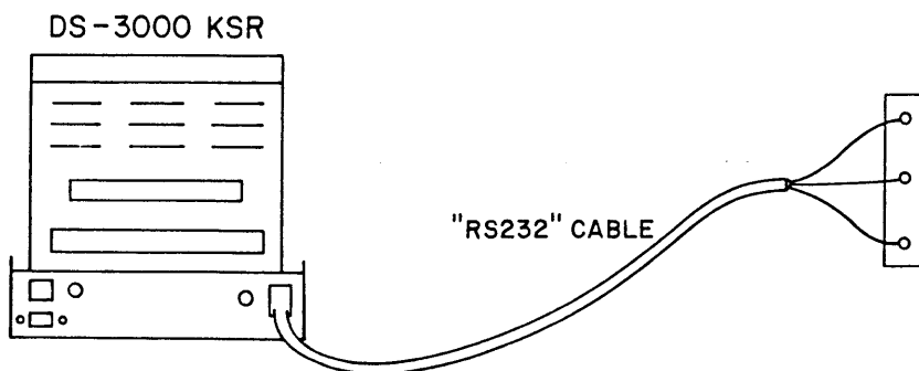
(c) General connections to EIA - RS-232C circuits
