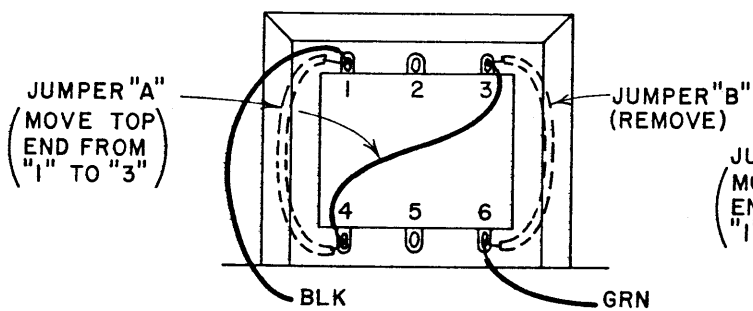
(a) 220 - 250 VAC Connection
