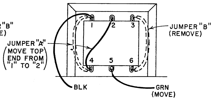
(b) 190 - 220 VAC Connection
