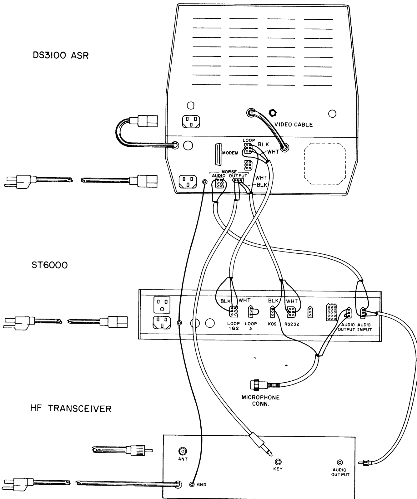
FIGURE 16. SYSTEM CABLE - PICTORIAL
