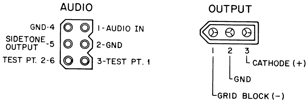
FIGURE 11. DS3100 ASR REAR PANEL CONNECTORS
