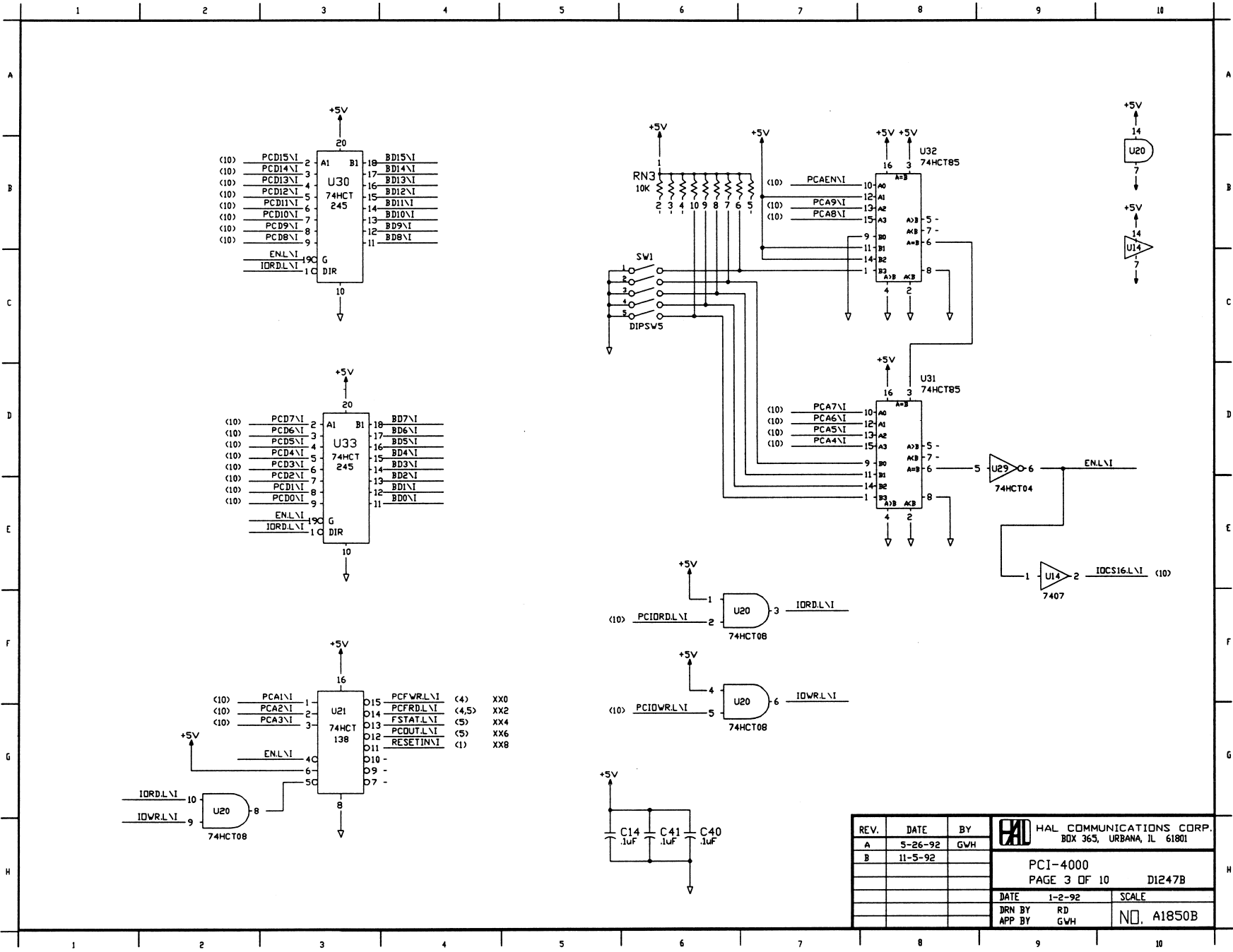
Figure 4.4 PC Bus Interface, I/O Address
