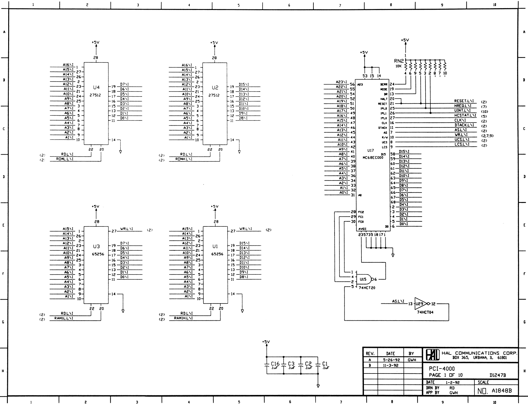
Figure 4.2 Control Processor, RAM, ROM
