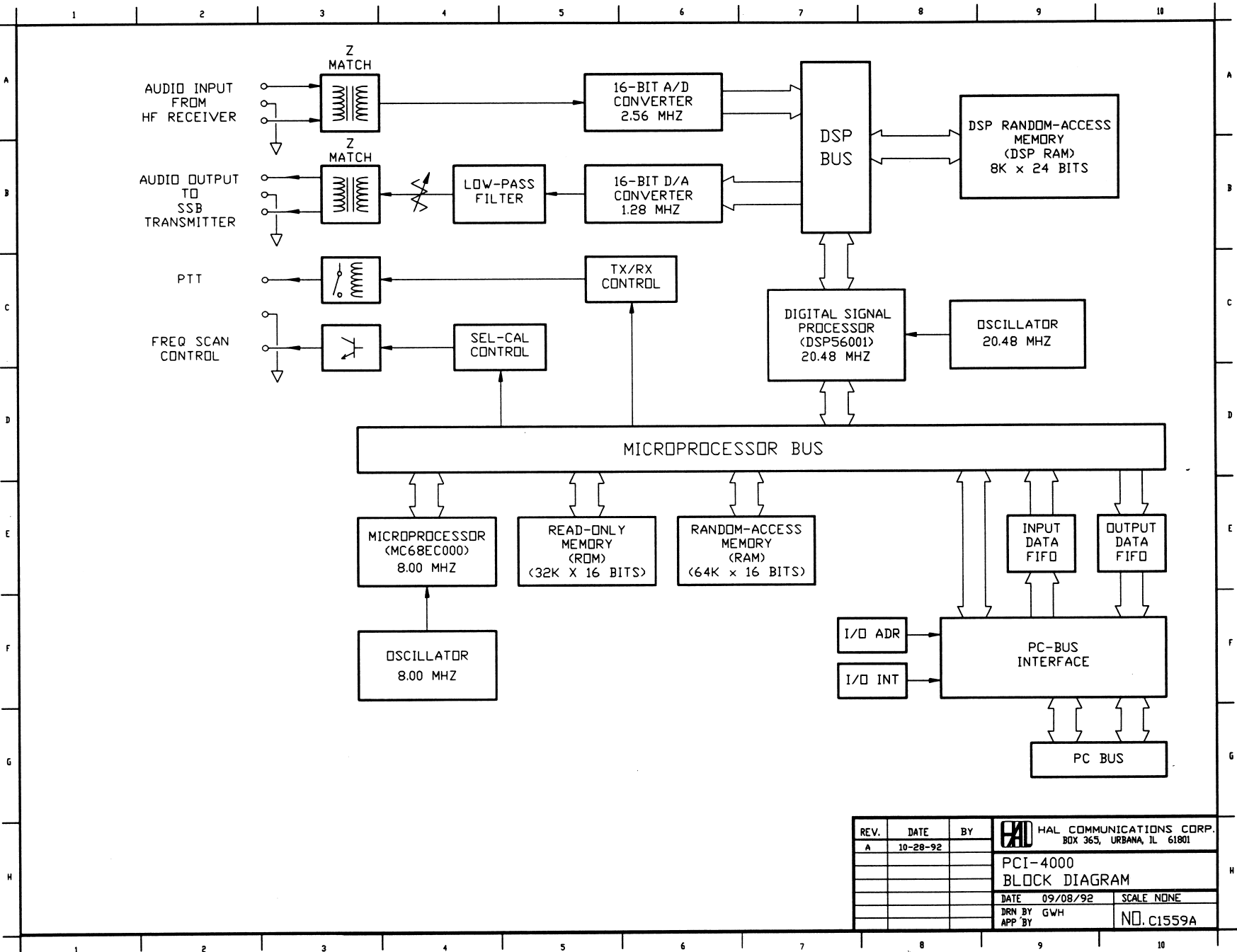
Figure 4.1 PCI-4000 Block Diagram
