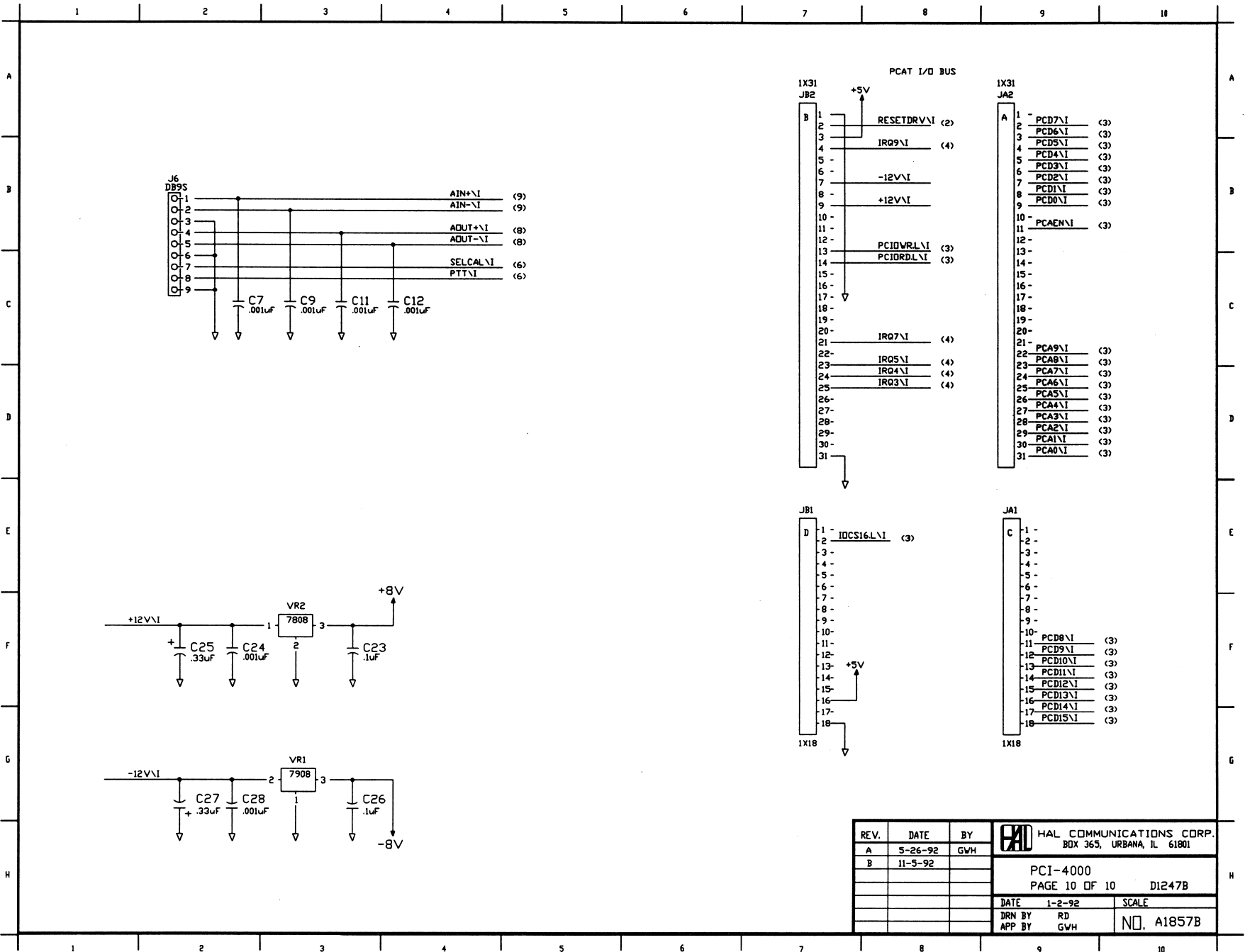
Figure 4.11 I/O Connections, Voltage Regulators
