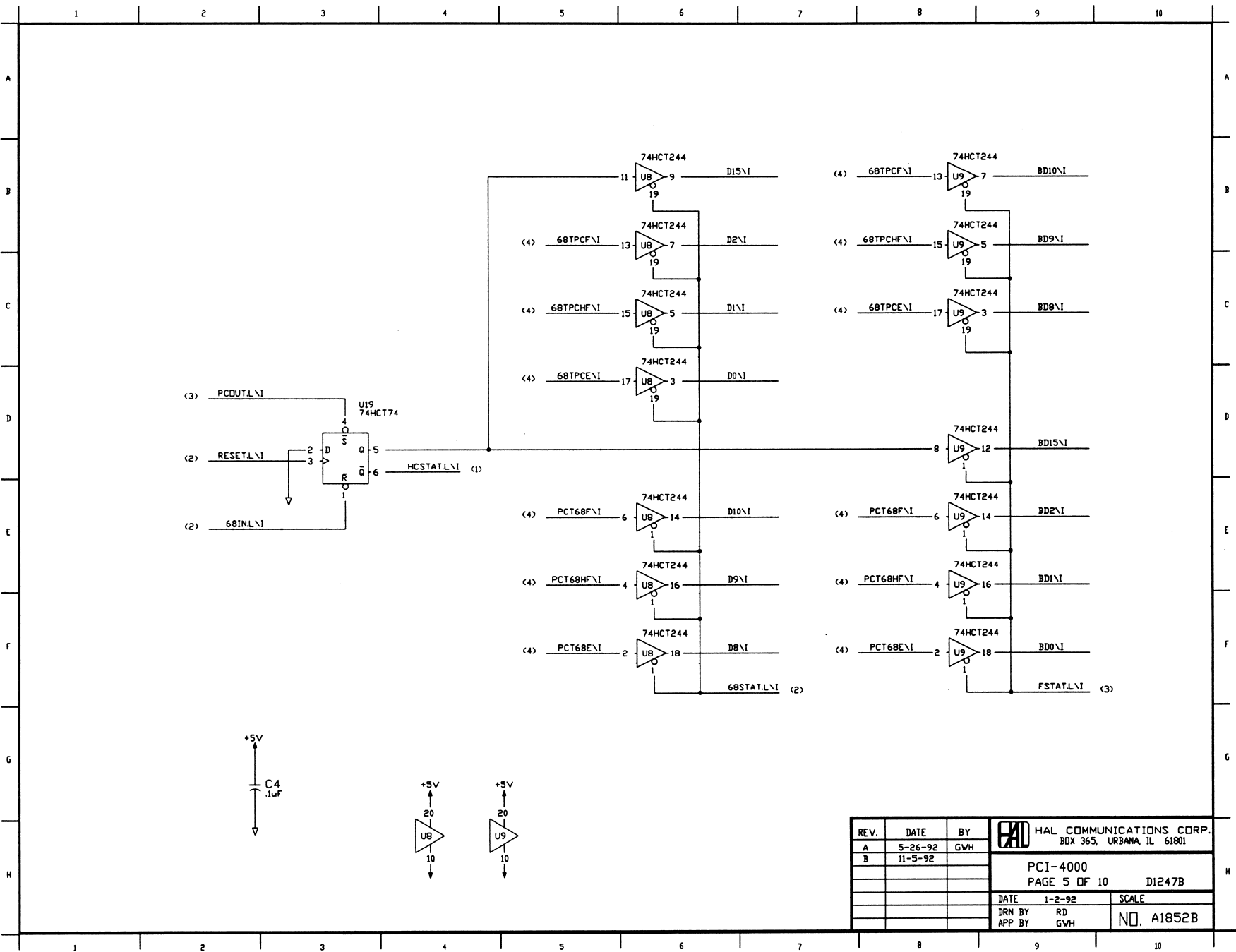
Figure 4.6 68000 Bus Interface
