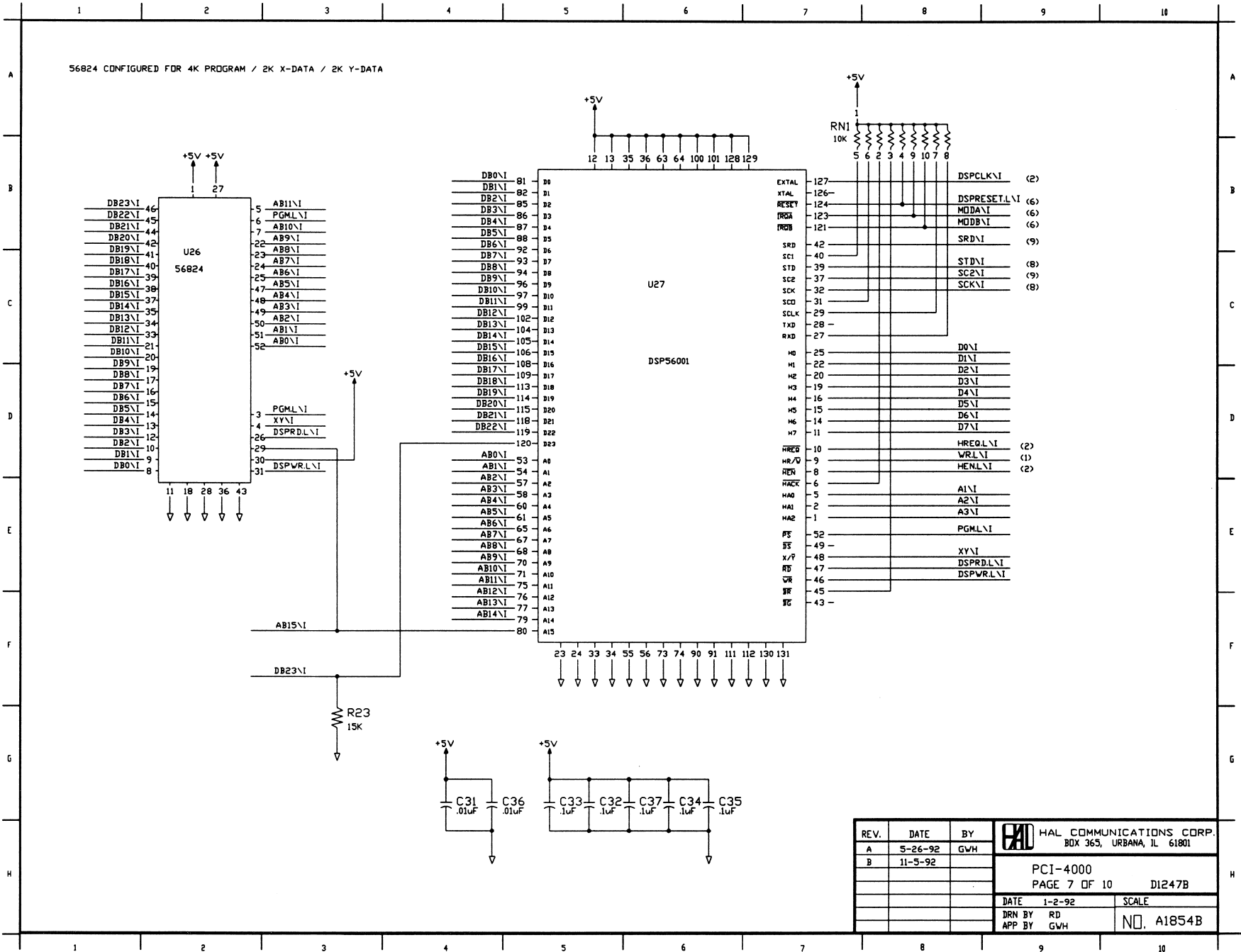
Figure 4.8 Digital Signal Processor, DSP RAM
