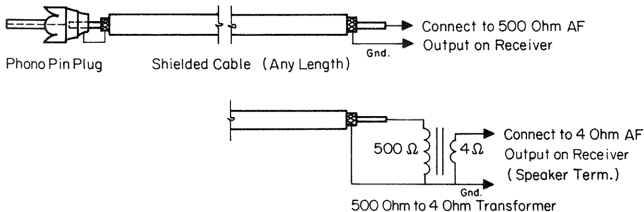
Connections to Audio Input of Demodulator
