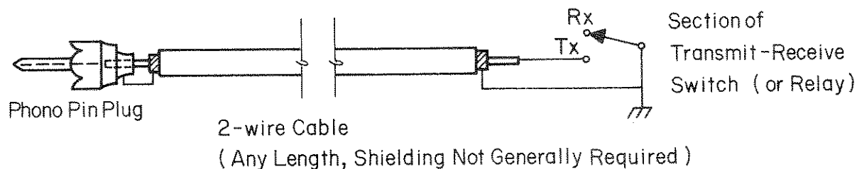
Connections to Remote Jack
