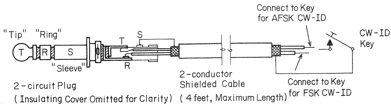
Connections to CW-ID Key Jack
