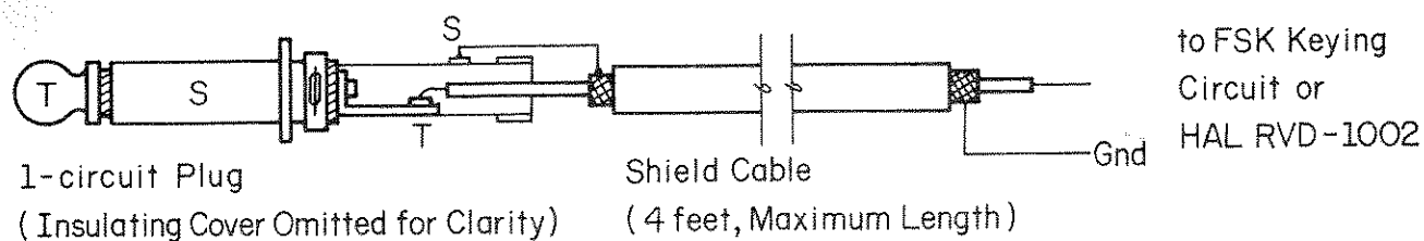
Connections to FSK Jack
