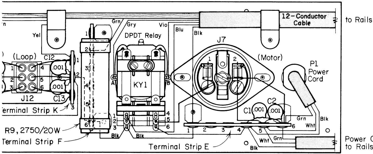
Ground Connection Detail for Terminal Strip E
