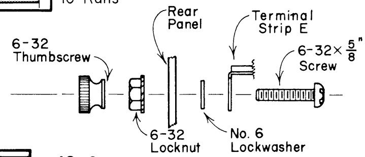
Ground Connection Detail for Terminal Strip E
