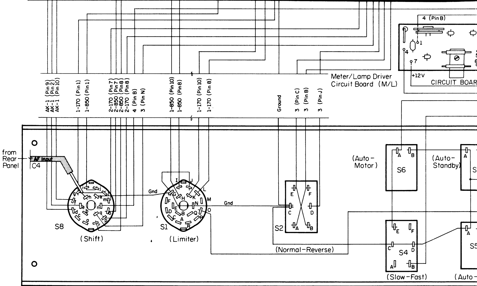
Front Panel (as Viewed from Inside)
