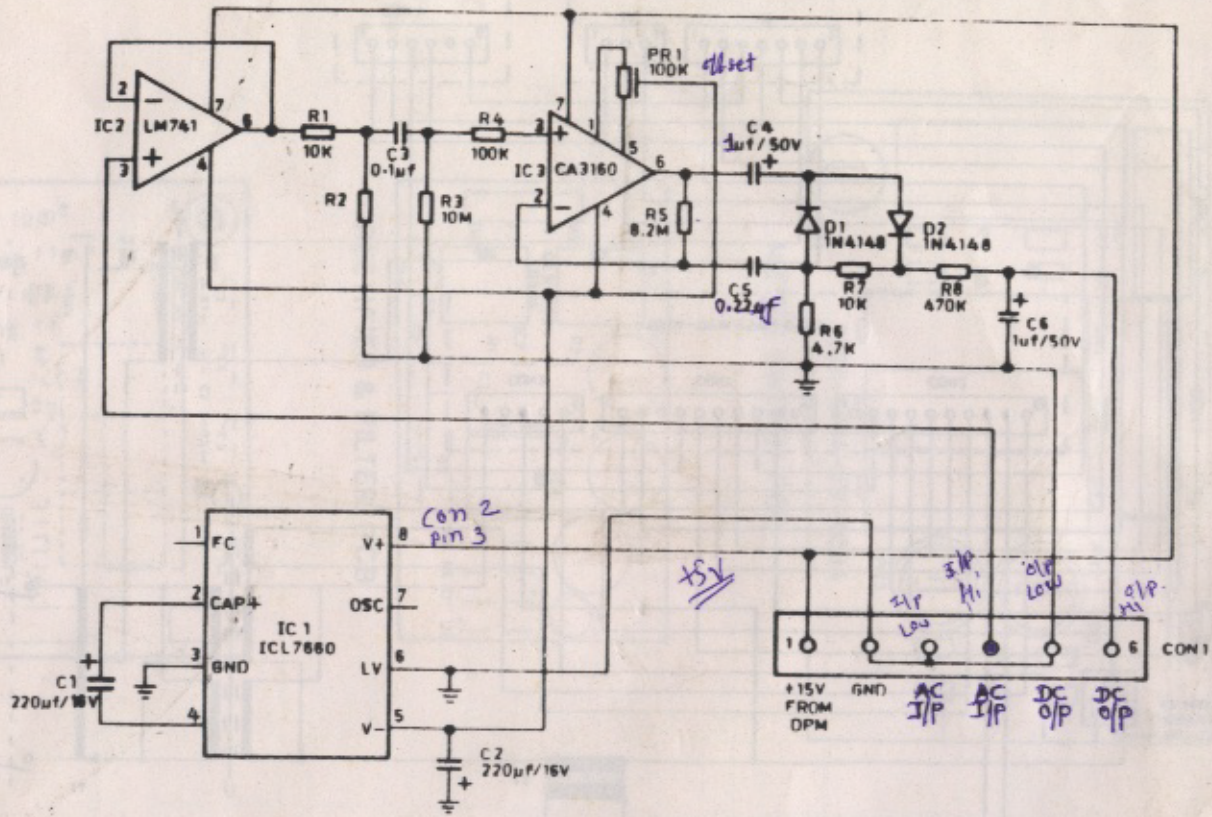
RECTIFIER & FILTER CIRCUIT SCHEMATIC (PCB. REF: GLB-1504-0694)
