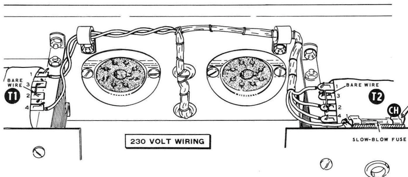
Detail 10B
