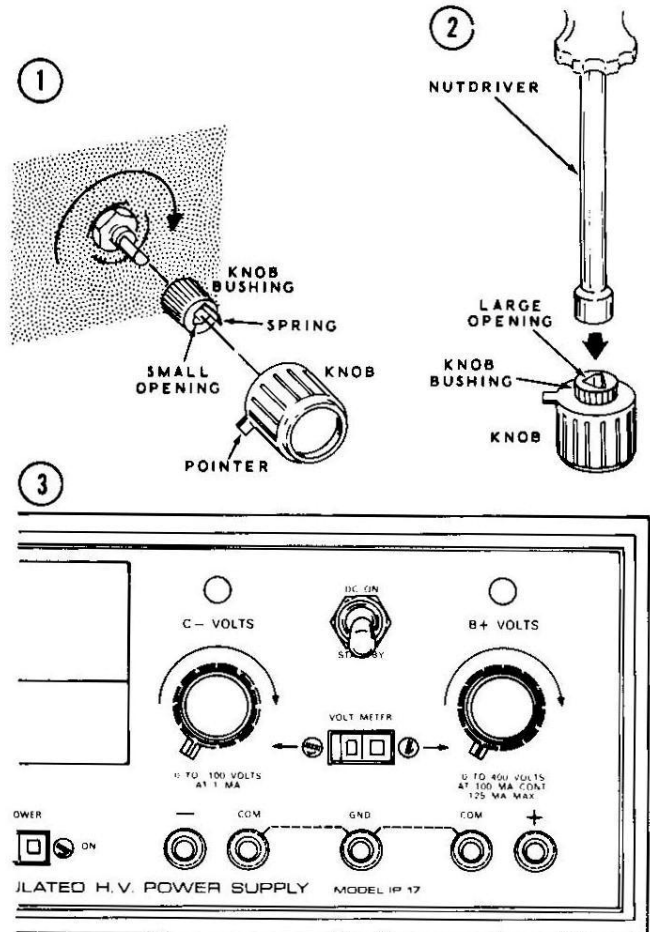
Detail 12B
