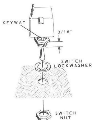
Detail 3F
