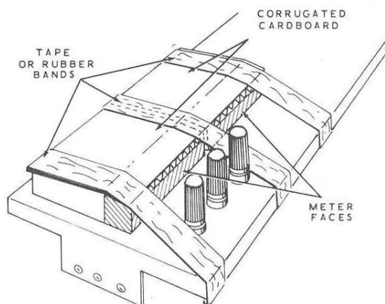
Detail 3J
