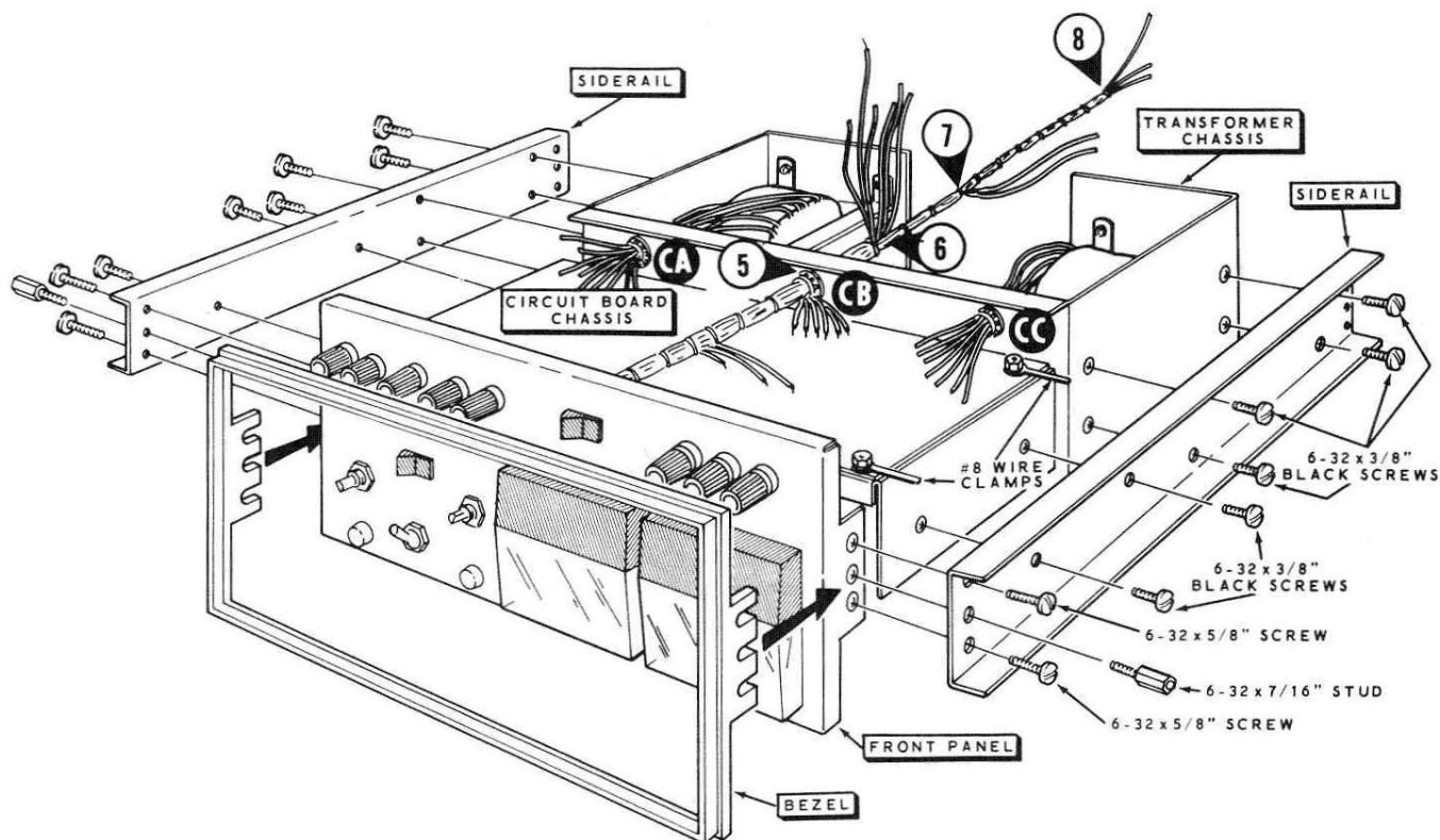
PICTORIAL 8
