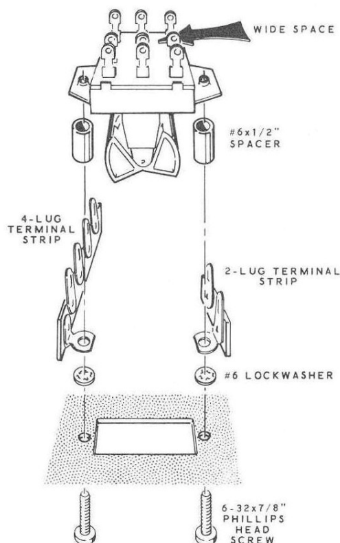
Detail 3D
