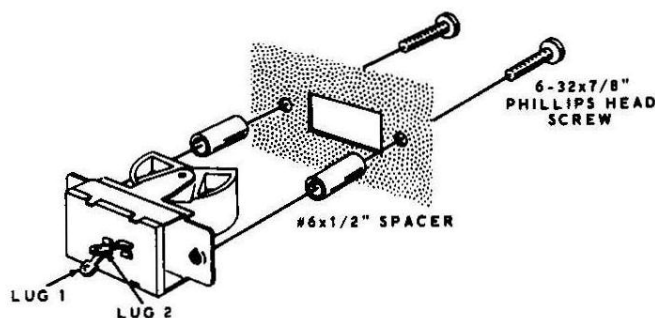
Detail 3B
