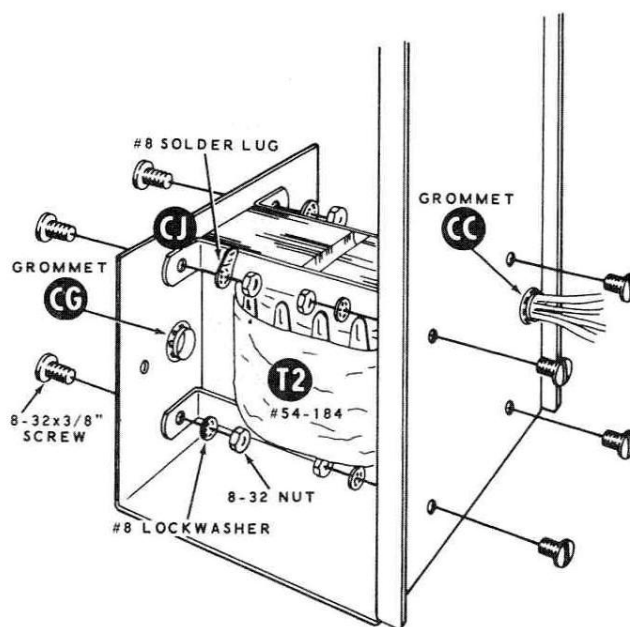
Detail 7C
