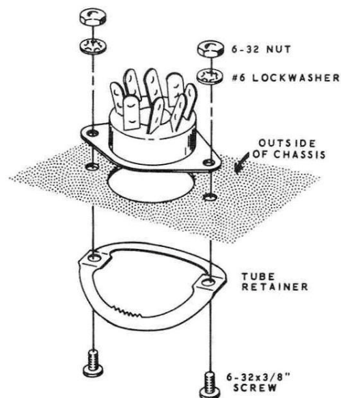
Detail 7B
