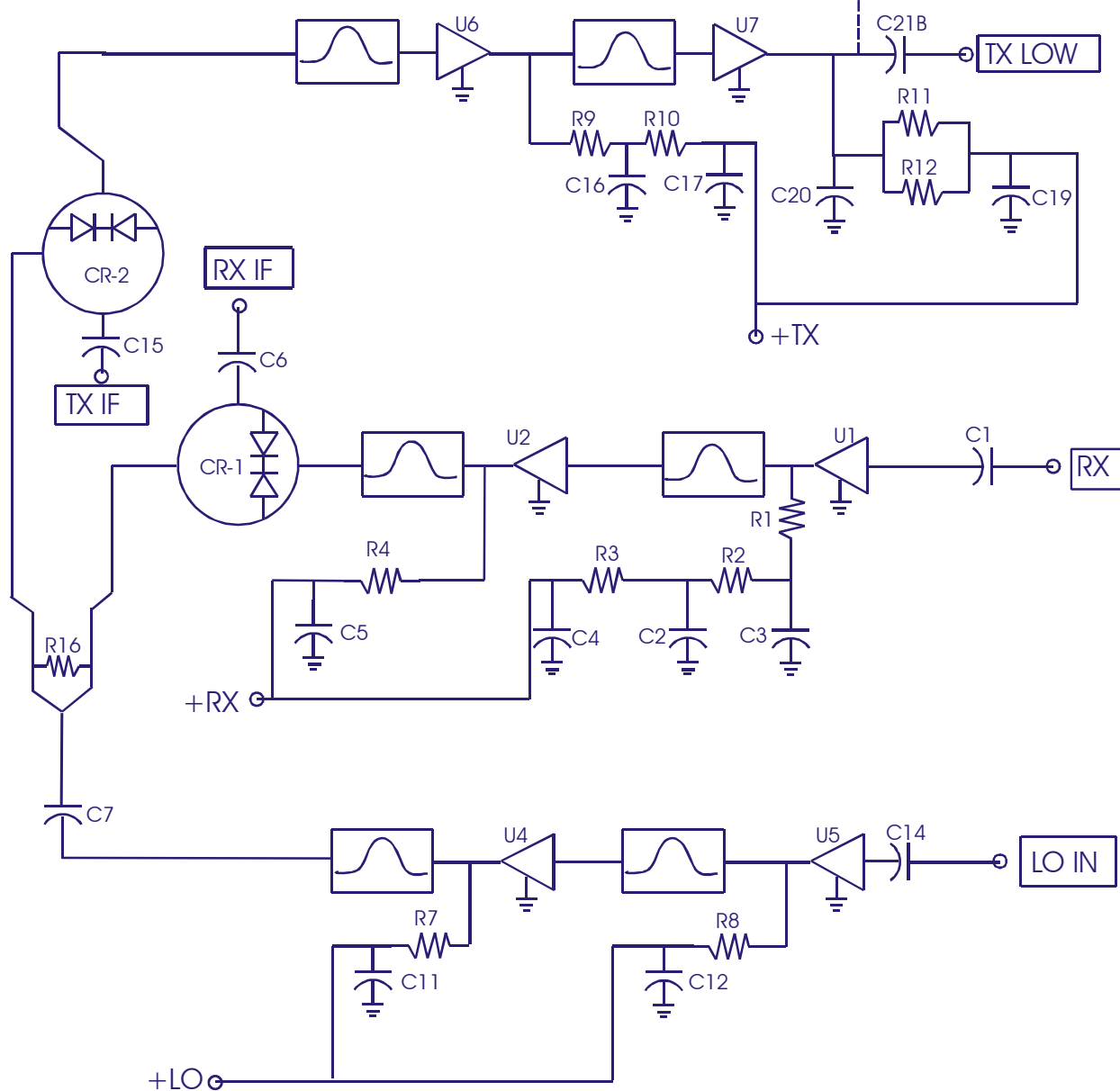
2304-144 TRANSVERTER SCHEMATIC
