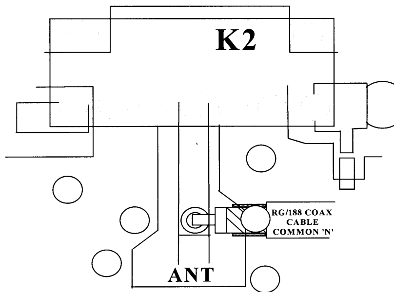
Figure 7 Coaxial Cable mounting on PCB shaded areas are solder points
