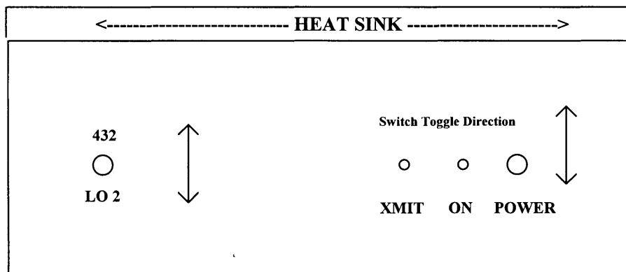
Figure 5 Switch / LED Mounting Positions
