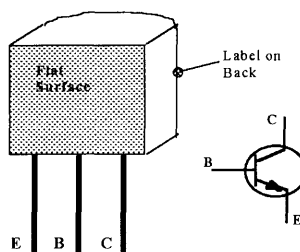
MPS5179 Transistor
