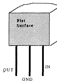
78L09 Regulator
