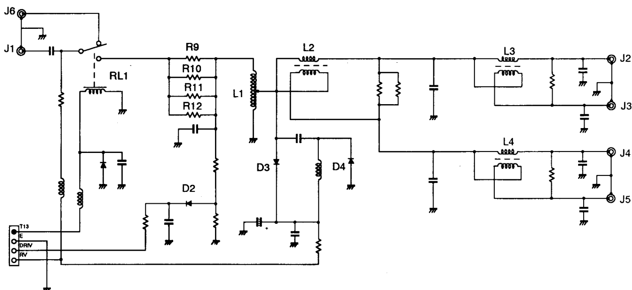
Power splitter circuit
