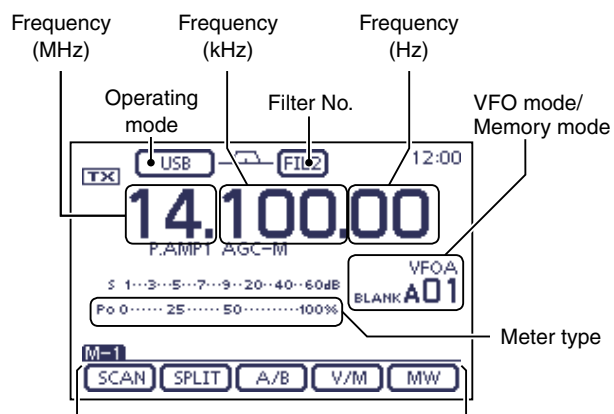
Touch key for each function. (Example: M-1 menu is selected.)
