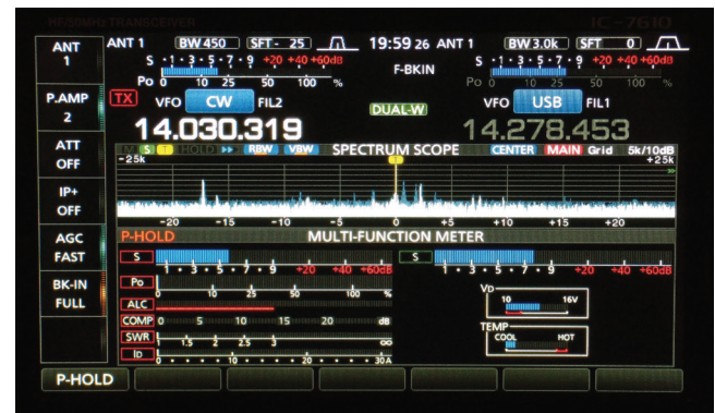
Figure 4 — A more compact bar graph of a selected meter at the top of the display allows more room for the spectrum display, or all meter choices can be viewed simultaneously, as shown here.
