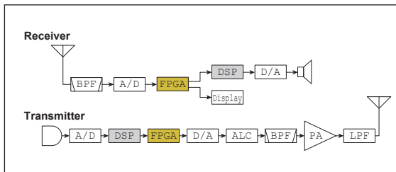
Figure 02-2. Block diagram of the IC-7760
