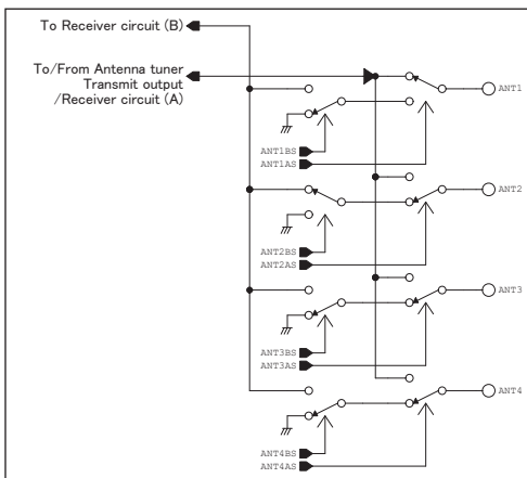
Figure 06-4. Block diagram of the antenna switching circuit
