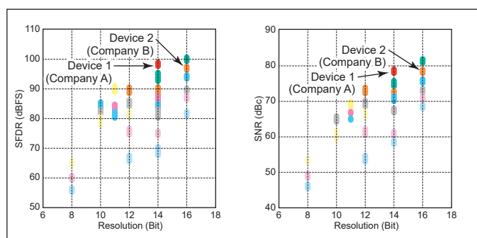
Figure 04-23. Comparison chart between SFDR and SNR
