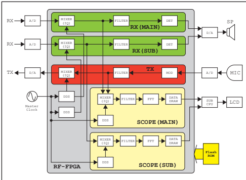
Figure 06-20. Scope block diagram for the IC-7760
