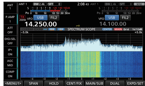
Figure 05-30. Scope with a pseudo audio spectrum (DPD function = OFF)
