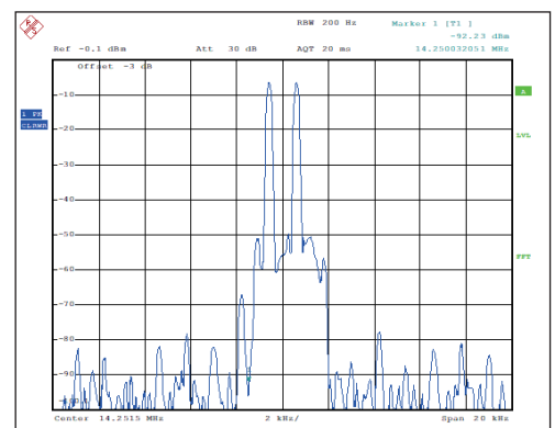
Figure 05-27. Transmit IMD characteristics when DPD is activated
