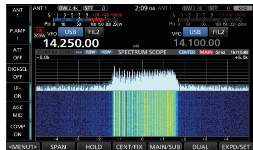
Figure 05-31. Scope with a pseudo audio spectrum (DPD function = ON)
