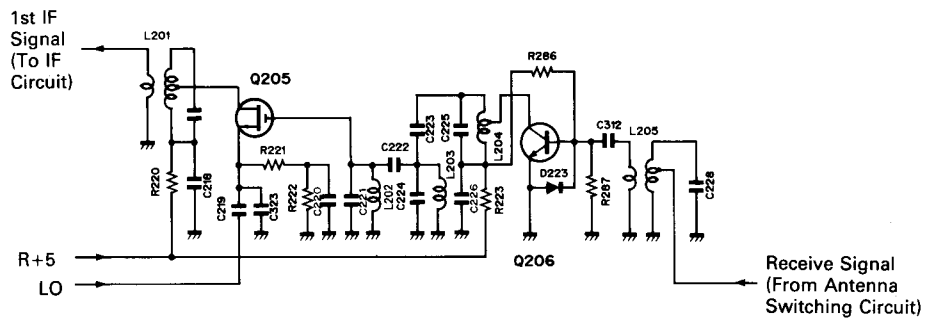
Fig. 4-1 RF Circuit
