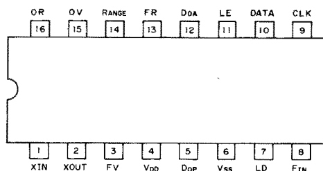
PLL2001 IC3 (PLL IC)
