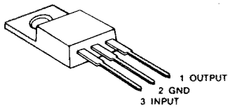
AN6541 IC3 (3-TERMINAL POSITIVE VOLTAGE REGULATOR)
