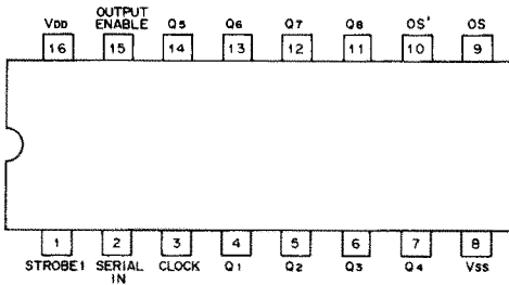
μPD4094BC (IC-228A: U.S.A., Asia) IC5 (8-STAGE SHIFT REGISTER)
