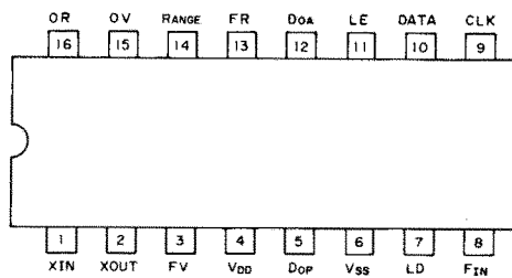
PLL2001 IC3 (PLL IC)
