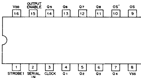
μPD4094BC IC5 (8-STAGE SHIFT REGISTER)
