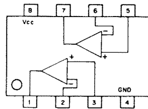
NJM4558D IC4 (DUAL NOISE LOW AMP)
