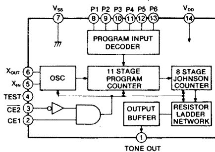
S7116A (IC-228H: U.S.A., Asia) IC6 (PROGRAMMABLE TONE GENERATOR)
