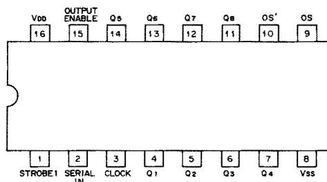
μPD4094BC (IC-228H: U.S.A., Asia) IC5 (8-STAGE SHIFT REGISTER)
