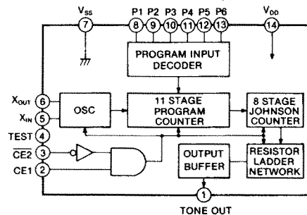
S7116A (IC-228A: U.S.A., Asia) IC6 (PROGRAMMABLE TONE GENERATOR)
