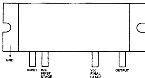
SC-1022 IC1 (45W VHF RF POWER AMP)
