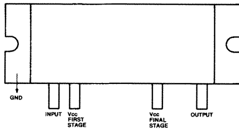
SC-1019 IC1 (25W VHF RF POWER AMP)
