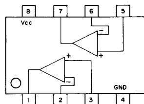
NJM4558M IC9 (LOW NOISE DUAL OPERATIONAL AMPLIFIER)
