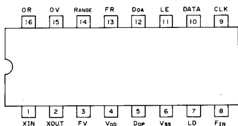
PLL2001S IC6 (PLL SYNTHESIZER)
