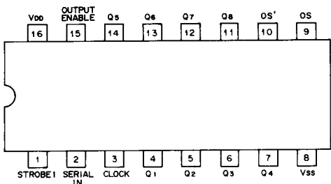
μPD4094BG IC3, IC4 (8-STAGE SHIFT AND STORE BUS)
