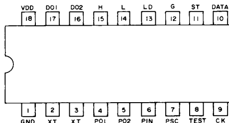
TC9181P IC7 (PROGRAMMABLE DIVIDER)
