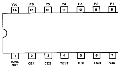
S7116A IC2 (PROGRAMMABLE TONE GENERATOR)
