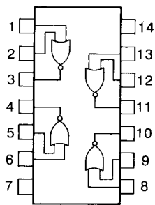
LC4001BM IC203 (QUAD 2 INPUT NOR GATE)
