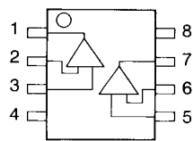
M5218FP IC205 (LOW NOISE DUAL OPERATIONAL AMPLIFIER)
