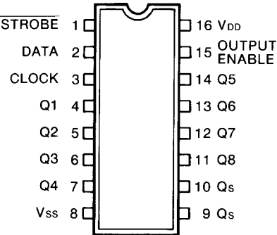
μPD4094BG IC602 (8 STAGE SHIFT/STORE BUS REGISTER)
