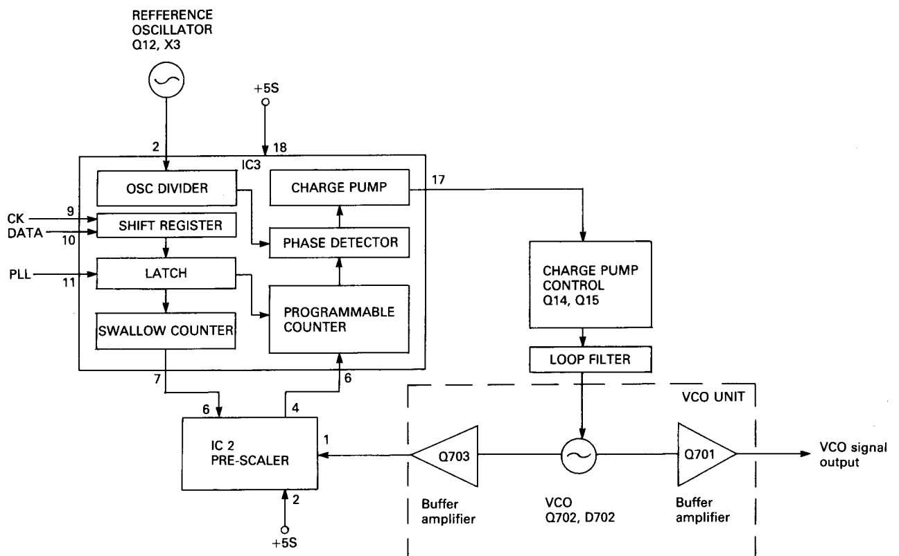
PLL CIRCUIT BLOCK DIAGRAM
