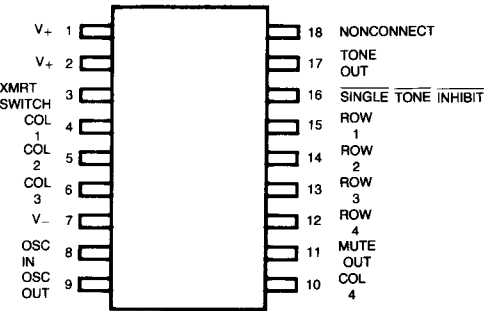
LR40872 IC801 (TONE DIALING)
