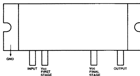
SC-1019 IC4 (UX-29A/E only) SC-1022 IC4 (UX-29H only) (POWER AMPLIFIER)
