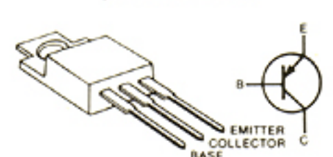
2SB1019 O/Y Q26 (UX-29H only)
