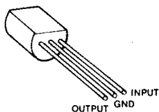
TA78L005AP IC3 (3-TERMINAL 5V REGULATOR)
