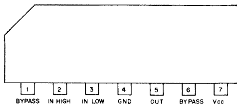
μPC577H IC1 (FM IF AMPLIFIER)
