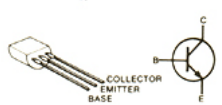
2SC3355 Q4
