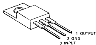
AN6541 IC7 (3-TERMINAL 8V REGULATOR)
