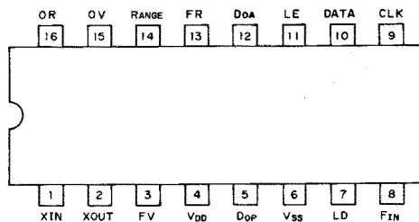
PLL 2001 IC5 (PLL SYNTHESIZER IC)
