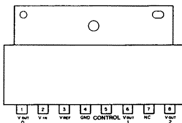
MB3756 IC3 (VOLTAGE REGULATOR)
