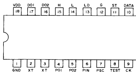
TC9181P IC9 (PROGRAM DIVIDER)
