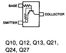
RN1404 (Symbol: XD)
