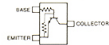
RN1404 (Symbol: XD)
