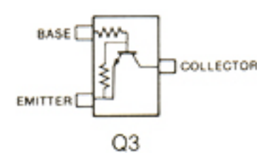
RN1409 (Symbol: XJ)
