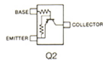
RN2404 (Symbol: YD)
