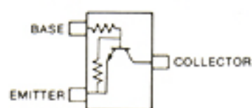
RN1402 (Symbol: XB)
