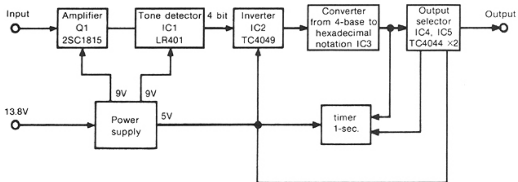
Block diagram
