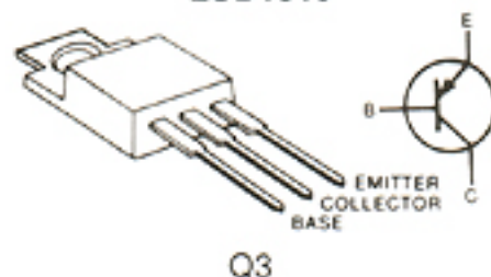
2SB1019
