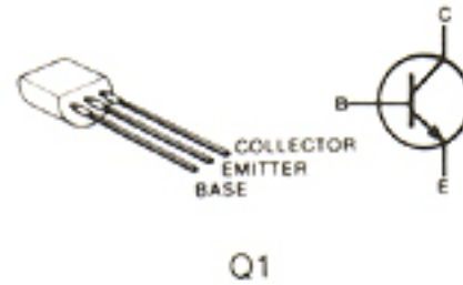
2SC2407 (A)
