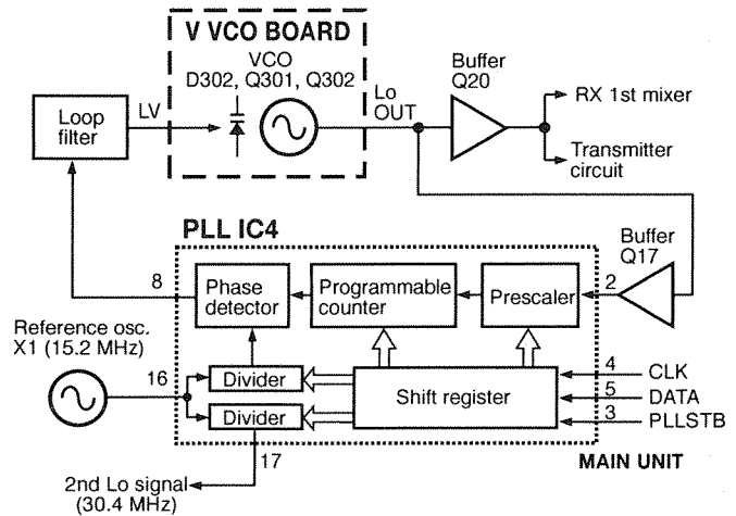
Fig. 4 PLL CIRCUIT
