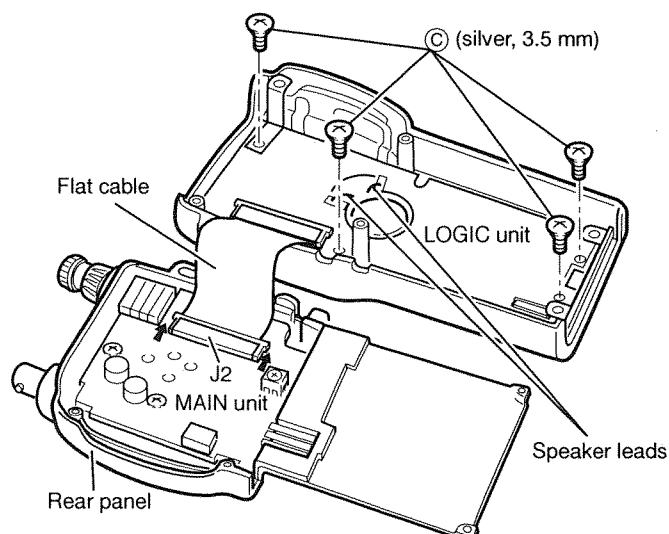
Fig. 2 Removing the LOGIC unit
