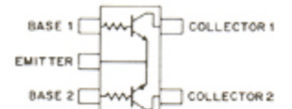
XP1210 (Symbol: AC)
