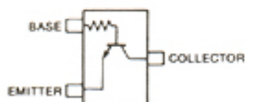
UN9210 (Symbol: 8L)
