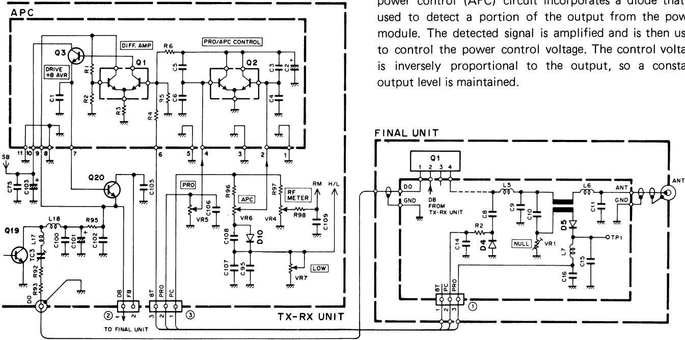
Fig. 3 APC and SWR protection circuits
