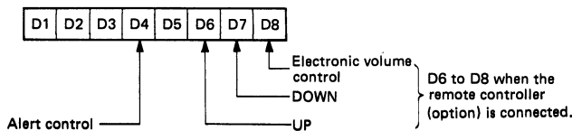
Fig. 14 Data configuration for alert and electronic volume control
