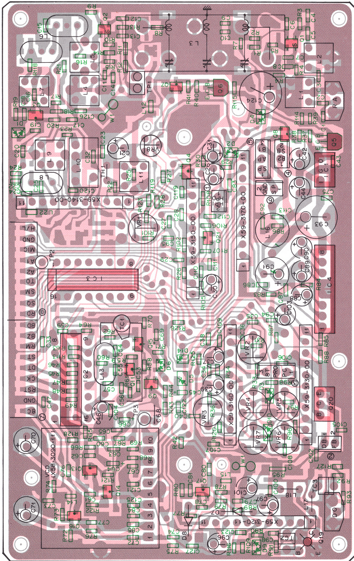
TX-RX UNIT (X57-3170-10) Foil side view
