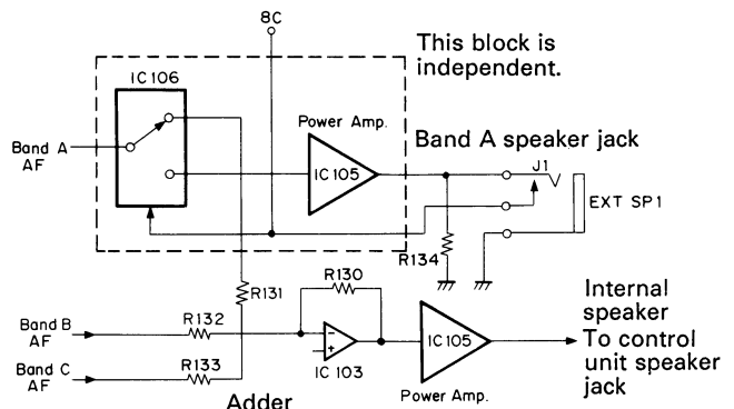
Fig. 28 Speaker Selection Circuit
