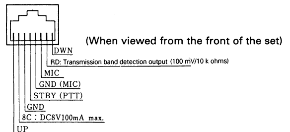
Fig. 32 Microphone Socket (on Front Panel)
