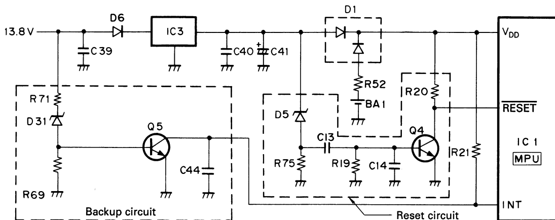
Fig. 16 Reset and Backup Circuits
