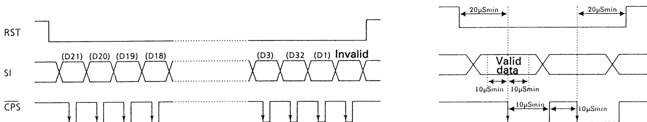
Fig. 23 M56760 PLL DATA OUTPUT
