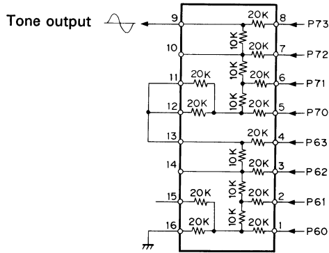
Fig. 17 Internal Configuration of Ladder Resistor (KRR-C001)
