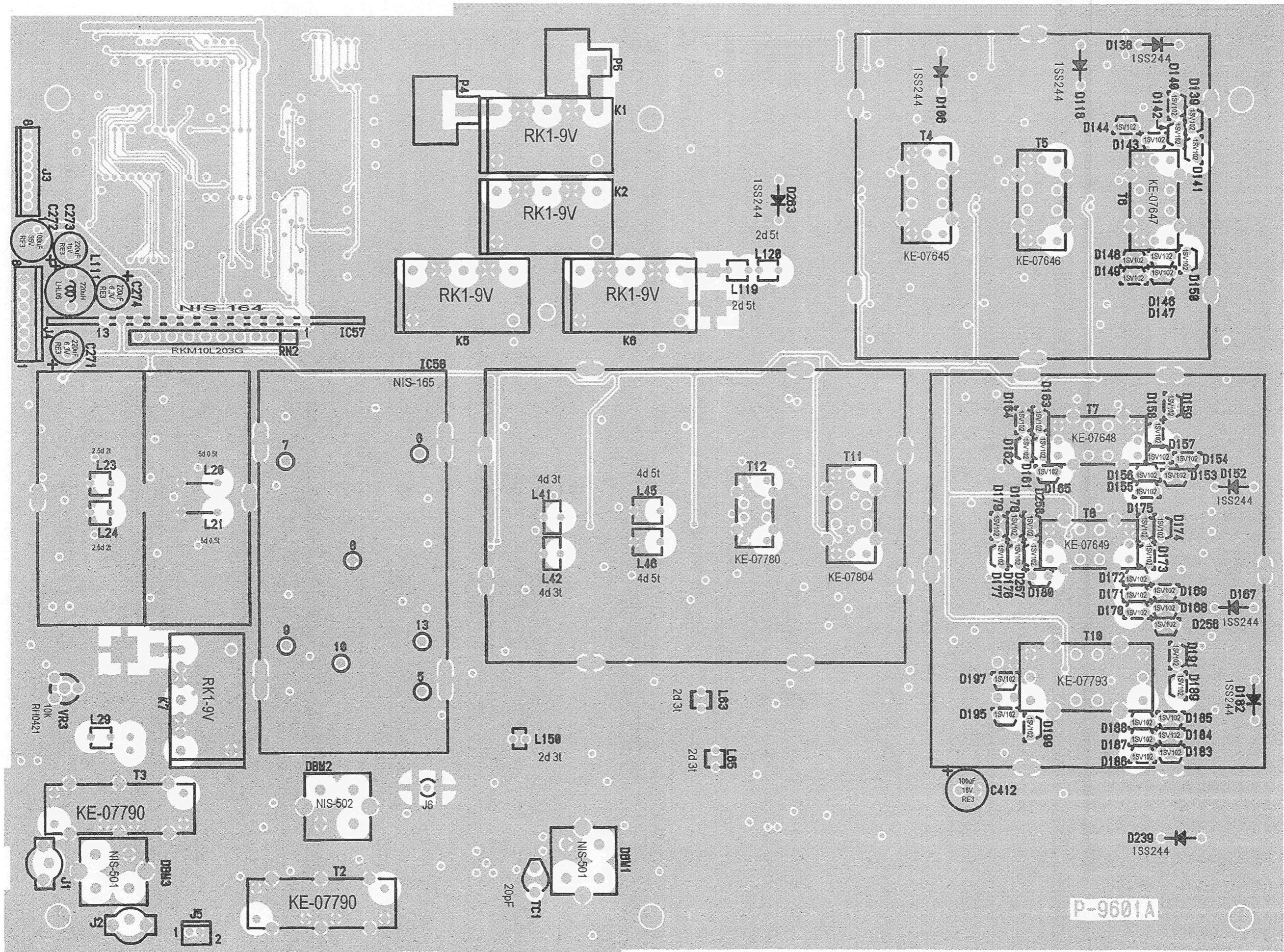
AR5K FRONT UNIT COMPONENT SIDE
