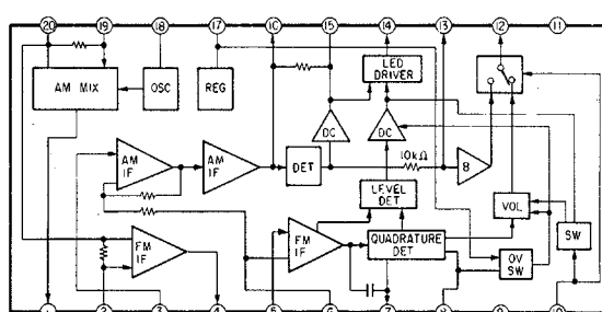
IC2 TA7758P
