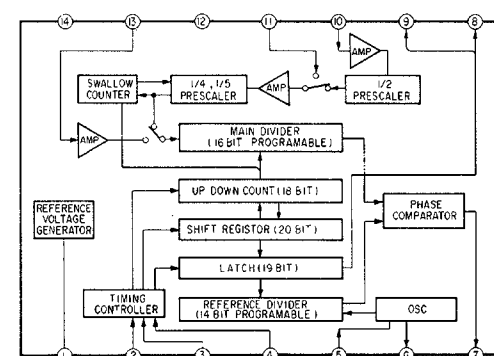
IC202 CXD1118M
