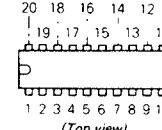
TA7758P
