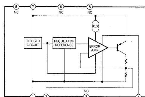
IC203 LA5003M
