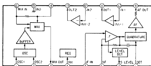
IC1 TA7761F
