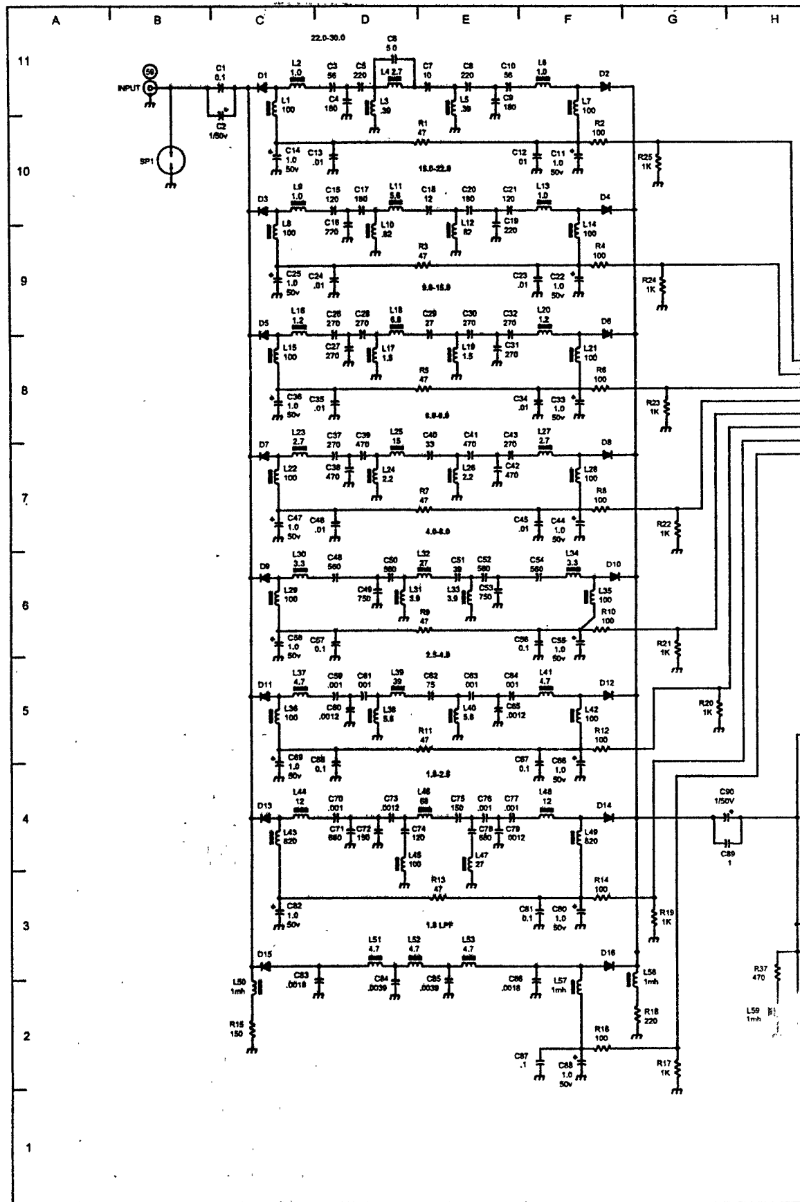
FIGURE 9-6. 81727 RX PRESEL
