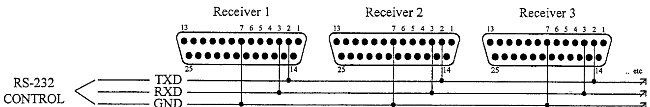
FIGURE 4-1 CONNECTION DIAGRAM
