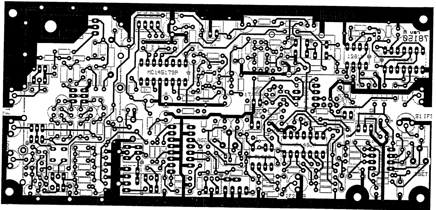
FIGURE 9-11. 81817 BOTTOM CIRCUIT TRACE
