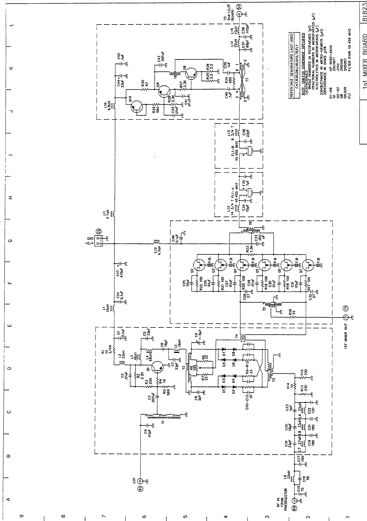
FIGURE 9-9. 81823 1st MIXER SCHEMATIC
