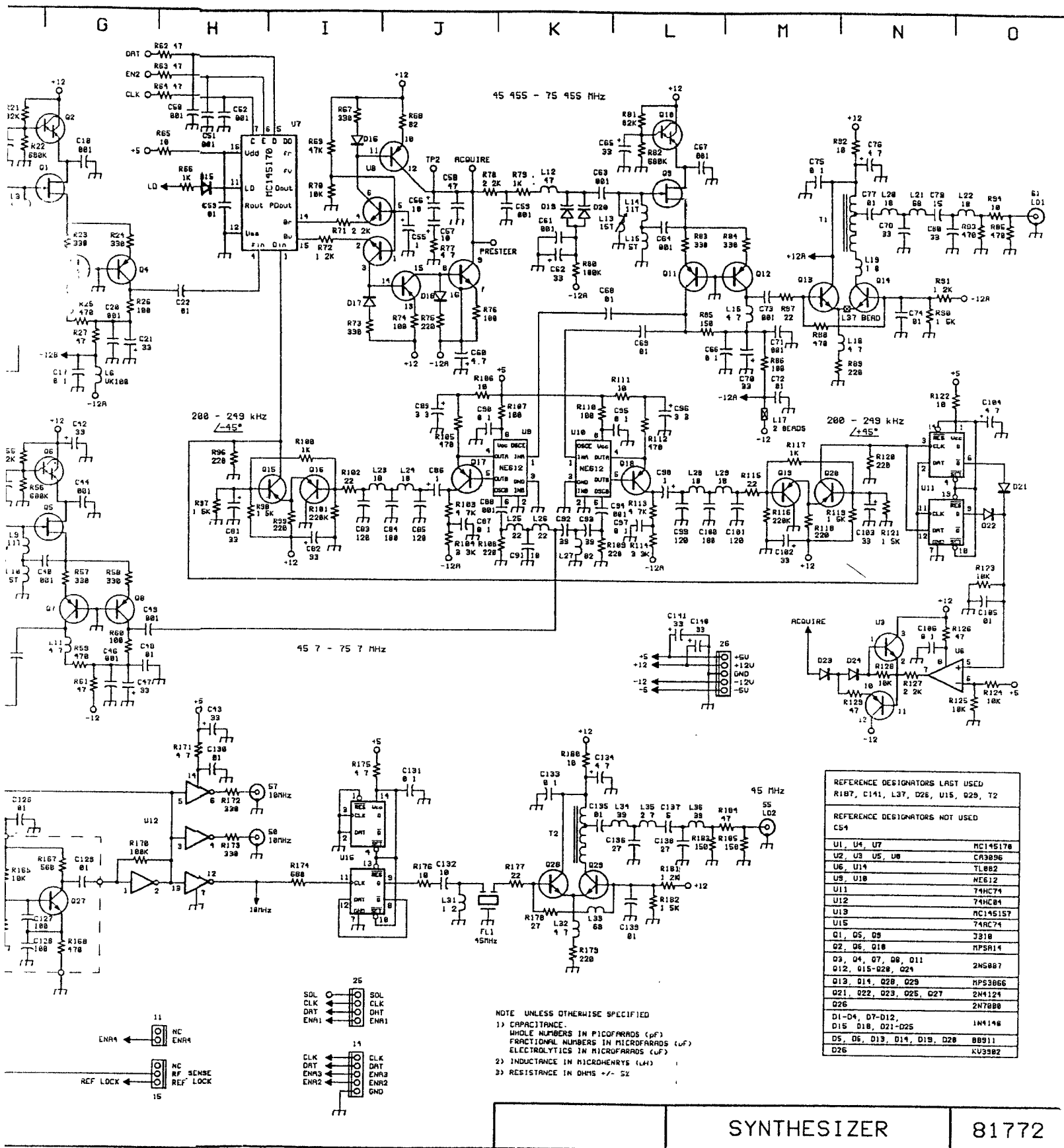
FIGURE 9-21 81772 SYNTHESIZER SCHEMATIC
