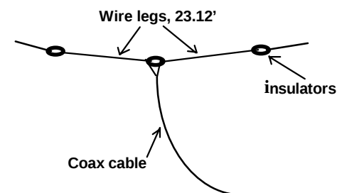
30-meter dipole
