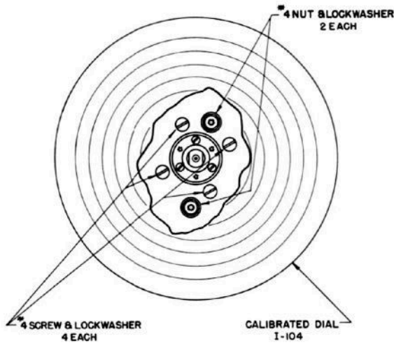
Figure 7-14. RF Signal Generator SG-45A/URM-26, Tuning Capacitor Mounting
