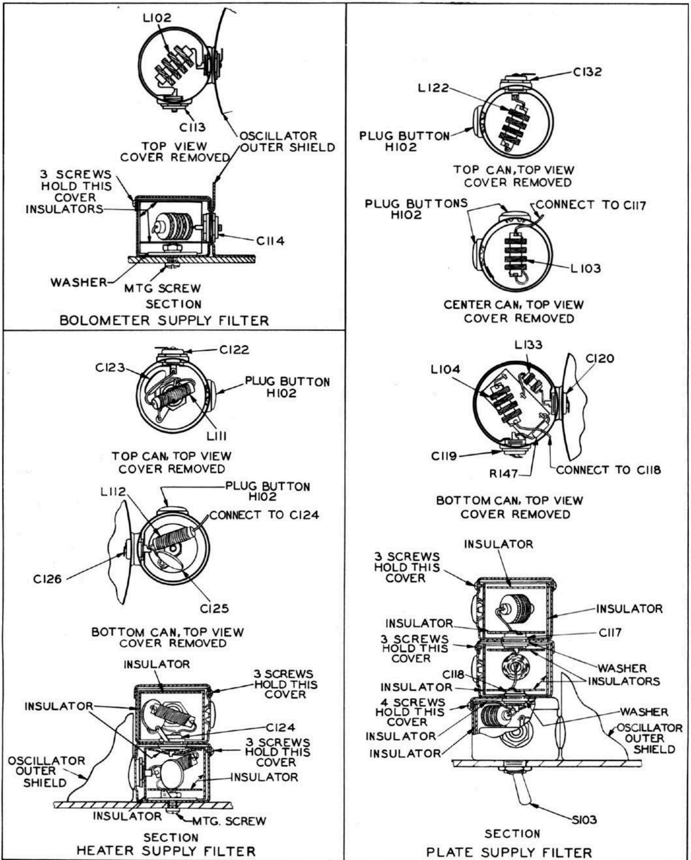
Figure 7-17. RF Signal Generator SG-45A/URM-26, RF Filters
