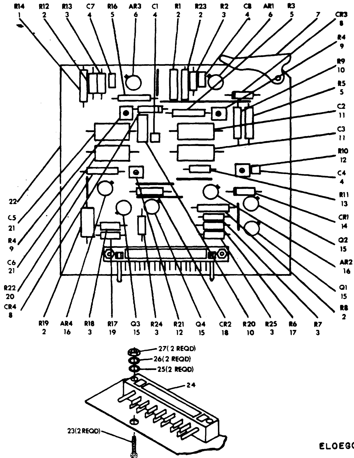
Figure 20. Circuit Card Assembly (A11).
