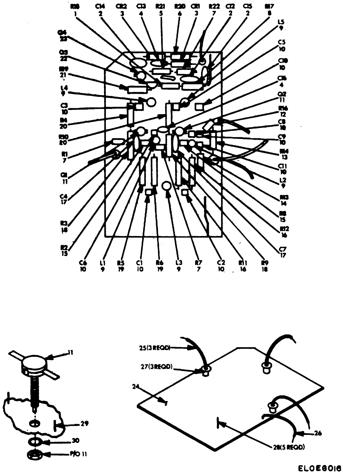
Figure 16. Circuit Card Assembly (A9A2).
