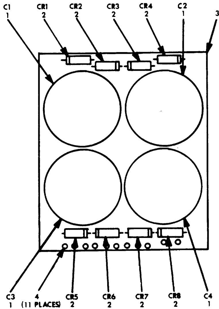
DETAIL FOR ITEM 1(4 PLACES)
