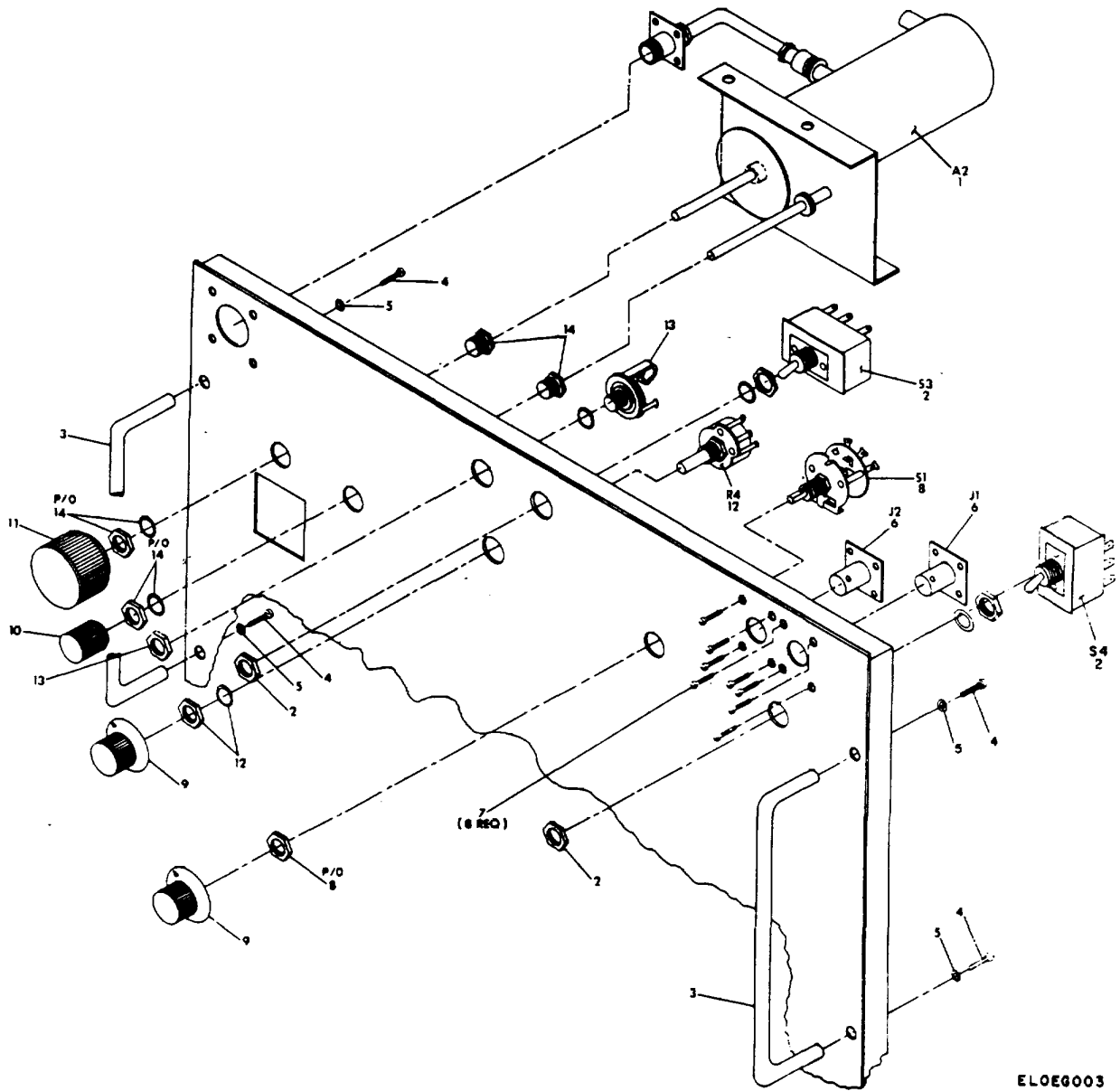
Figure 3. Front Chassis Assembly. 21
