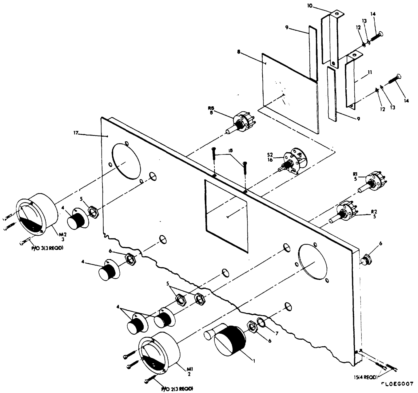
Figure 7. Panel Assembly Front (Top).
