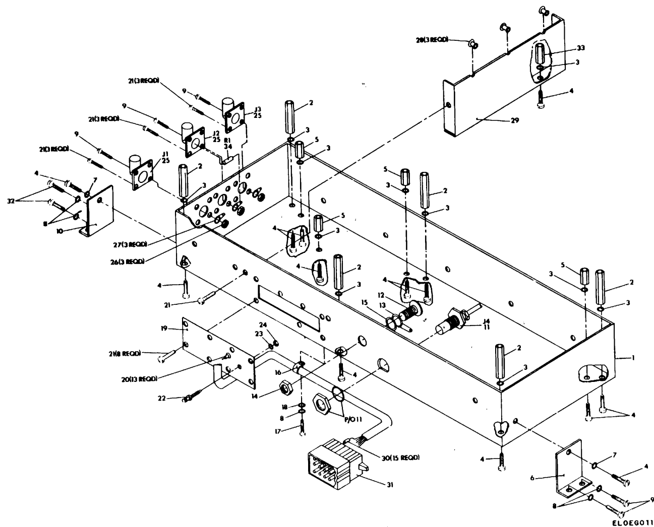
Figure 11. Box Assembly (P/O A9).
