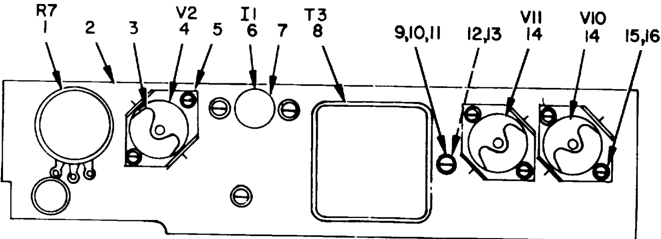
BOTTOM VIEW
