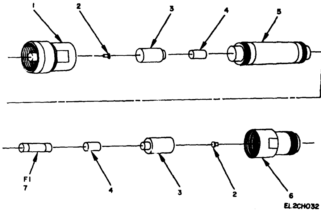
Figure 27. Fuseholder MX-1730/U.
