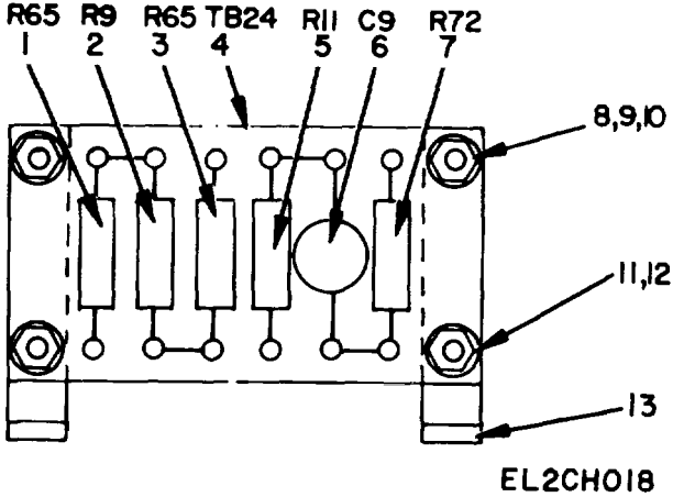
Figure 13. Terminal Board Assembly 608D-75R-2-PM.
