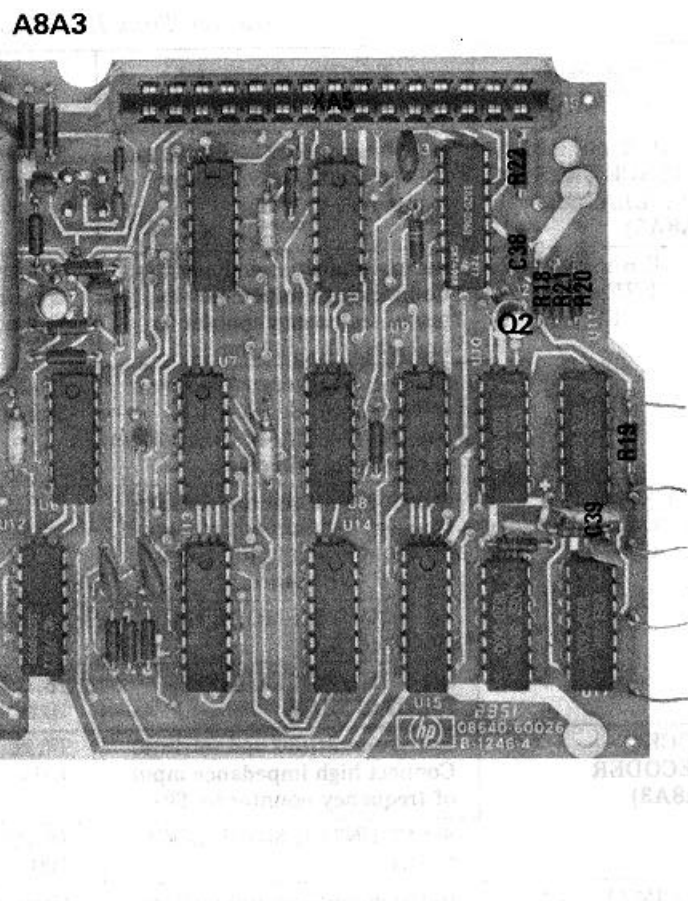
Figure 8-56. P/O A8A3 Time Base Assembly Component Locations
