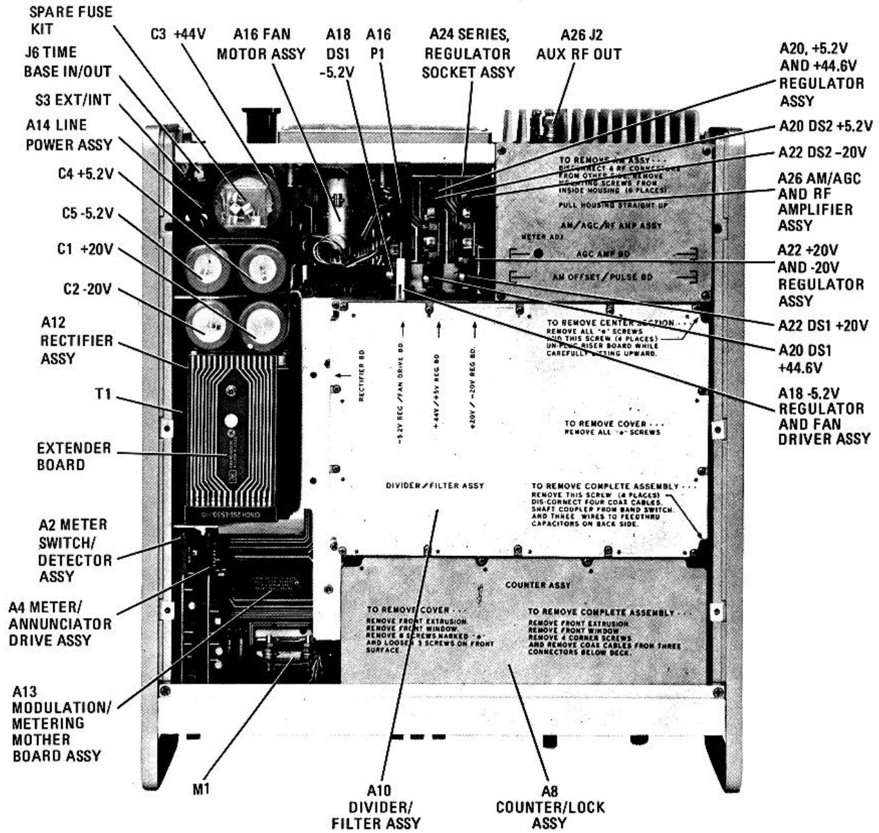
Figure 8-82. Top Internal Views (Options 001 Shown)
