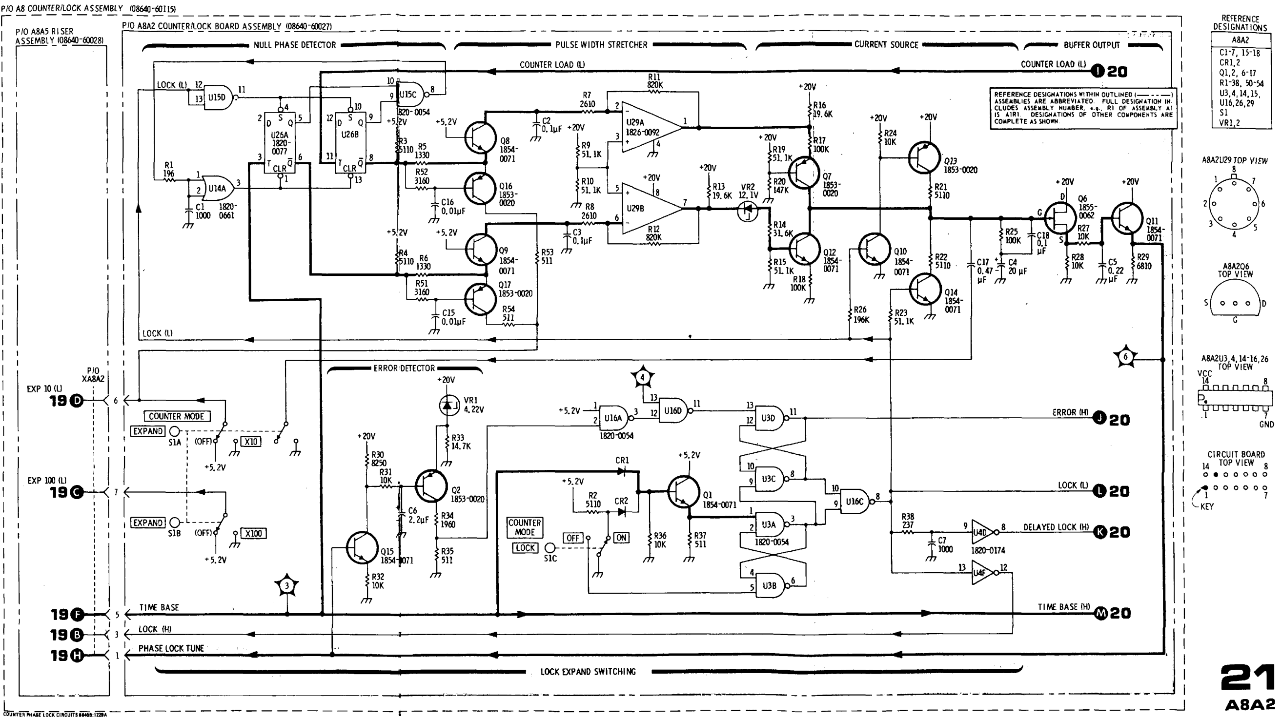
Figure 8-64. Counter Phase Lock Circuits Schematic Diagram
