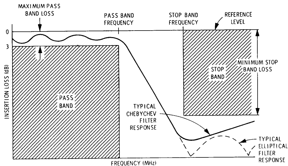
Figure 5-4. Filter Terminology
