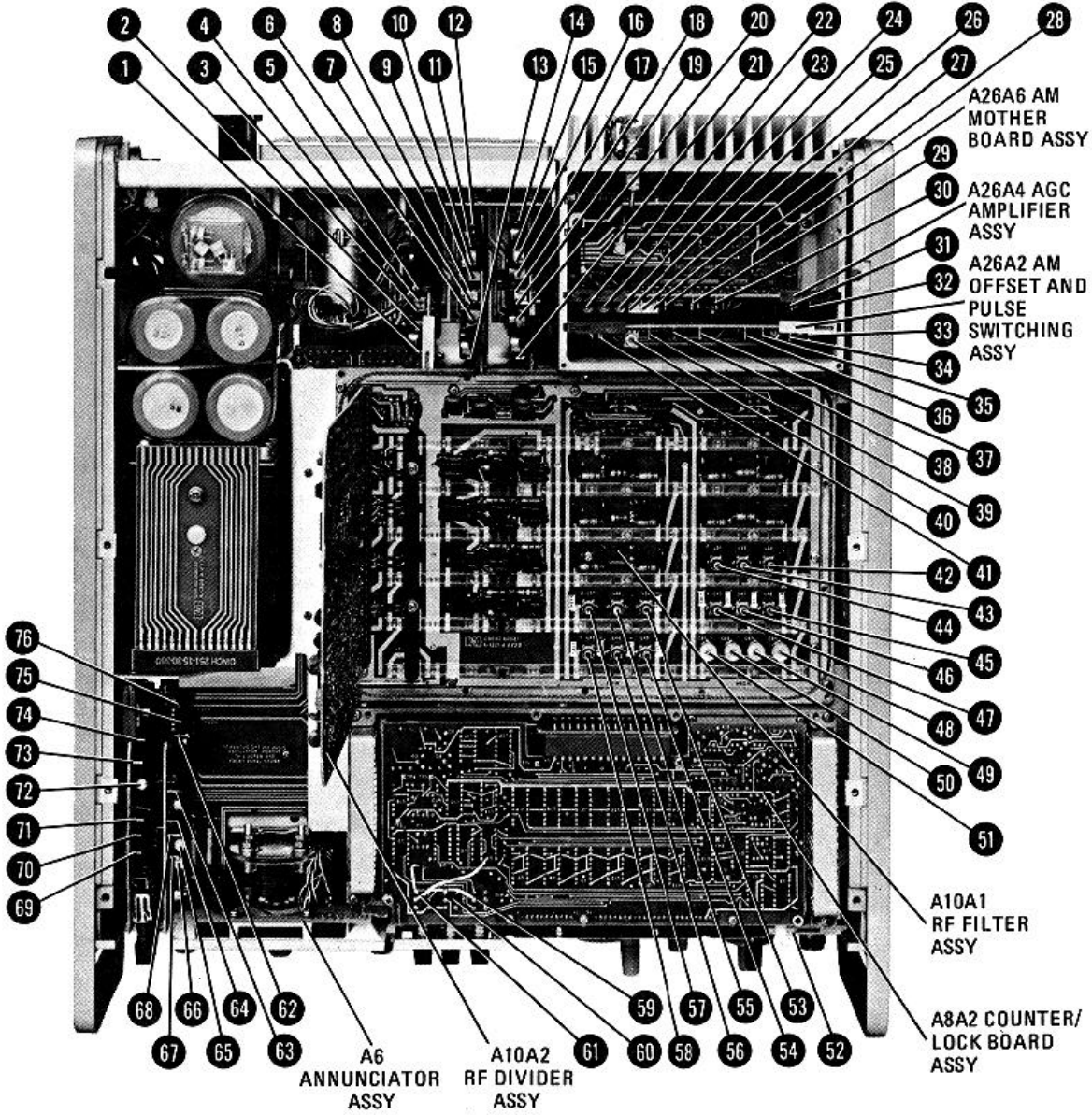
Figure 8-82. Top Internal Views (Options 001 Shown)
