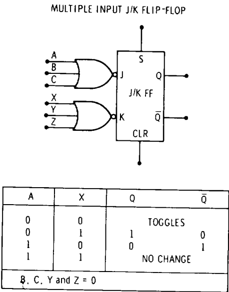
Figure 8-8. Multiple Input J/K Flip-Flop
