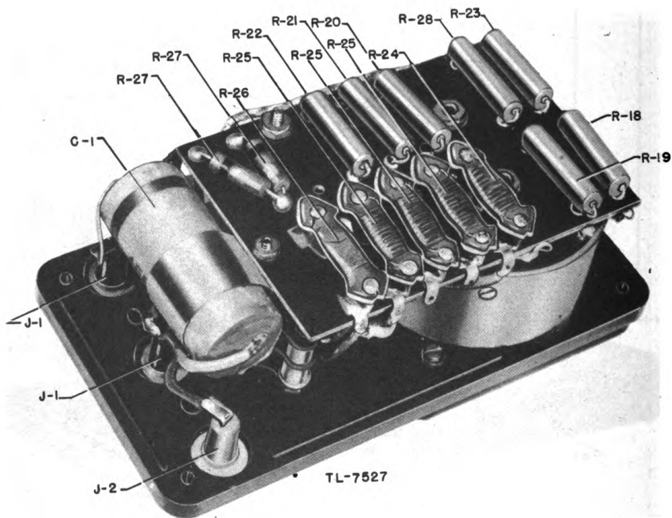
FIG. 36. MODEL 650-SC(J) OUTPUT METER, RESISTOR BOARD
