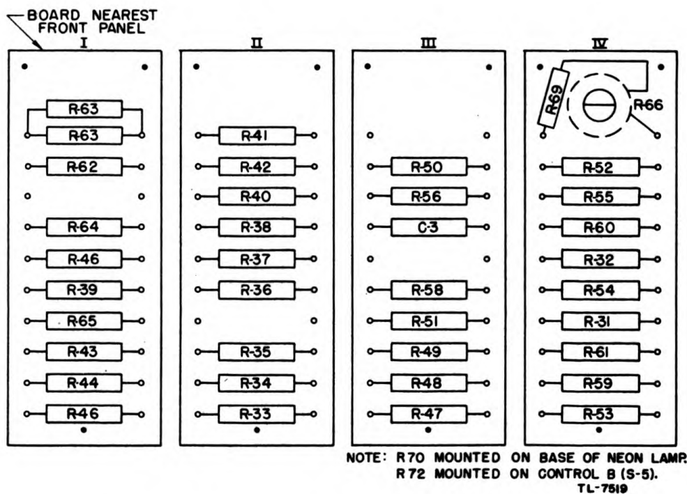
FIG. 24. MODEL 104 COMBINATION TESTER, RESISTOR BOARD DIAGRAM
