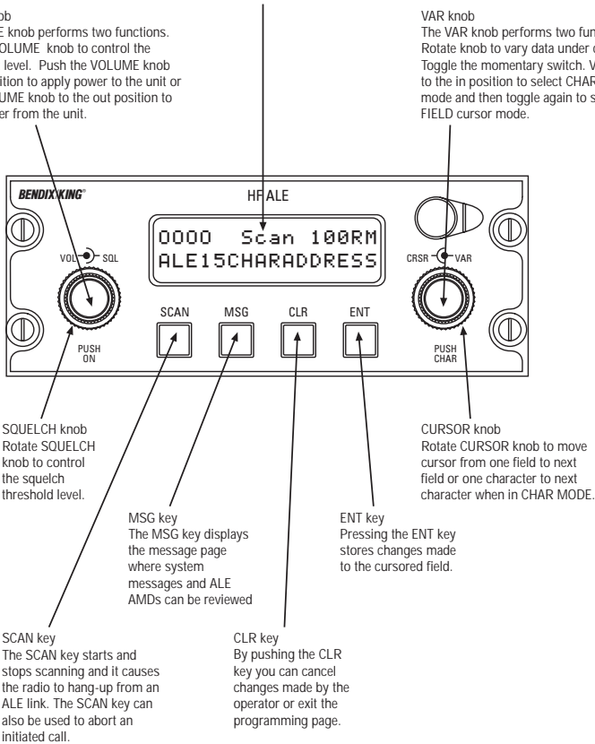
Figure 2-1 KCU 1051 Control Display Unit
