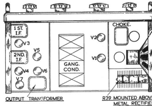
PLAN VIEW OF "670" RX. IN OUTLINE.
