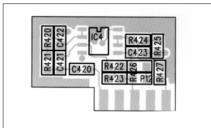
406-968-C (RF. PCB) TOP
