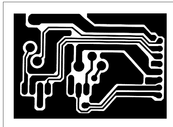
VOLUME BOARD BOTTOM VIEW
