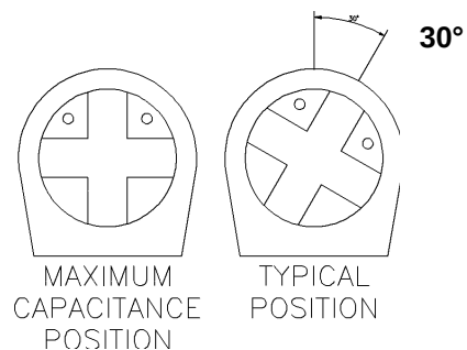
TC7 Maximum Capacitance Position
