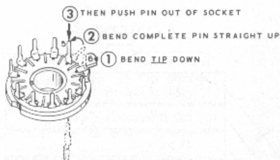
Detail 1-1B
