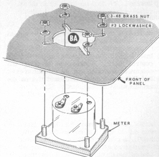
Detail 6-1B
