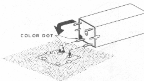
Detail 1-10D
